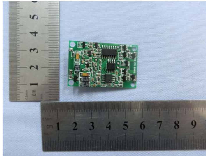
EUT – Front View (receiver DL-CS2017B)
