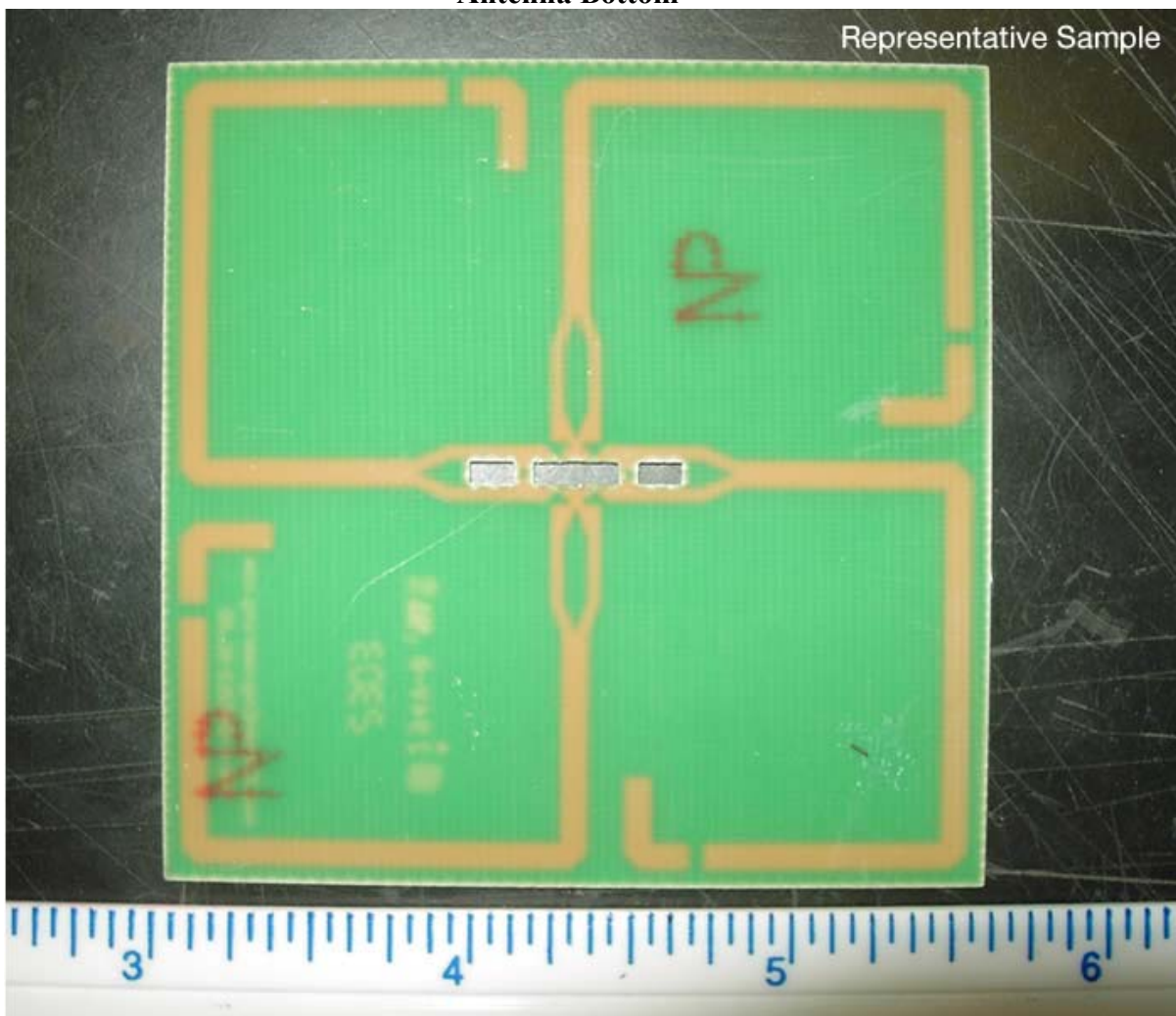
Antenna Bottom
