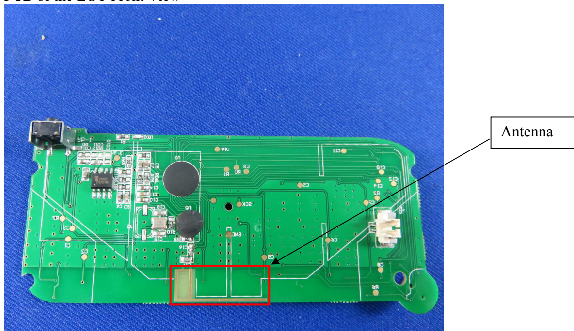
Figure 14 PCB of the EUT-Front View
