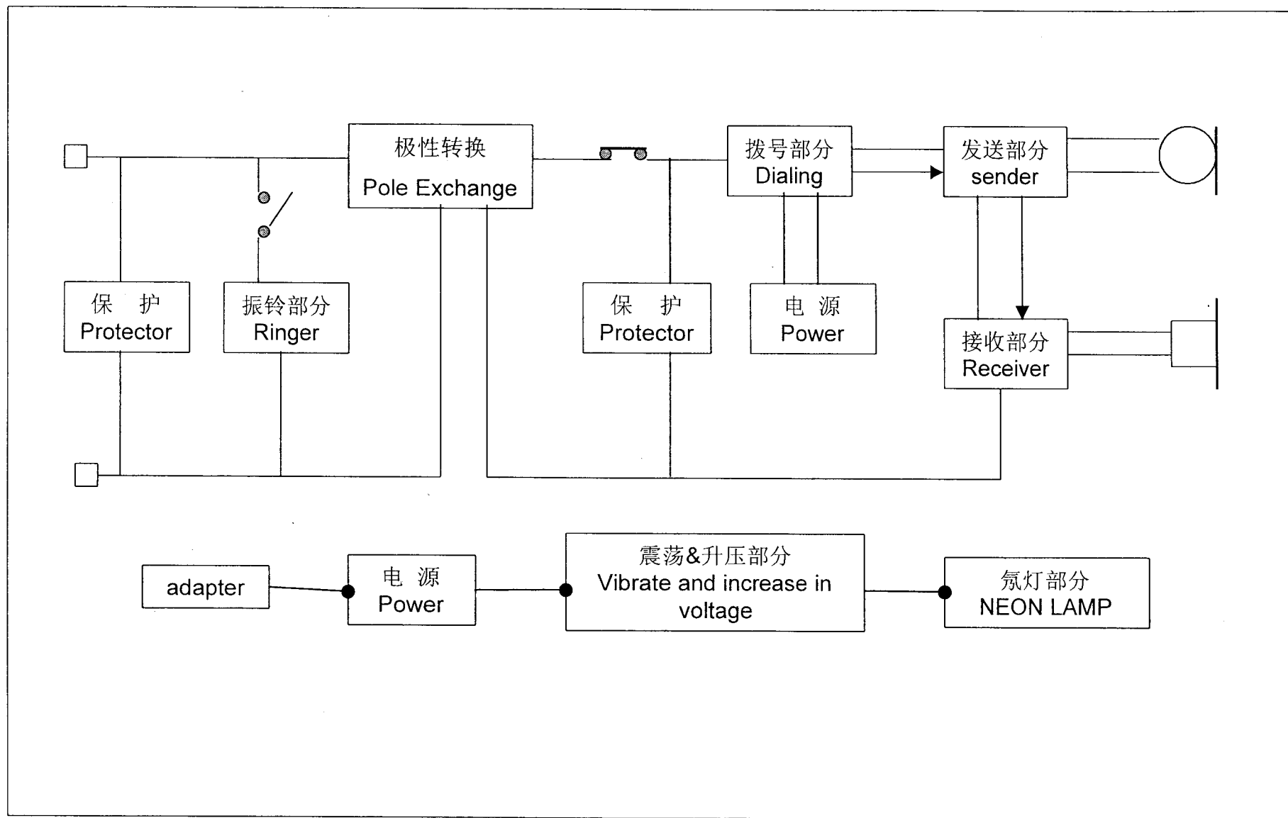
17J1622/WF-822 机方框图：BLOCK DIAGRAM
