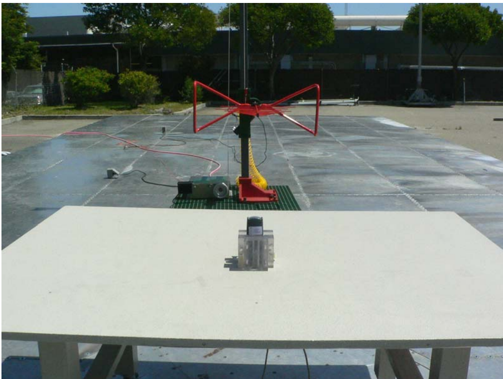
Handset Radiated Emission – Rear View
