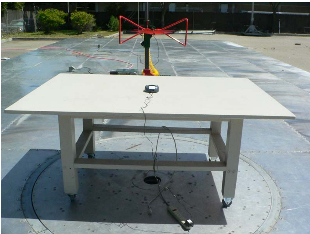
Base Radiated Emission – Rear View
