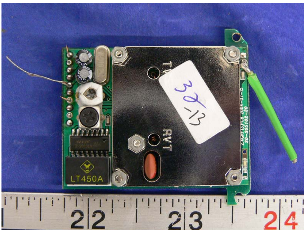
TX Board Component View
