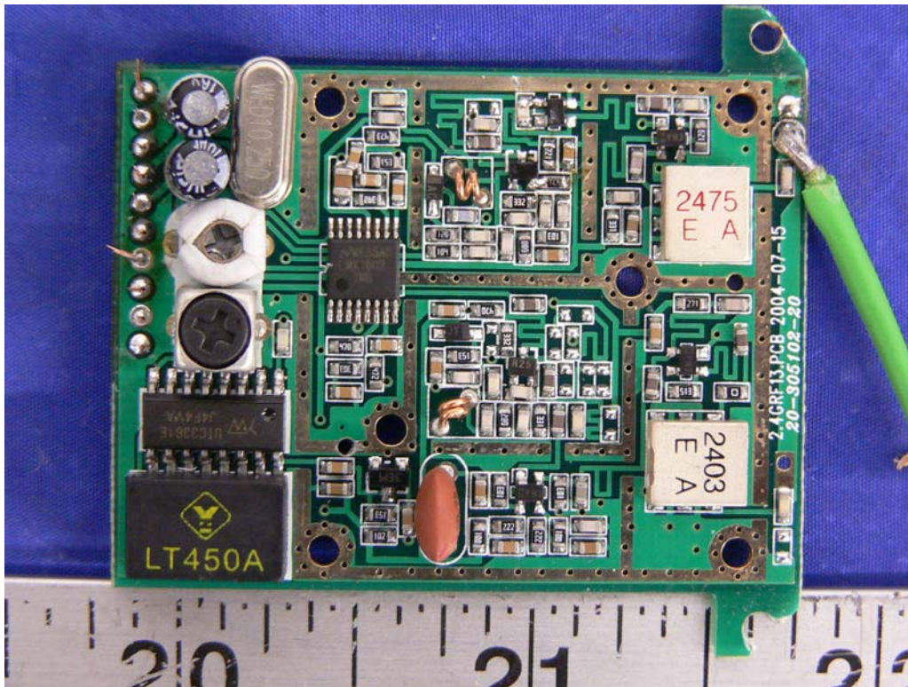
TX Board Cover Off View
