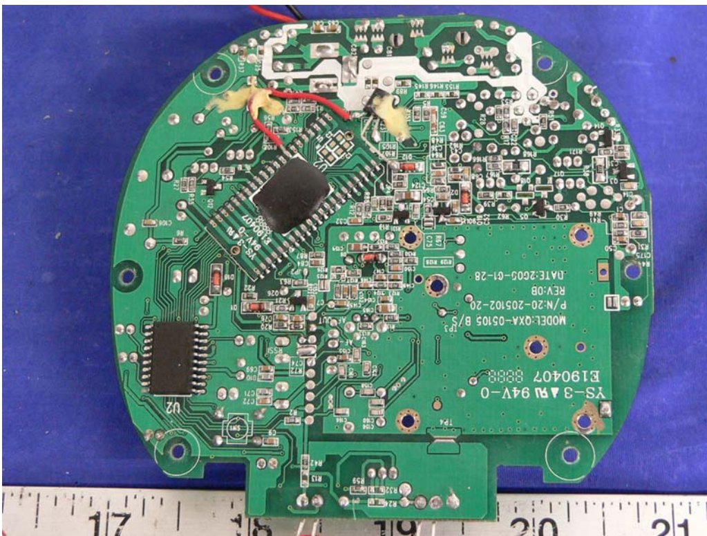
Base EUT – Board Solder View
