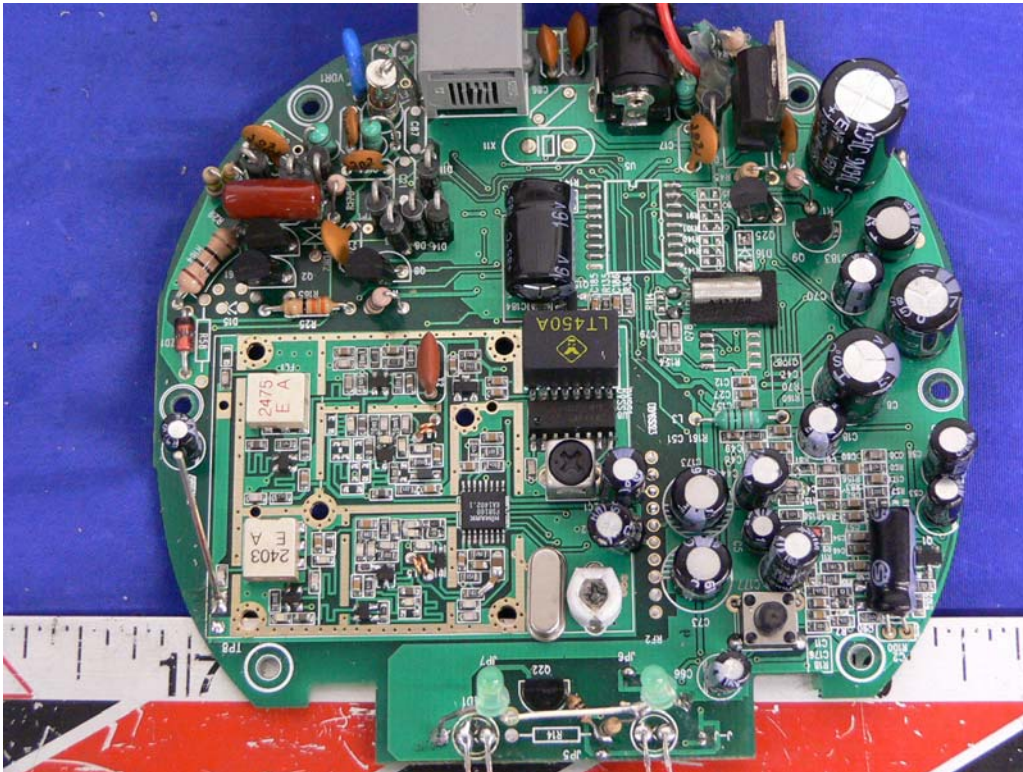
Base EUT – Board Component View
