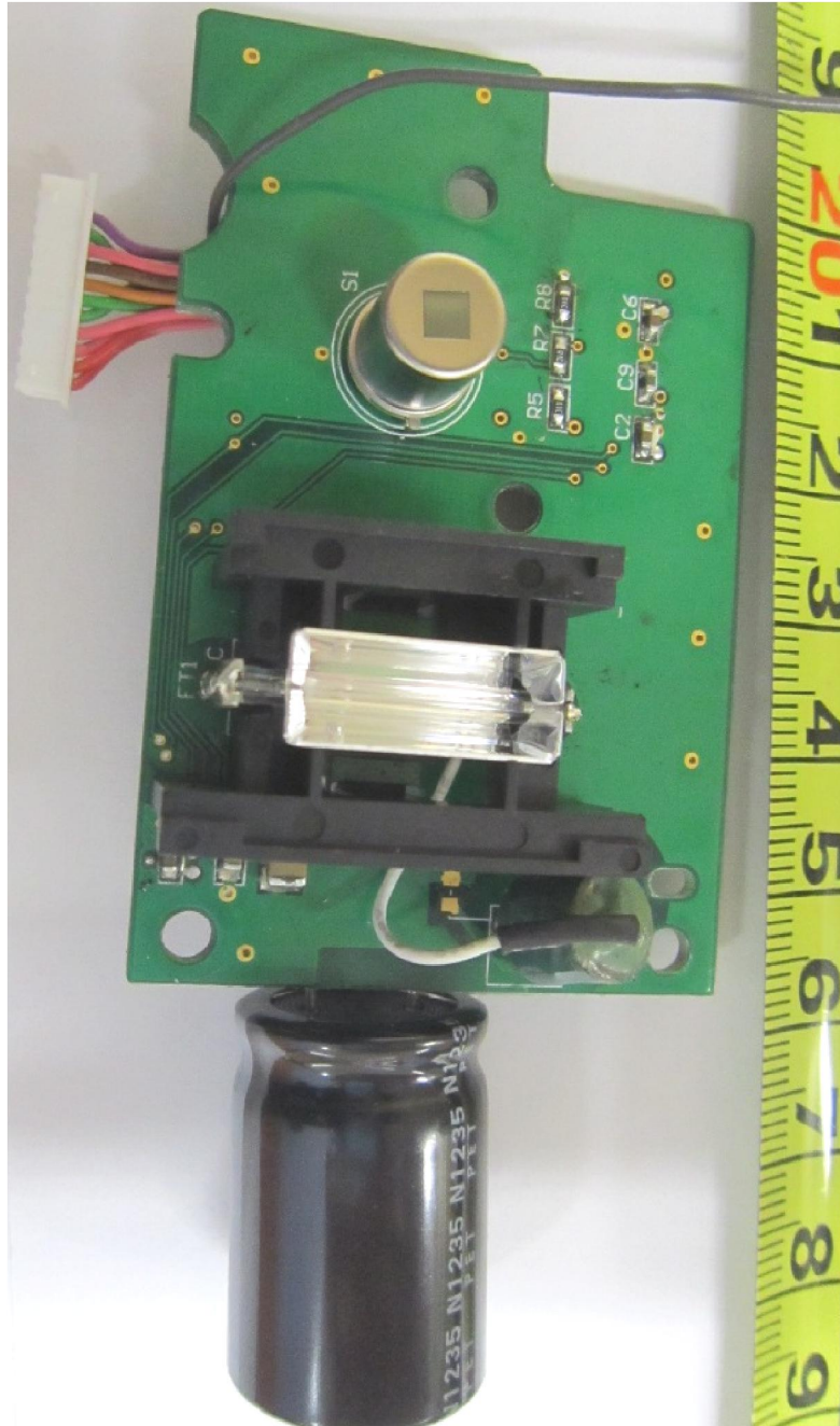
Flash Board PCB Trace Side
