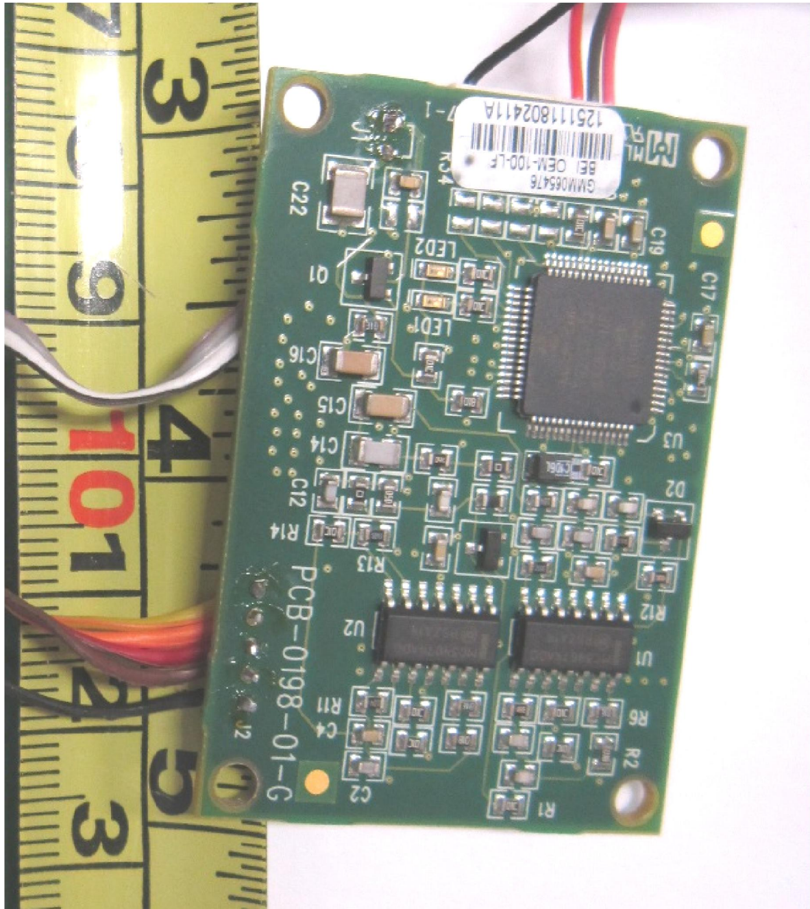
RF Module Circuit (Bottom View)
