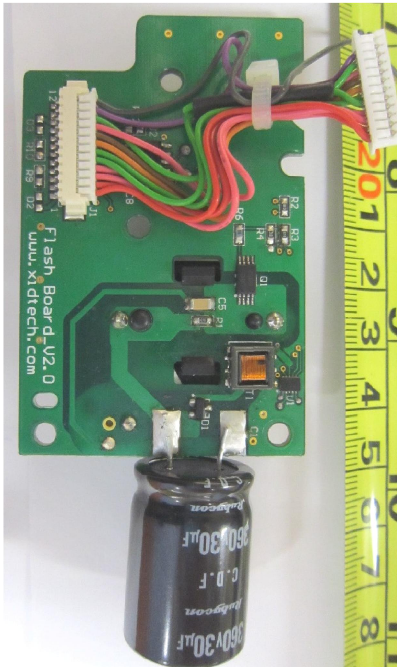
Flash Board PCB Component Side
