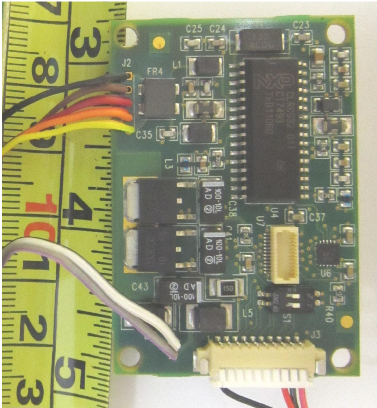
RF Module Circuit (Top View)
