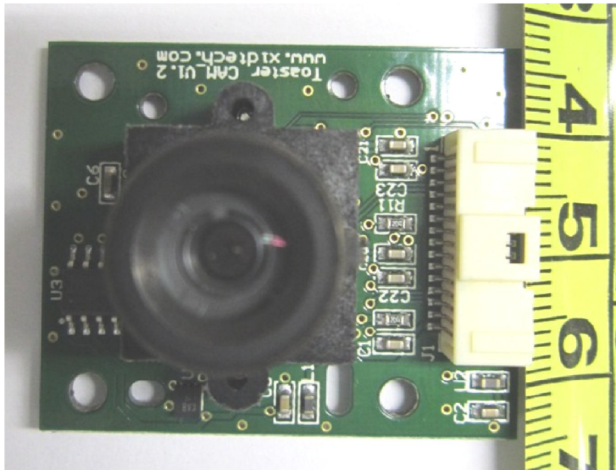
Camera Board PCB Component Side
