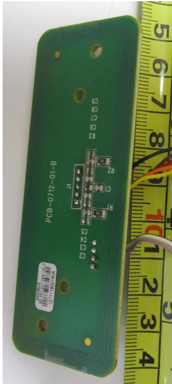
Antenna Board PCB Trace Side
