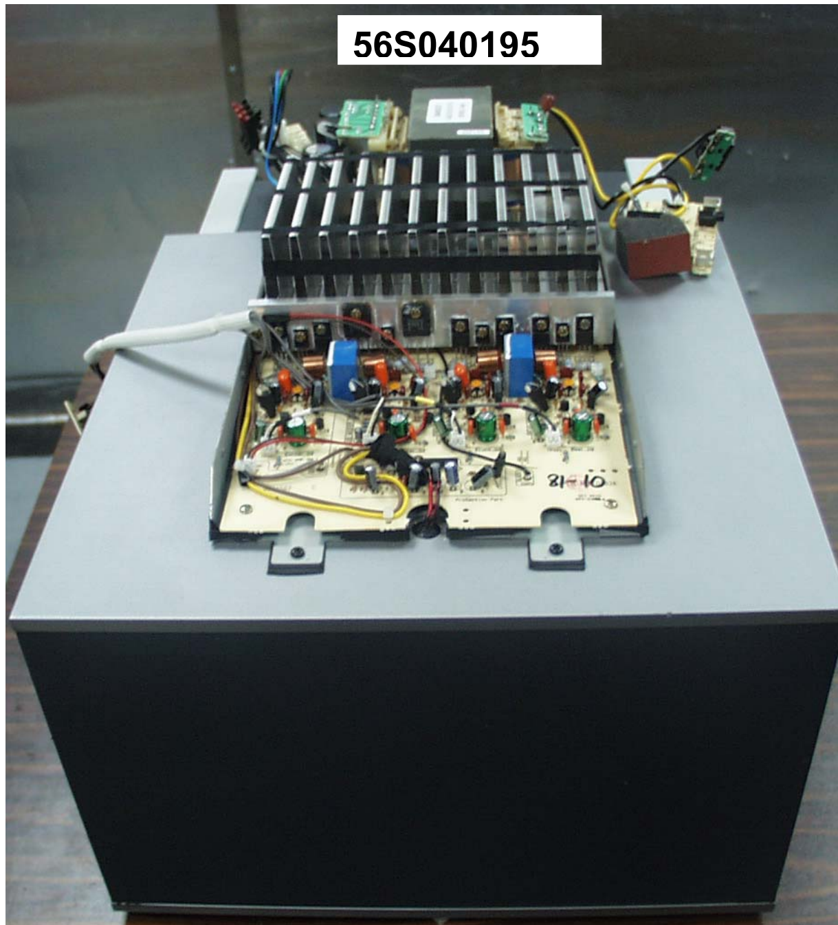
Subwoofer – Internal Layout
