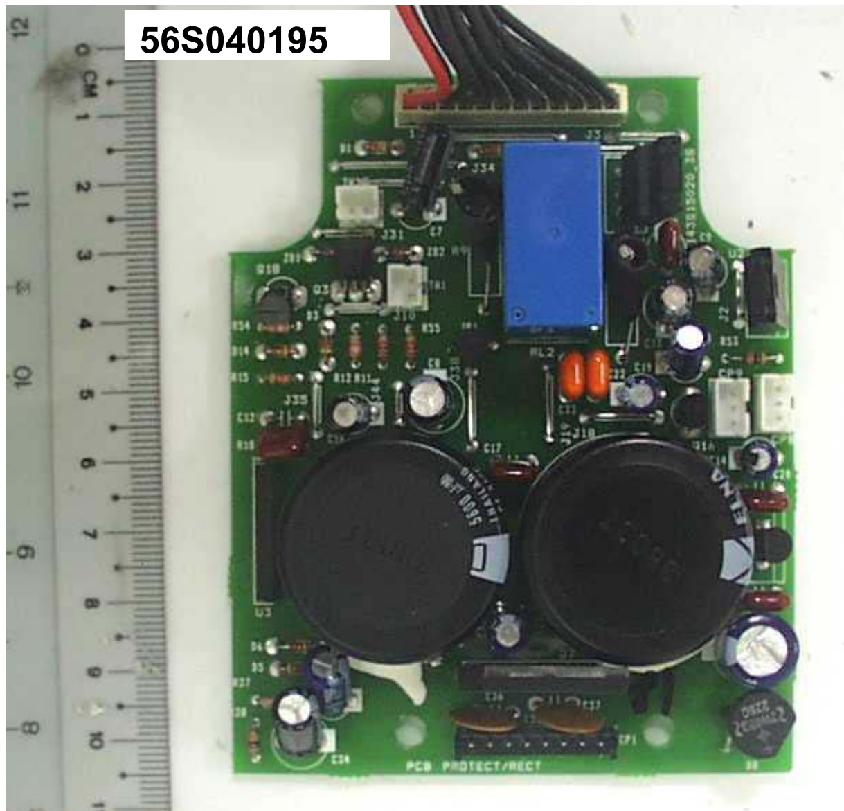
Rear Left/Right Speaker – Rectifier Board Component Side
