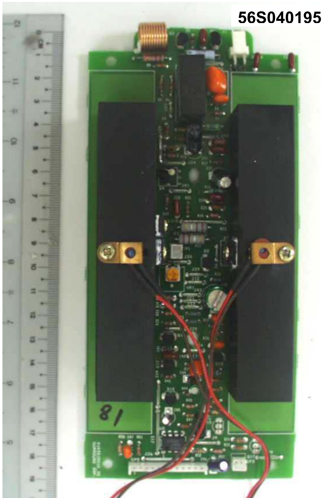
Rear Left/Right Speaker – Amplifier Board Component Side
