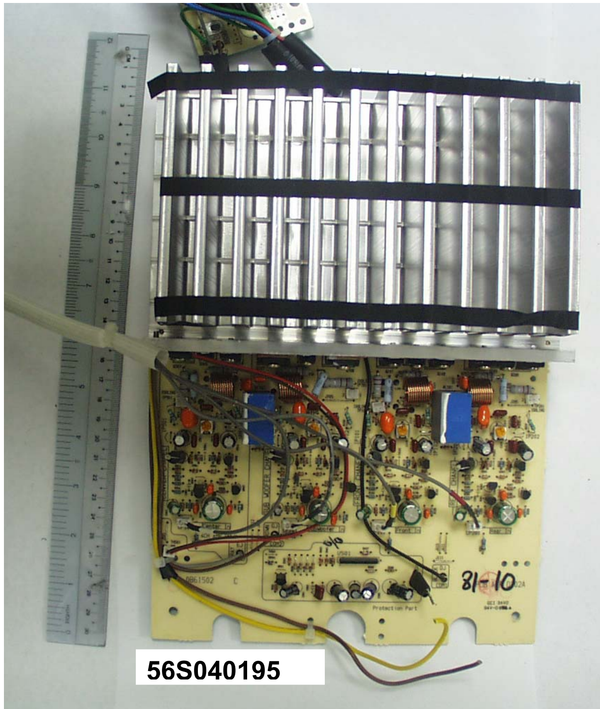
Subwoofer – Amplifier Board Component Side
