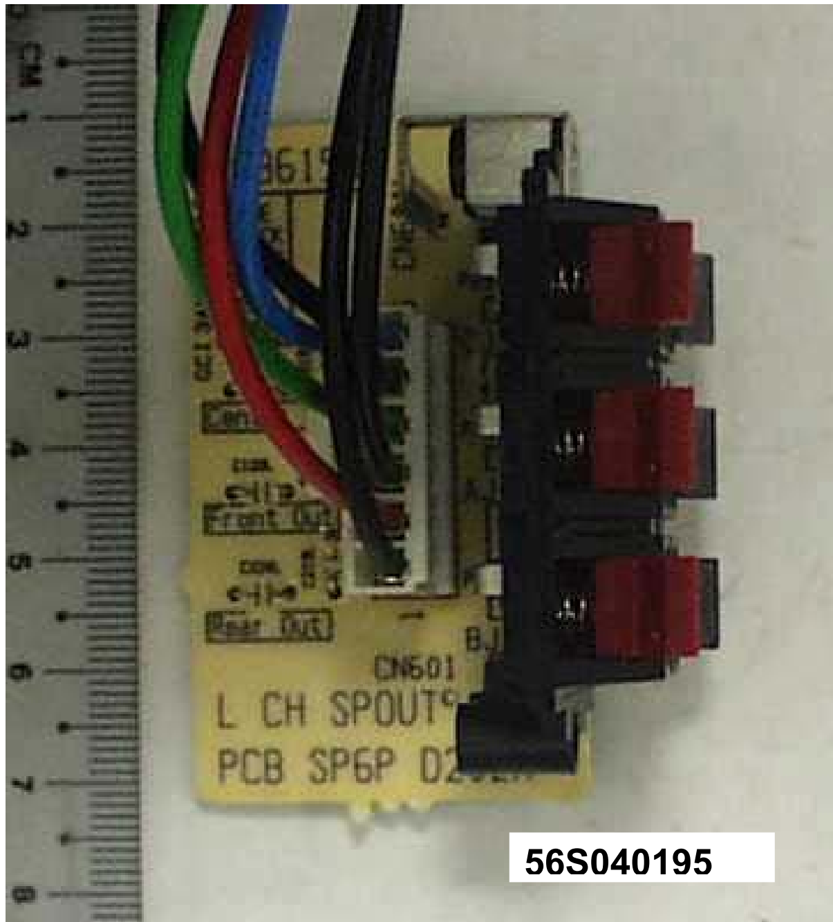
Subwoofer – Power Supply Sub-Board Component Side
