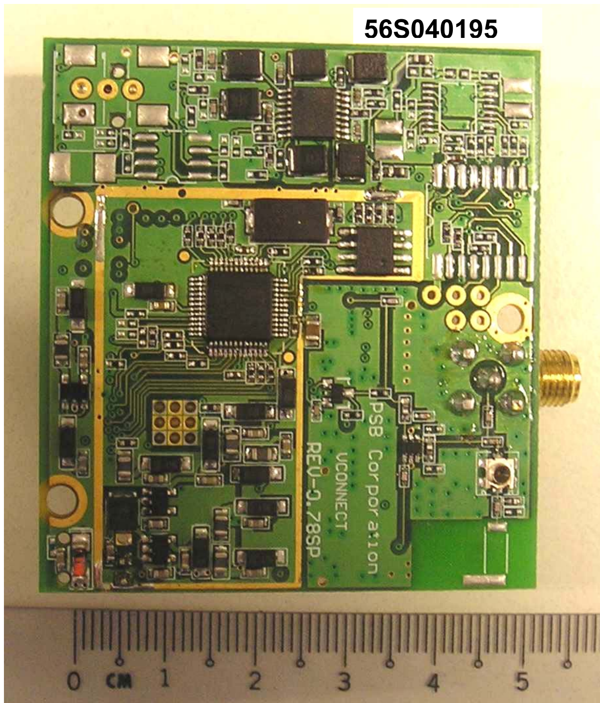
AV Unit – RF Board Component Side (With RF Shield Removed)
