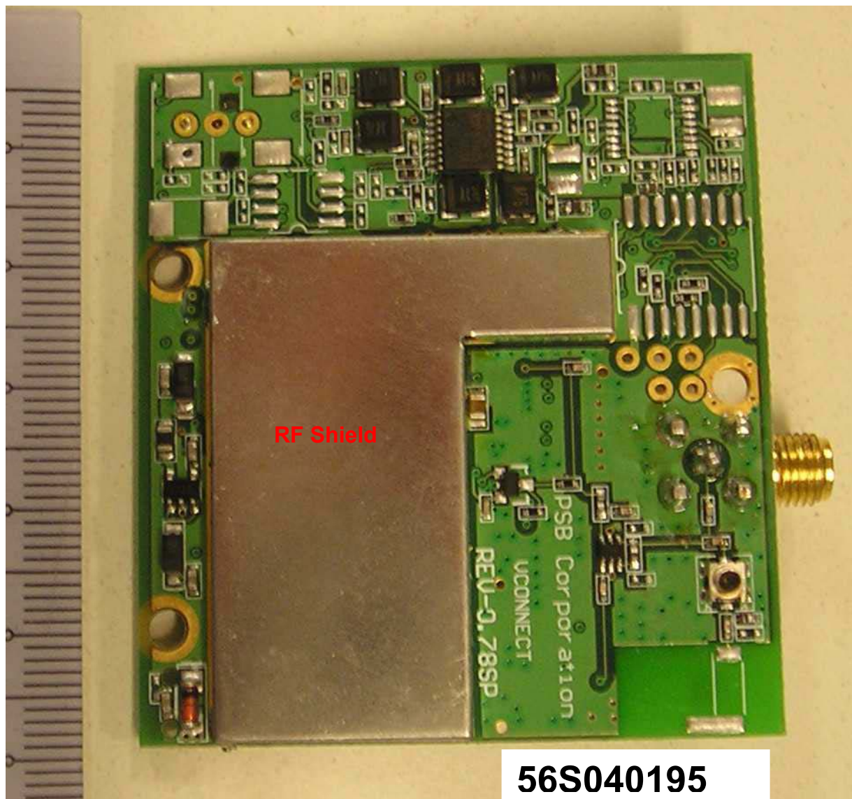
AV Unit – RF Board Component Side (With RF Shield)
