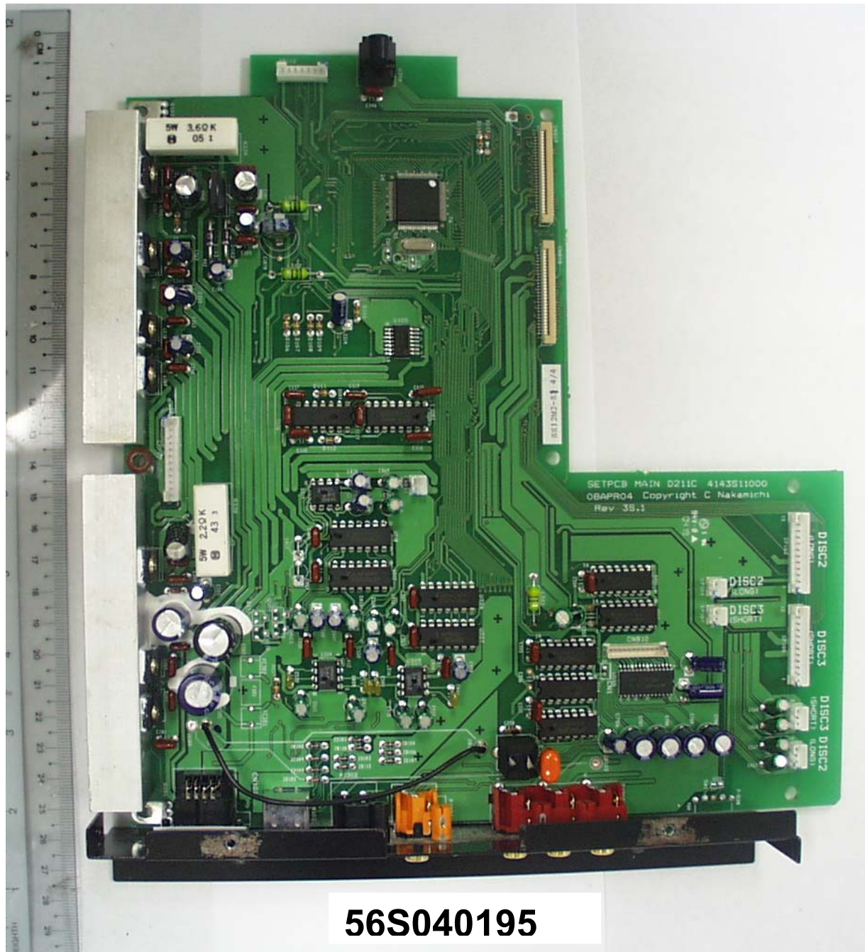
Main Unit – MainBoard Component Side
