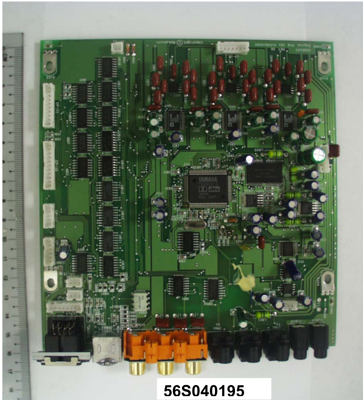
Main Unit – Digital Board Component Side
