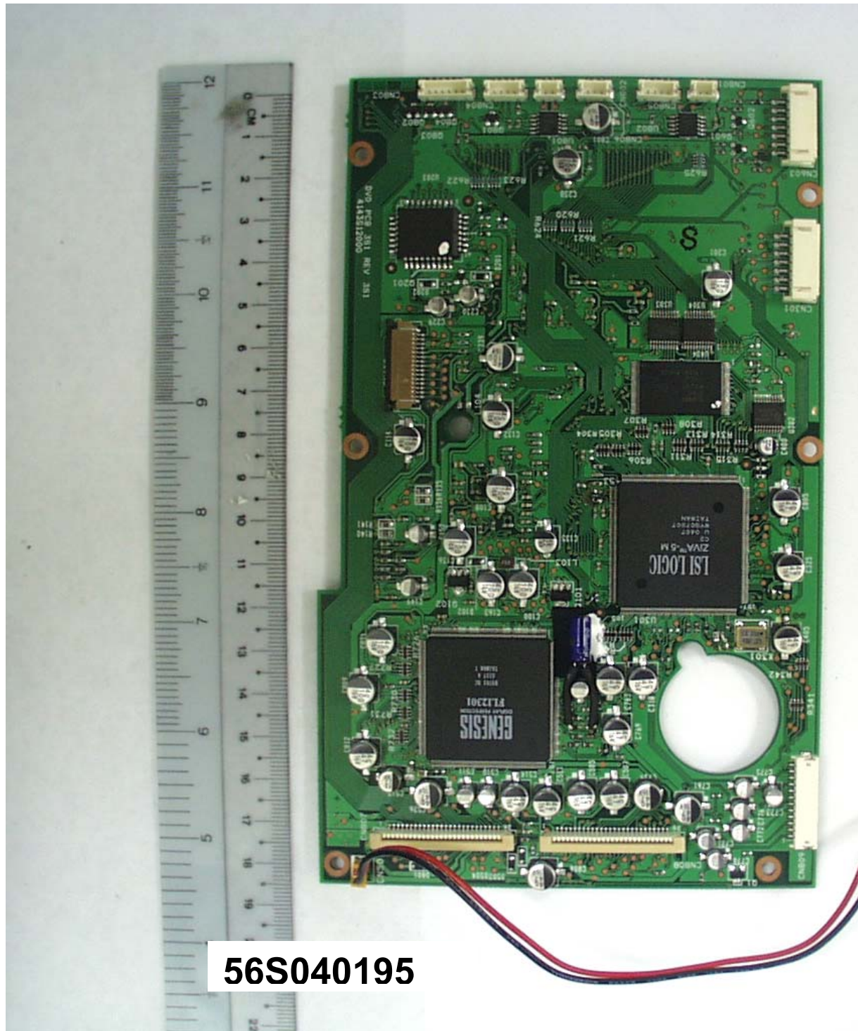
Main Unit – DVD Board Component Side
