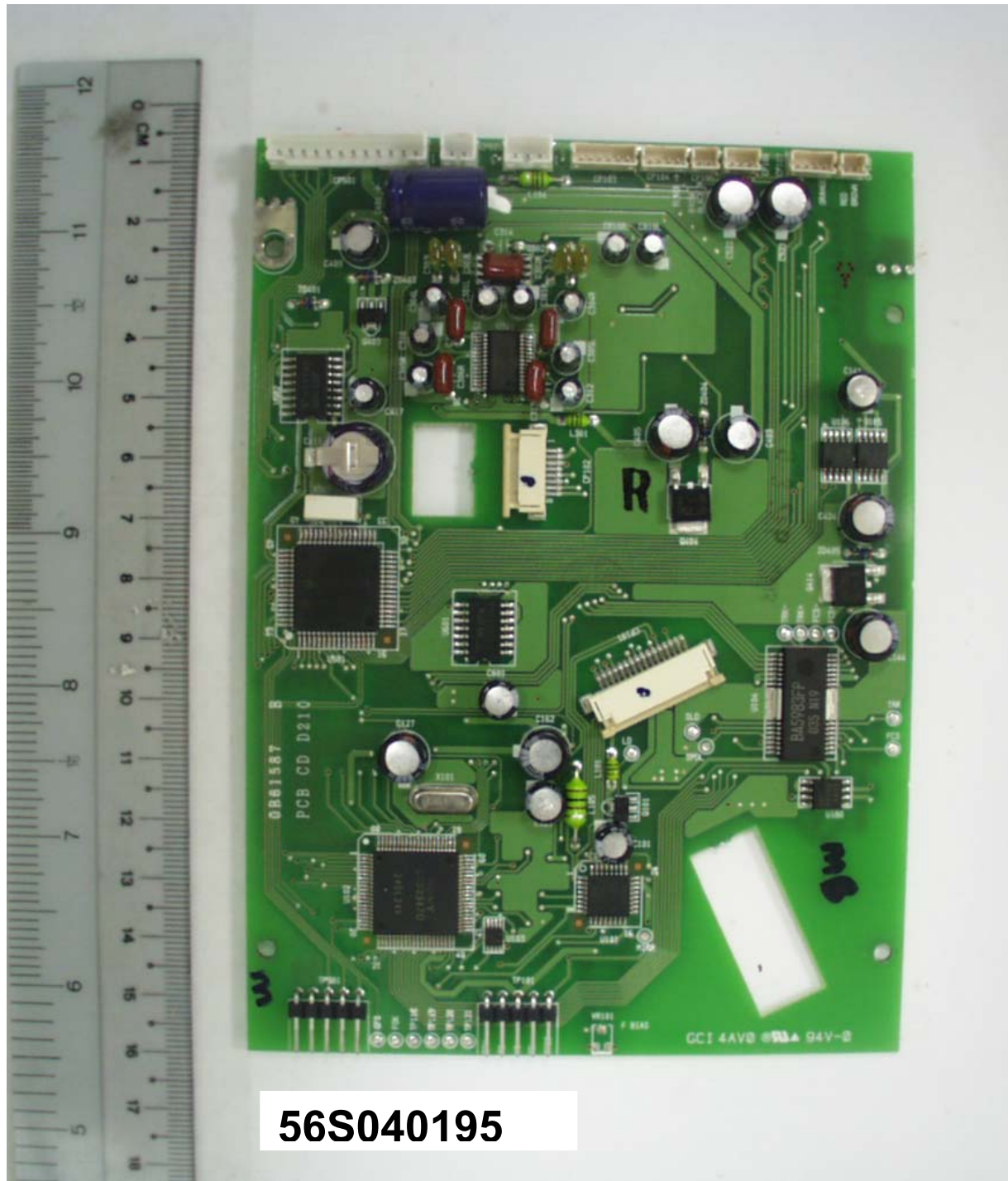
Main Unit – CD Board Component Side
