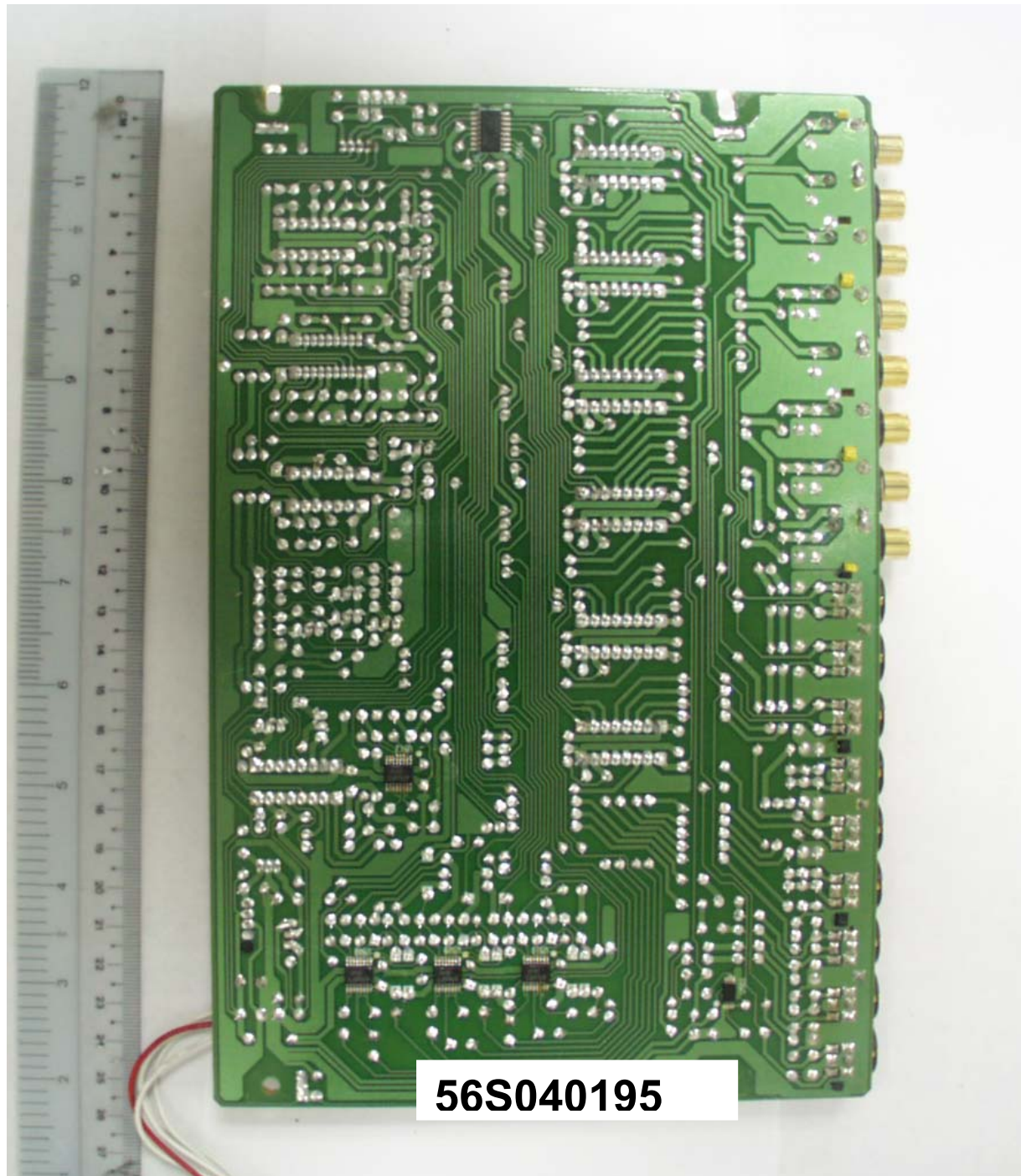
Main Unit – Video Board Trace Side
