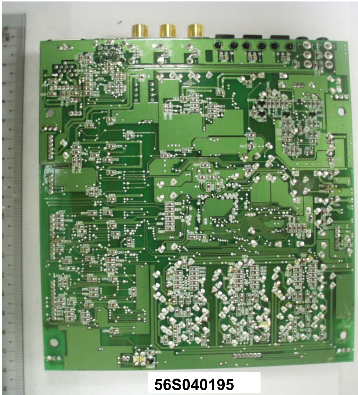
Main Unit – Digital Board Trace Side
