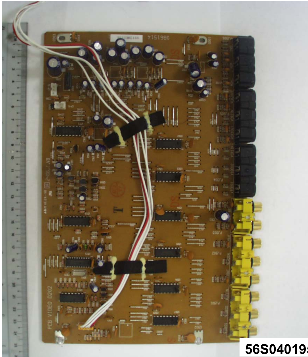
Main Unit – Video Board Component Side
