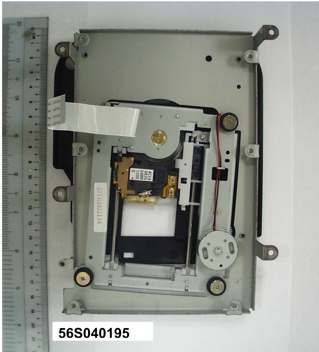
Main Unit – Mega View 2
