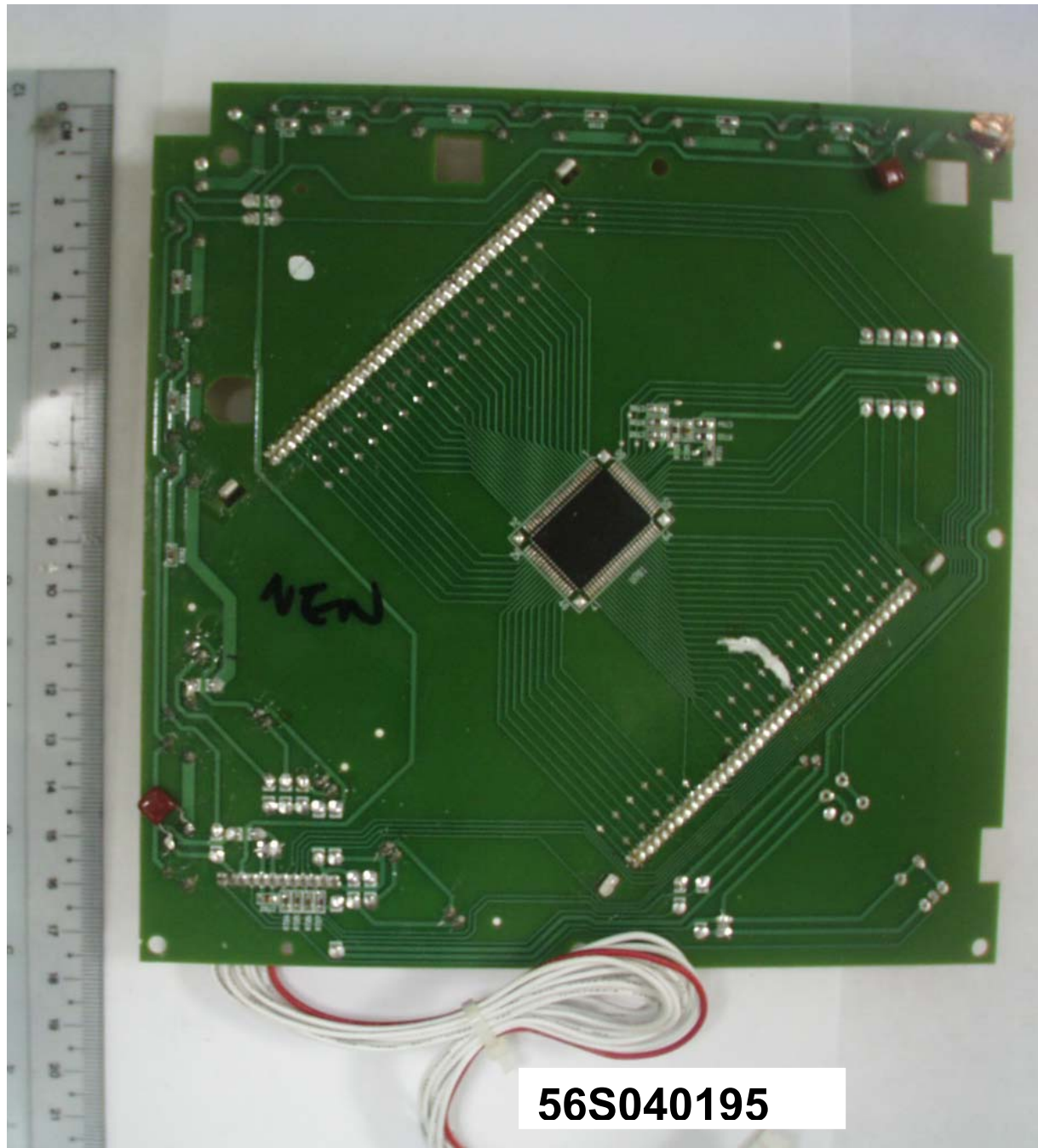
Main Unit – LCD Display Trace Side
