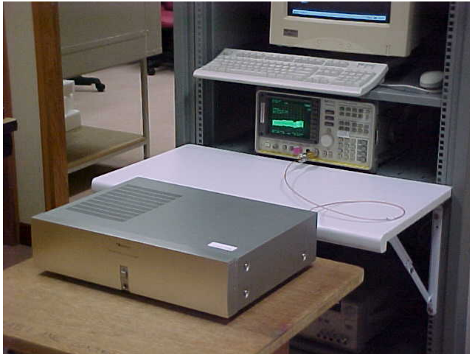
Average Frequency Dwell Time Measurement Test Setup – AV Unit
