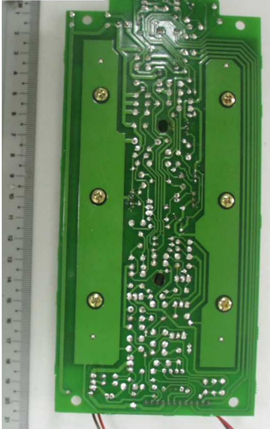
Rear Left/Right Speaker – Amplifier Board Trace Side
