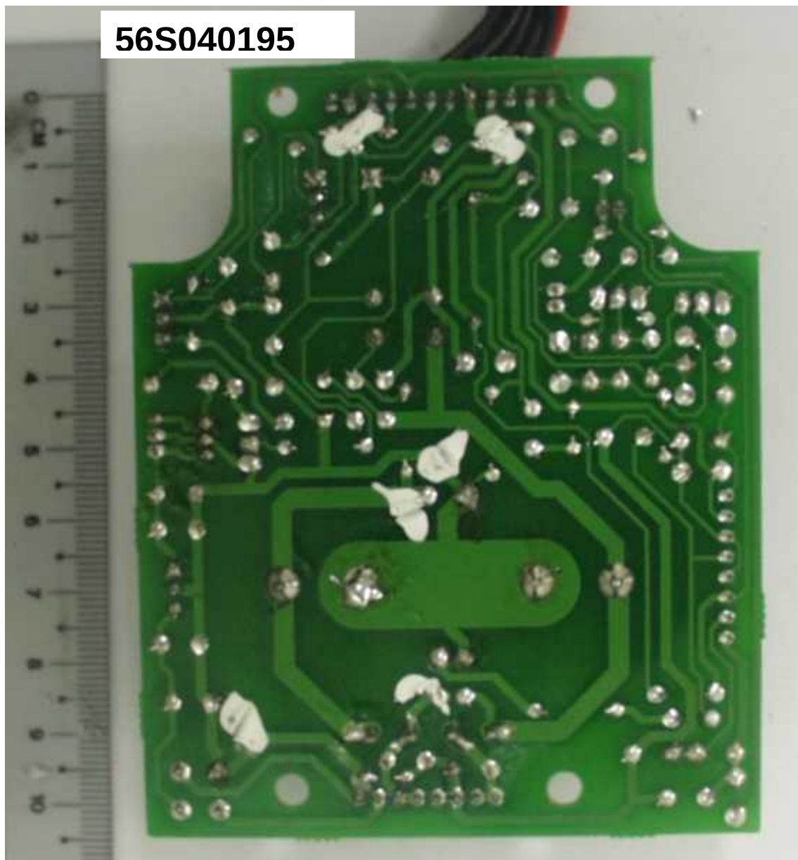
Rear Left/Right Speaker – Rectifier Board Trace Side
