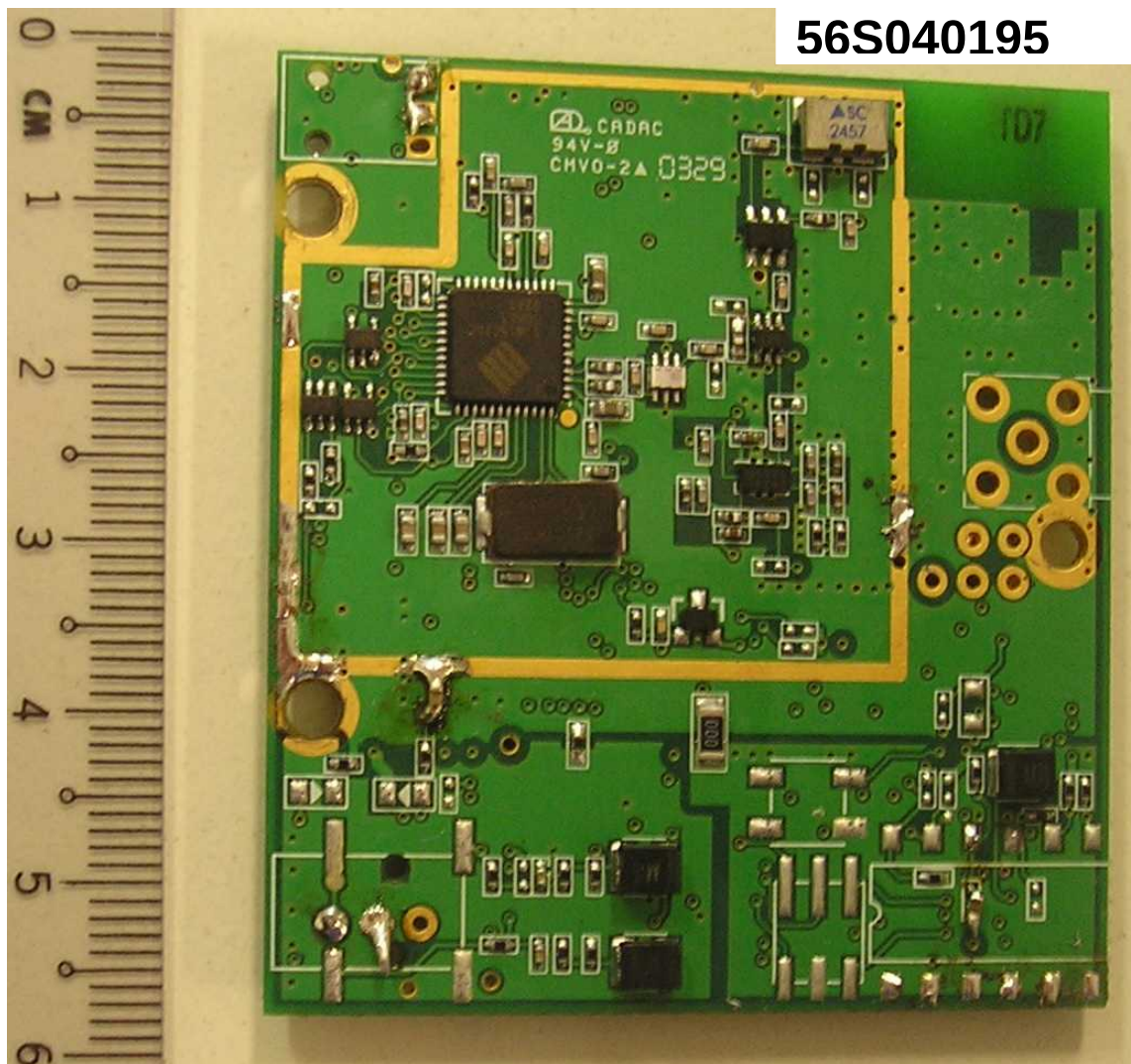
Rear Left/Right Speaker – RF Board Trace Side
