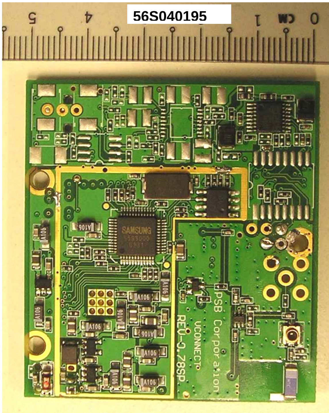
Rear Left/Right Speaker – RF Board Component Side (With RF Shield Removed)
