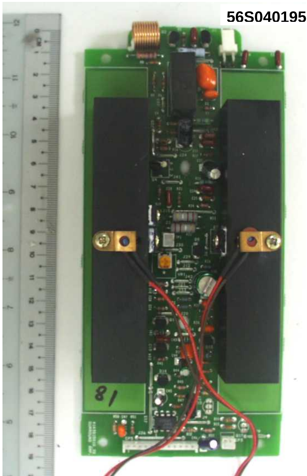
Rear Left/Right Speaker – Amplifier Board Component Side
