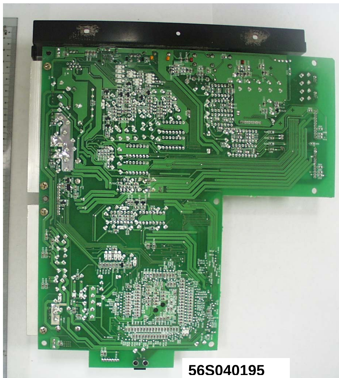
Main Unit – MainBoard Trace Side
