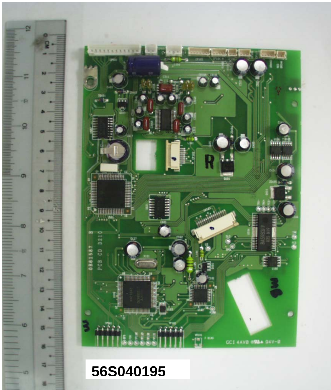
Main Unit – CD Board Component Side
