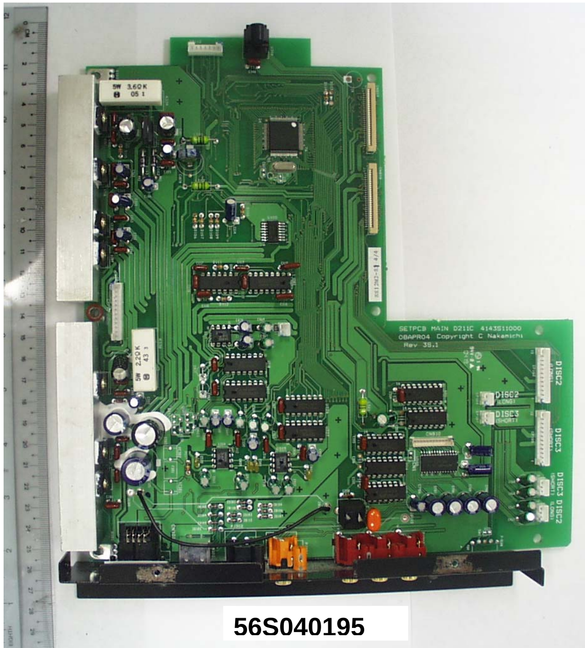
Main Unit – MainBoard Component Side
