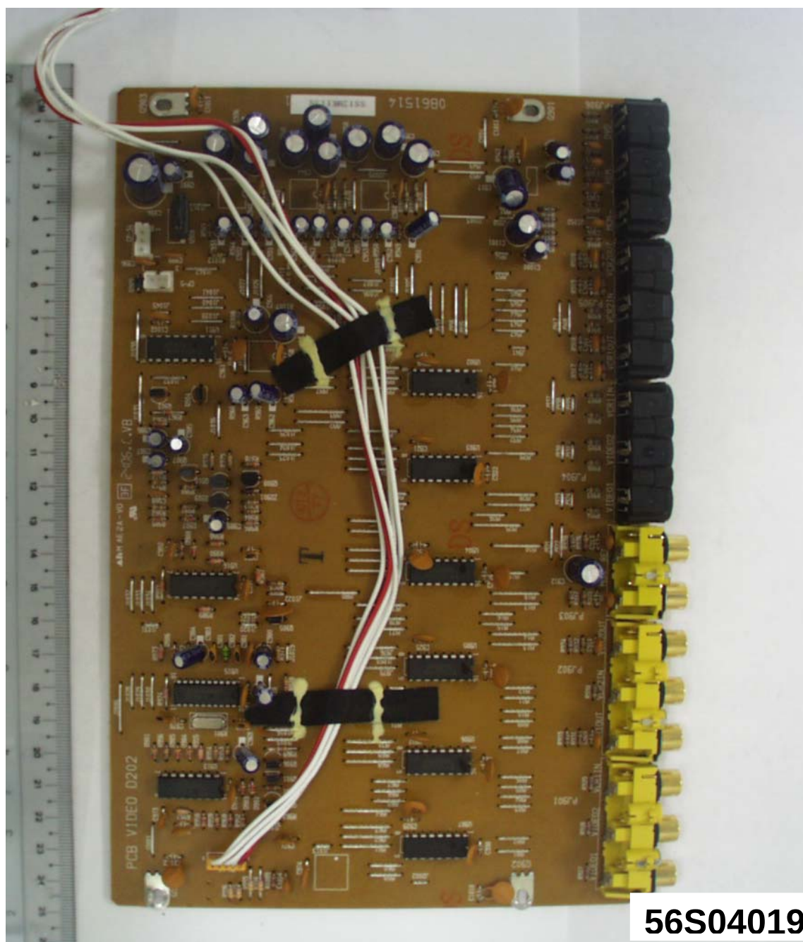
Main Unit – Video Board Component Side
