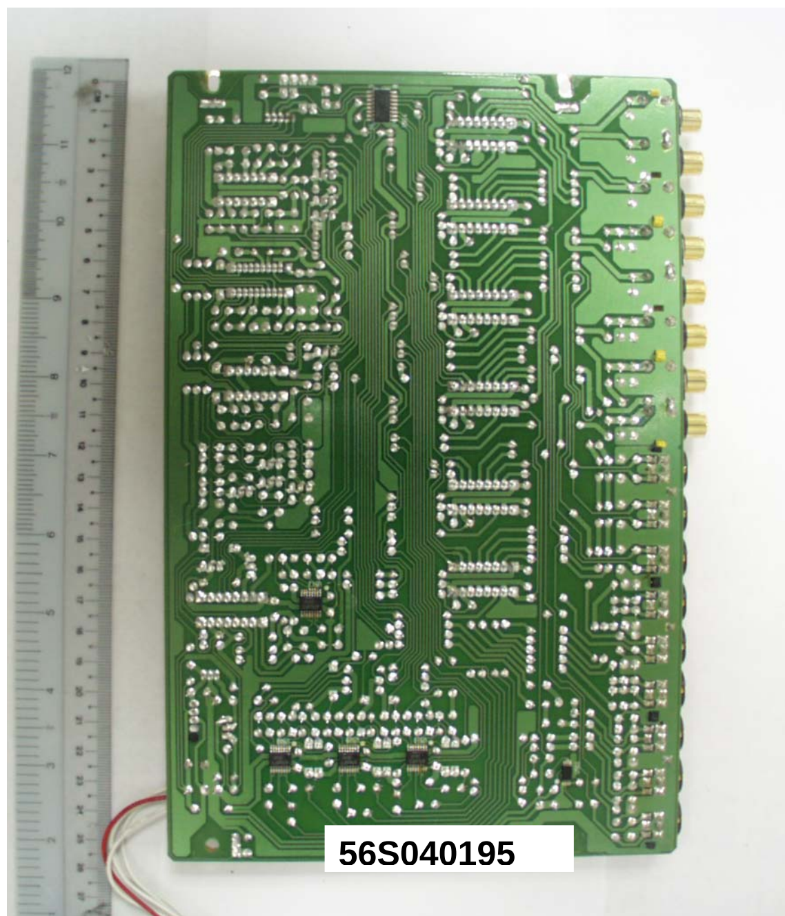
Main Unit – Video Board Trace Side
