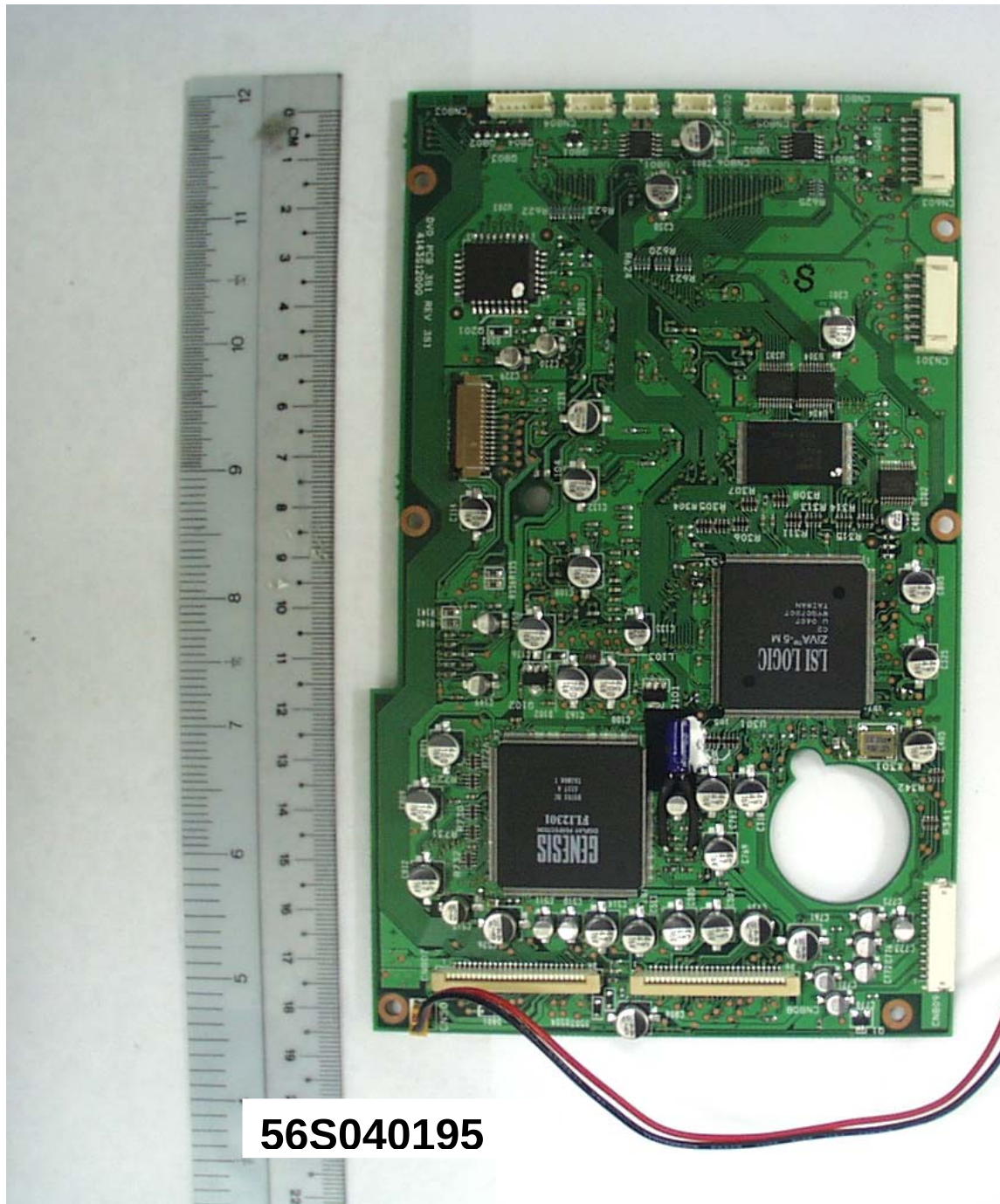
Main Unit – DVD Board Component Side
