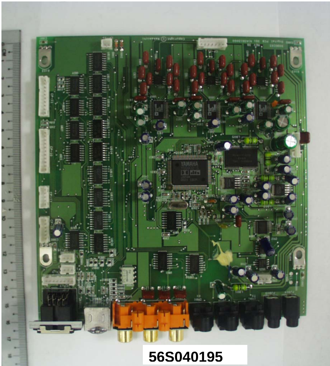
Main Unit – Digital Board Component Side
