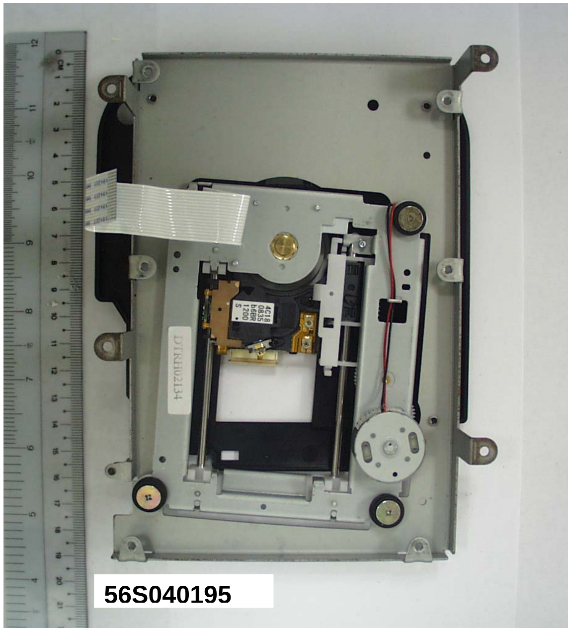
Main Unit – Mega View 2
