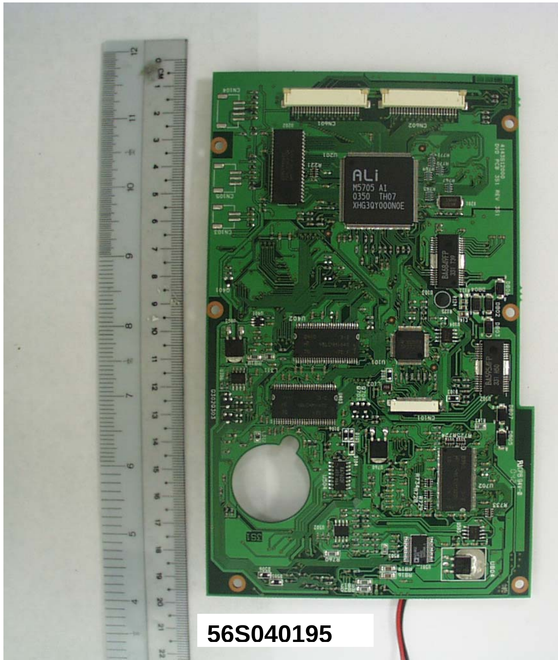
Main Unit – DVD Board Trace Side
