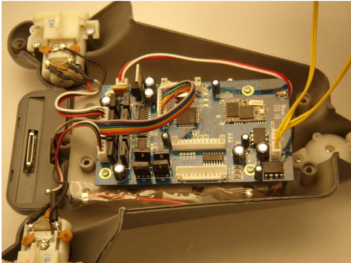
Main board
