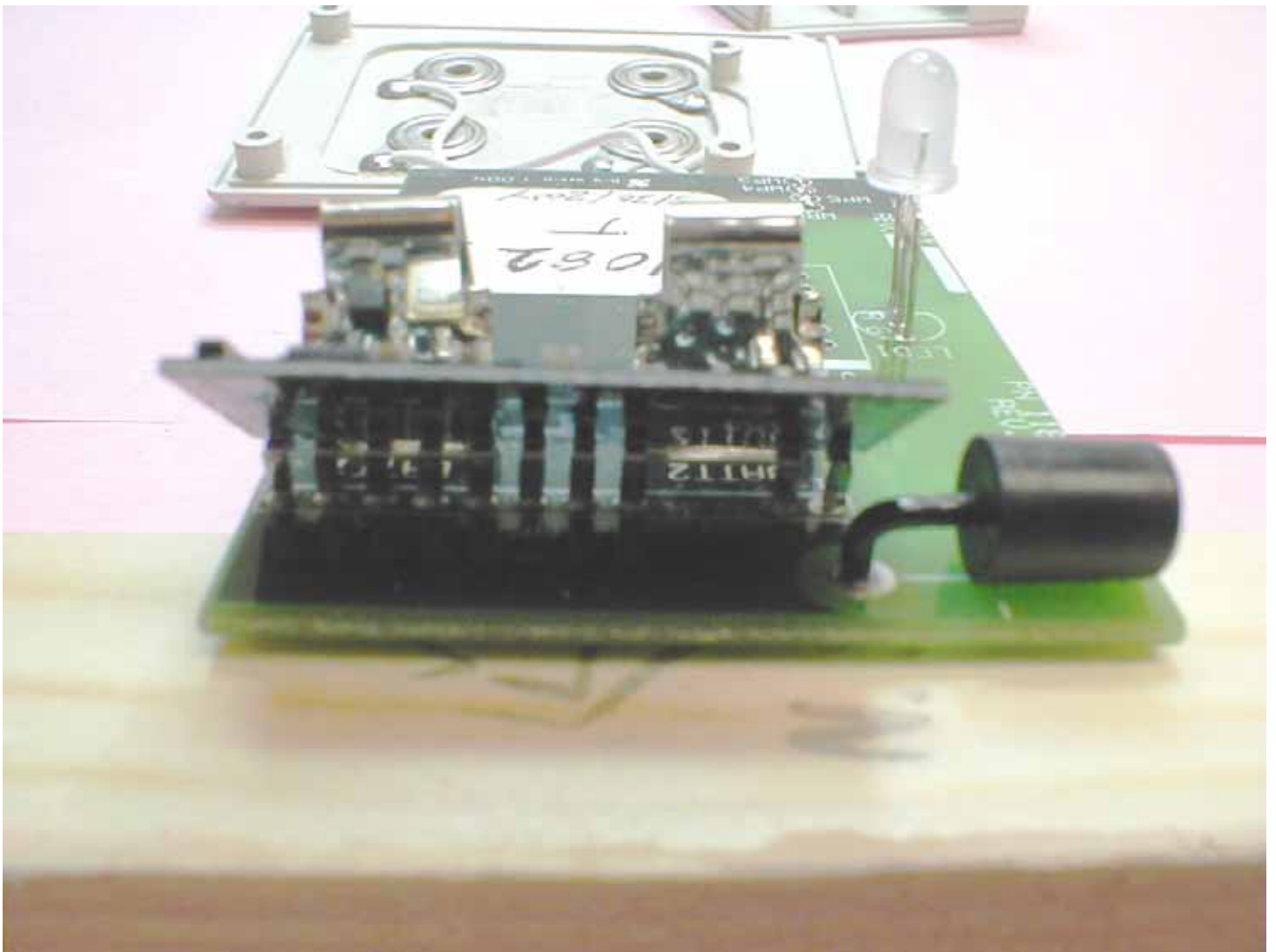
Underside of Transmit Board
