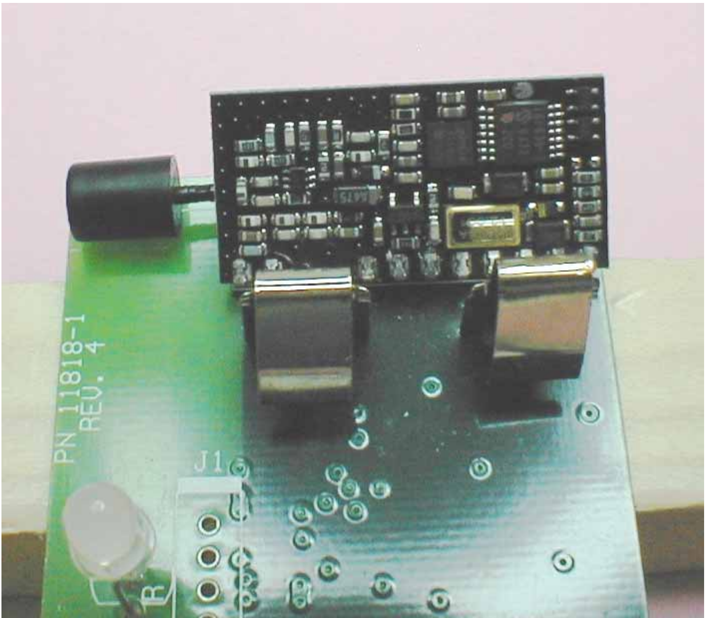
Detail View – Transmit Board
