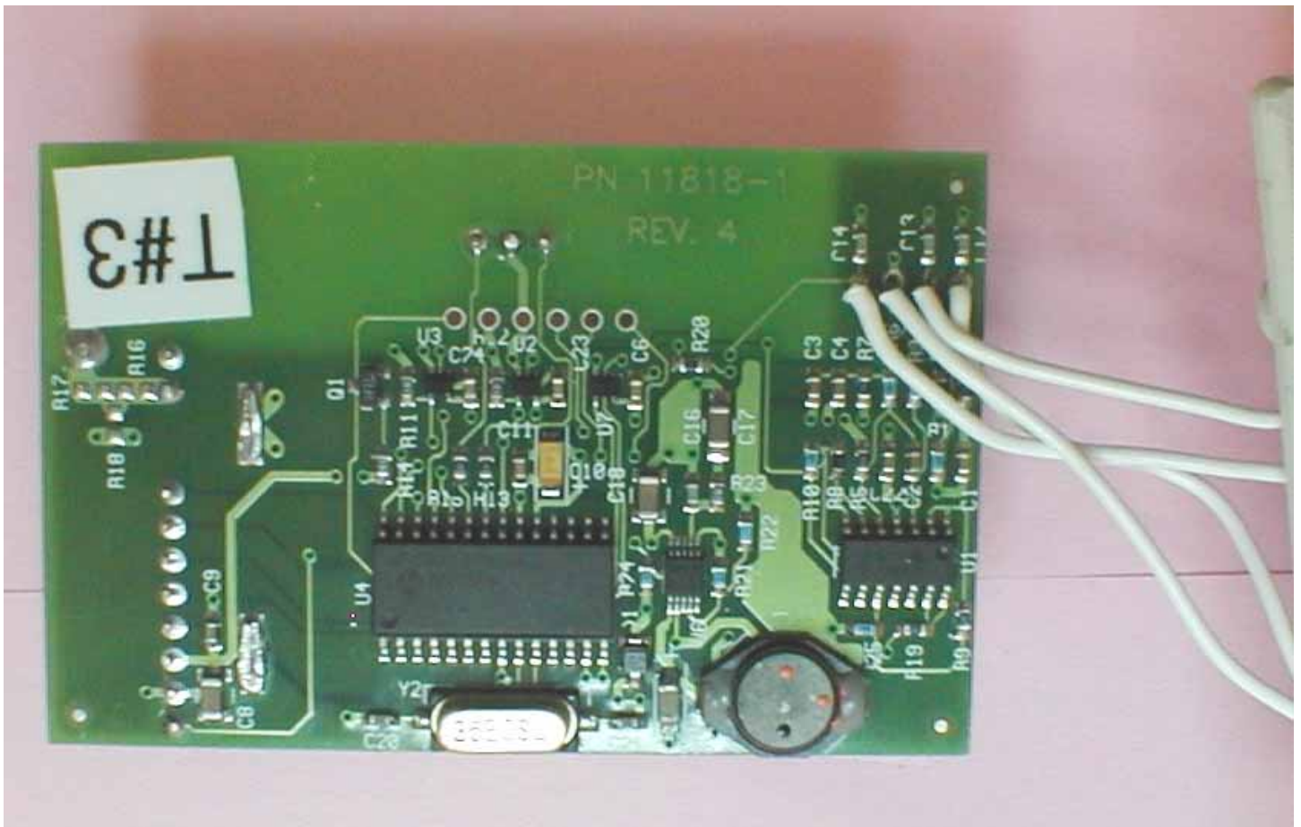
PCB Bottom View
