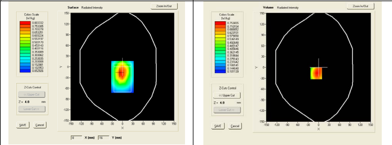
SAR, Z Axis Scan (X = -7, Y = -16)
