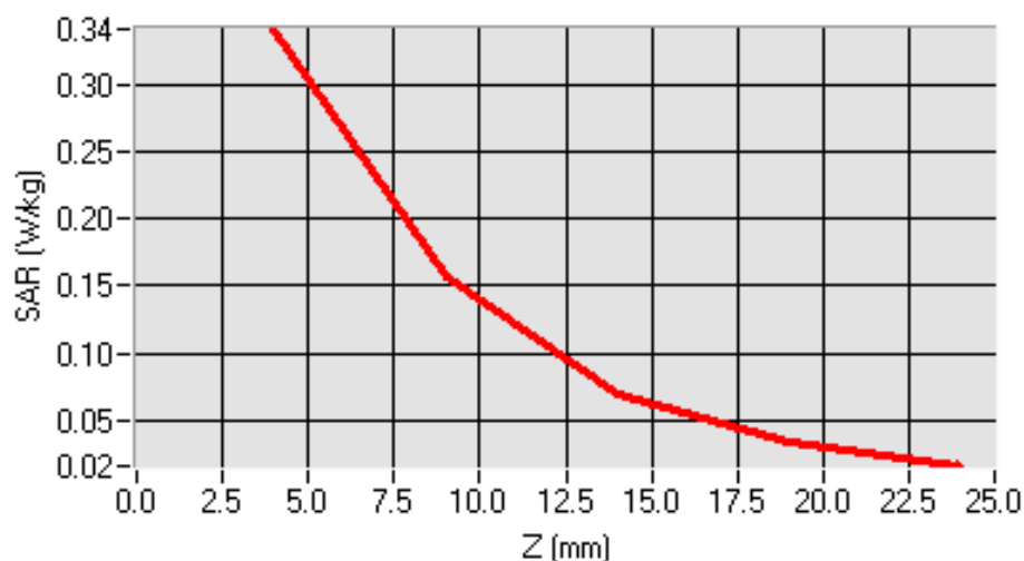
SAR, Z Axis Scan (X = -9, Y = -10)
