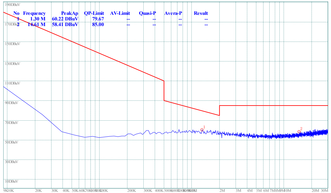
(Plot B.0: 9kHz to 30MHz @ GFSK, channel 39)
