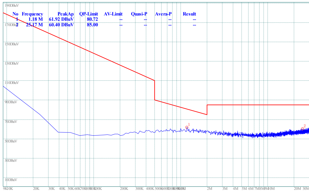
(Plot A.0: 9kHz to 30MHz @ GFSK, channel 0)
