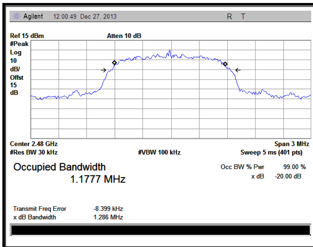
(Plot F: Channel = 2480 @ 1/4-DQPSK)
