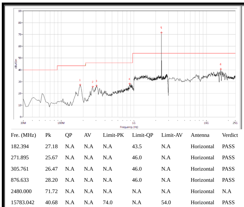
(Plot C.1: 30MHz to 25GHz, Antenna Horizontal @ GFSK, channel 78)
