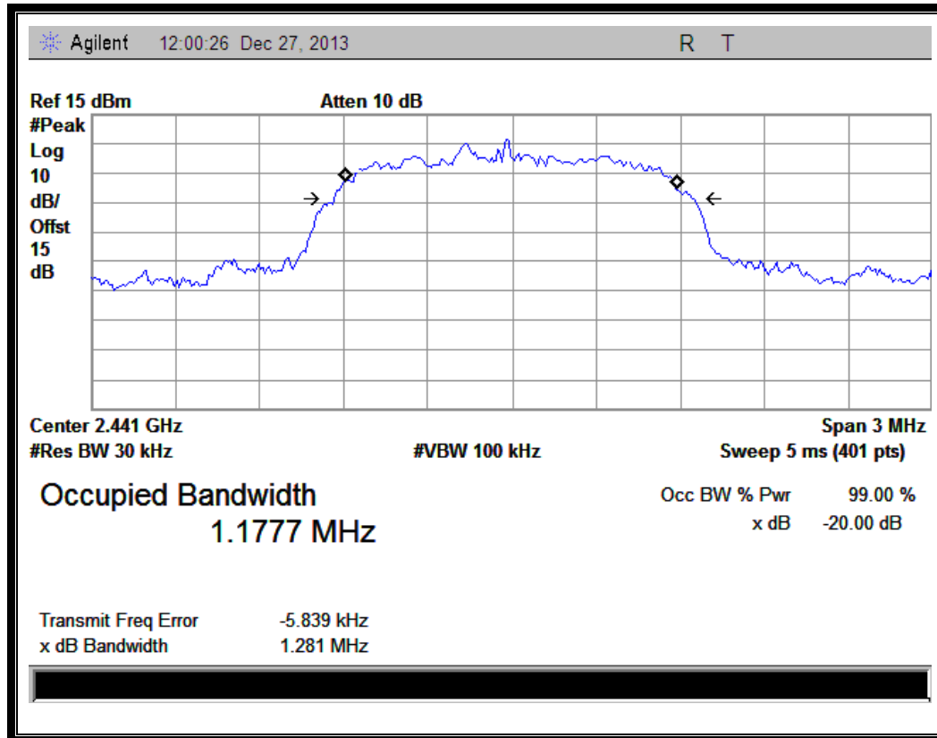
(Plot E: Channel = 2441 @ 1/4-DQPSK)
