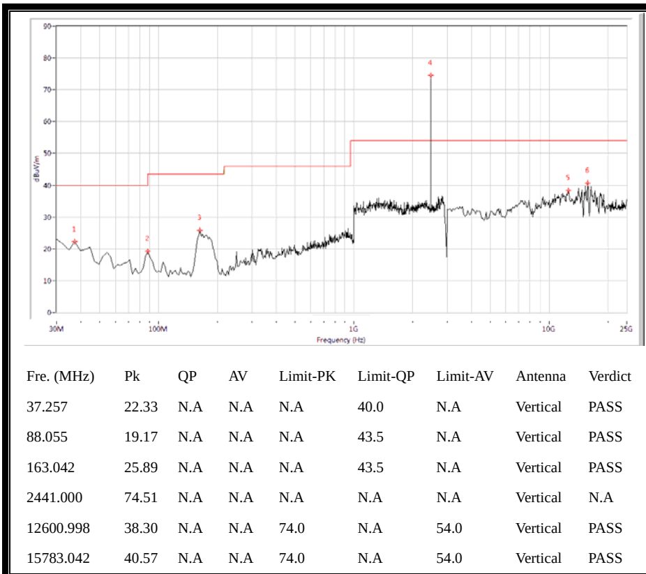
(Plot B.2: 30MHz to 25GHz, Antenna Vertical @8-DPSK, channel 39)
