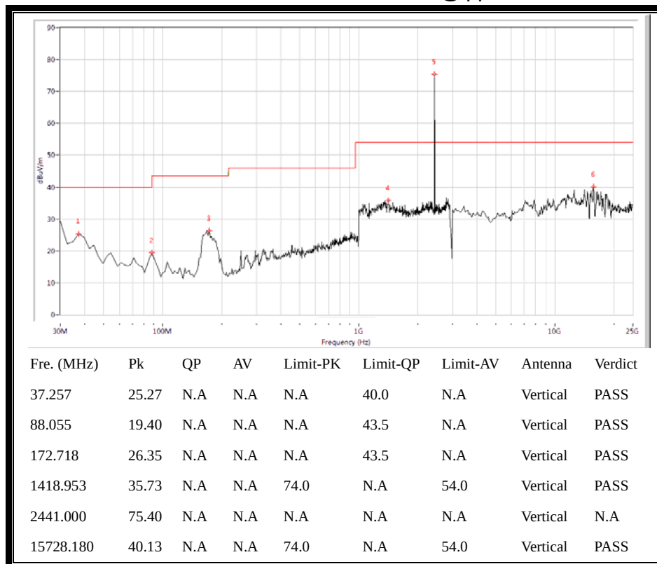
(Plot B.2: 30MHz to 25GHz, Antenna Vertical @ \pi/4 -DQPSK, channel 39)
