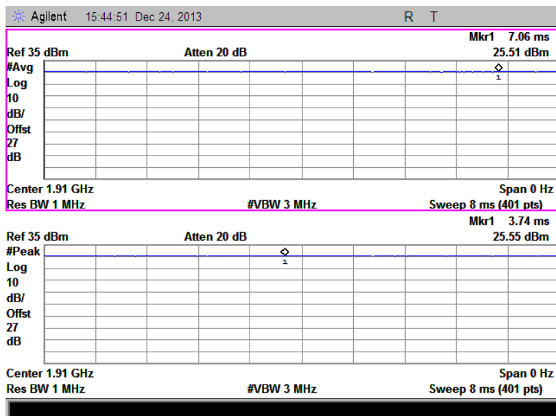
(Plot B3: EGPRS 1900MHz Channel = 810)
