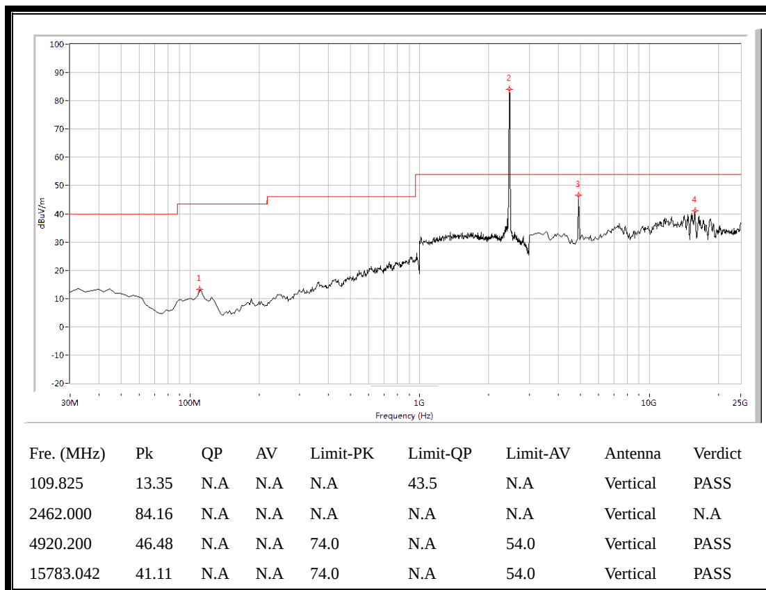
(Plot I.3: Antenna Vertical, 30MHz to 25GHz)
