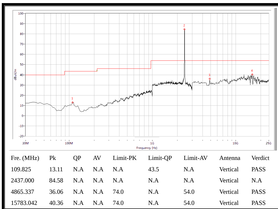
(Plot E.3: Antenna Vertical, 30MHz to 25GHz)
