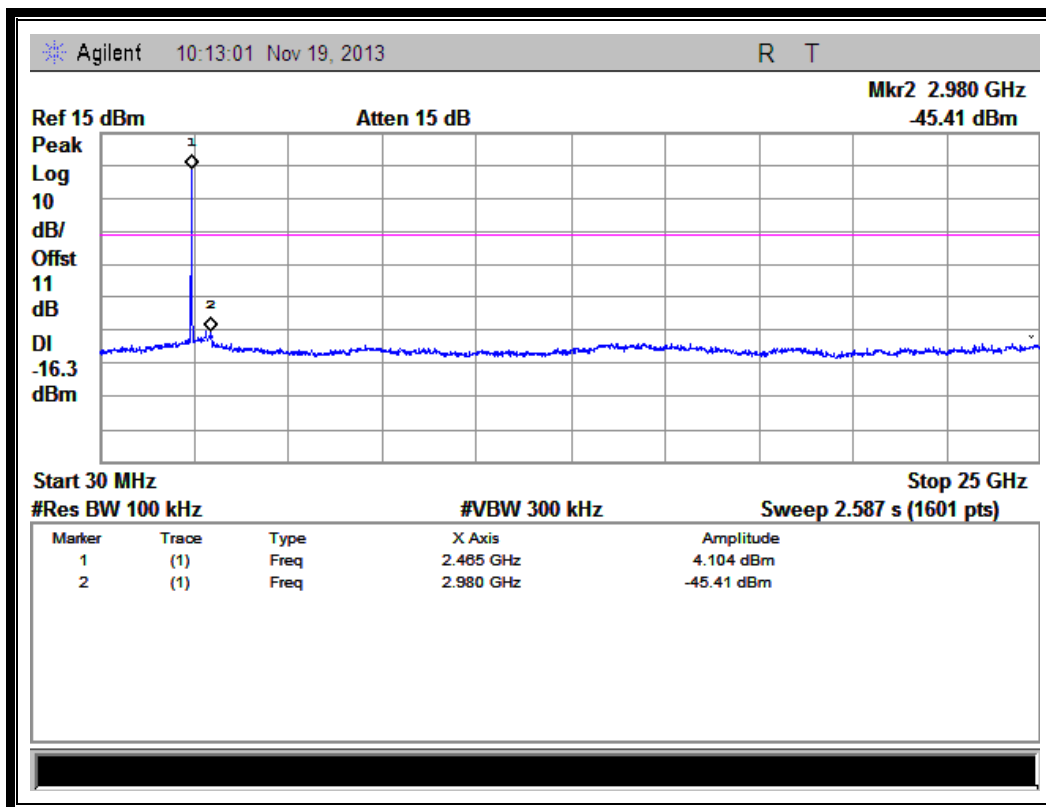
(Plot C.1: Channel = 11, 30MHz to 25GHz)
