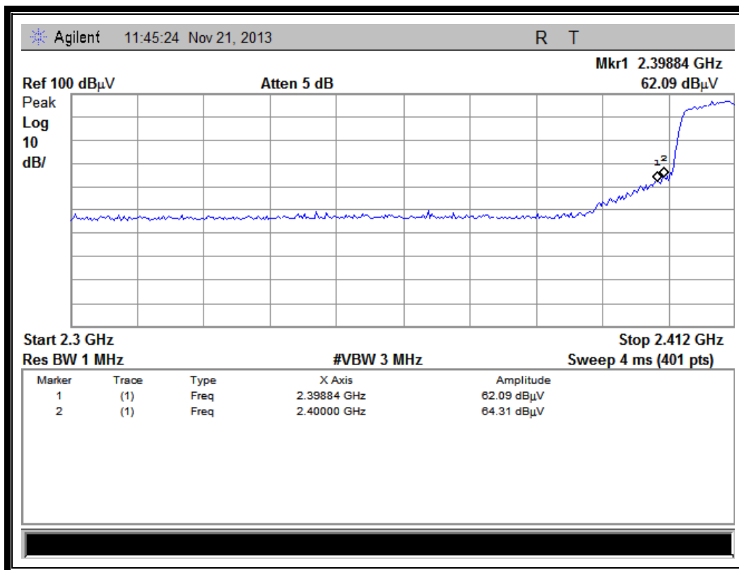
(Plot E1: Channel = 1 PEAK @ 802.11n-20)
