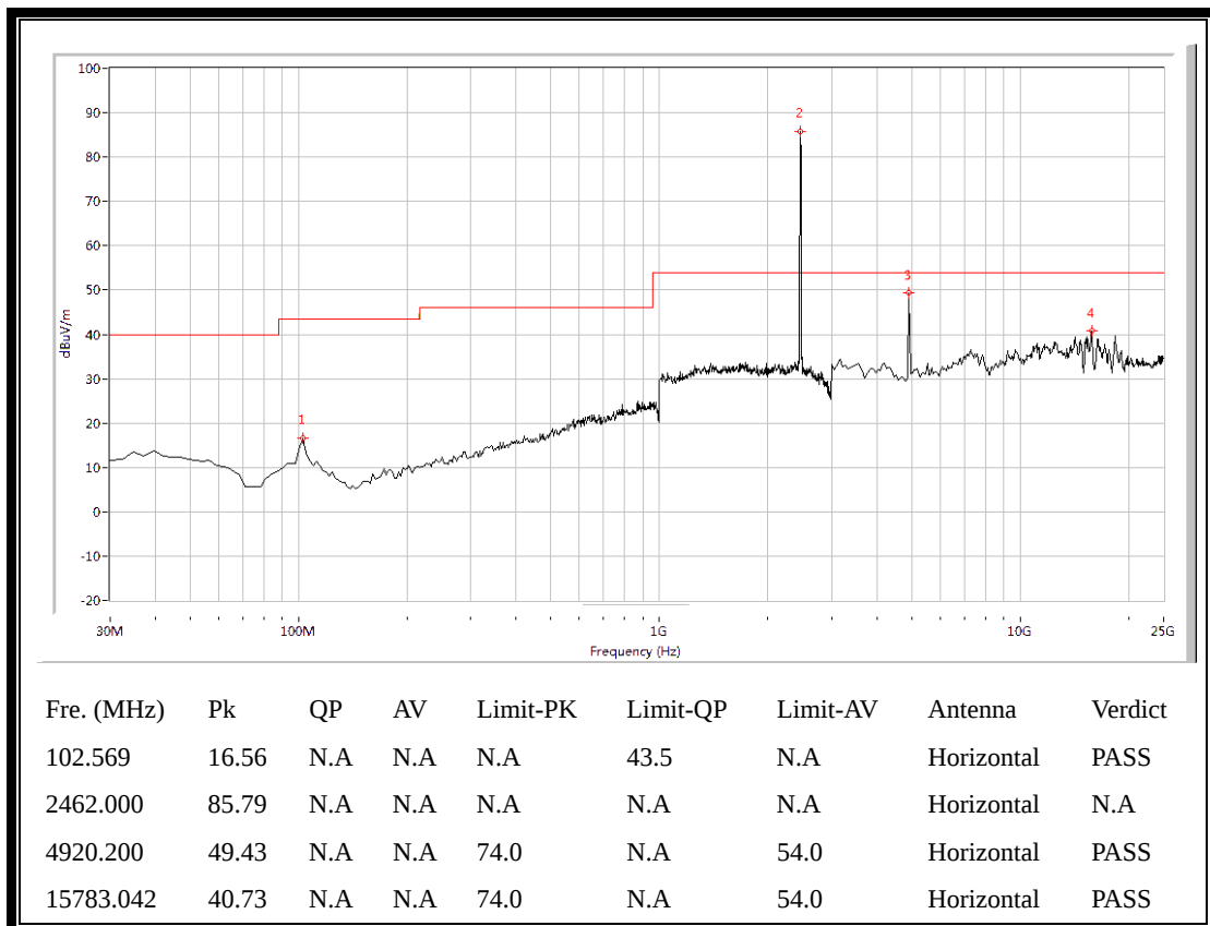
(Plot C.2: Antenna Horizontal, 30MHz to 25GHz)
