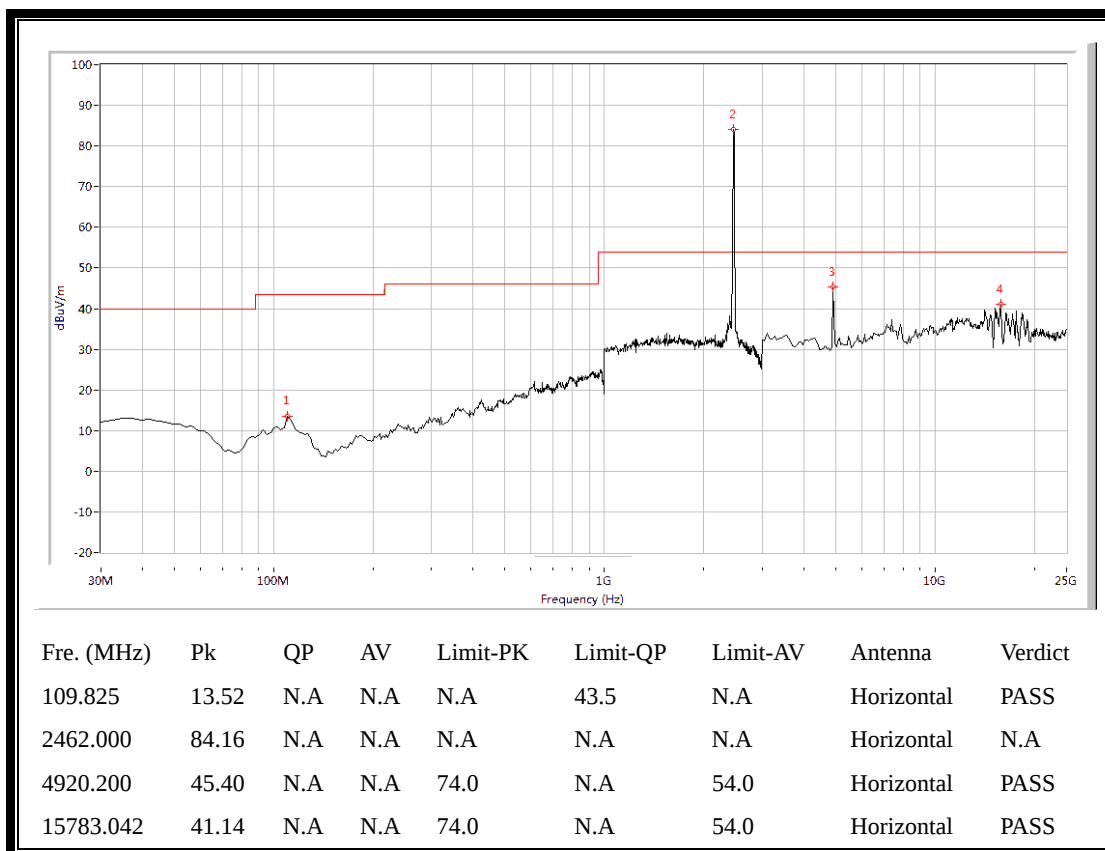
(Plot F.2: Antenna Horizontal, 30MHz to 25GHz)
