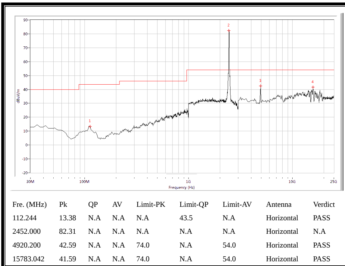
(Plot C.2: Antenna Horizontal, 30MHz to 25GHz)
