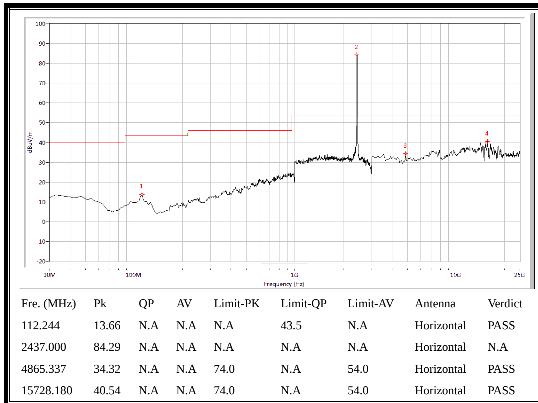
(Plot H.2: Antenna Horizontal, 30MHz to 25GHz)
