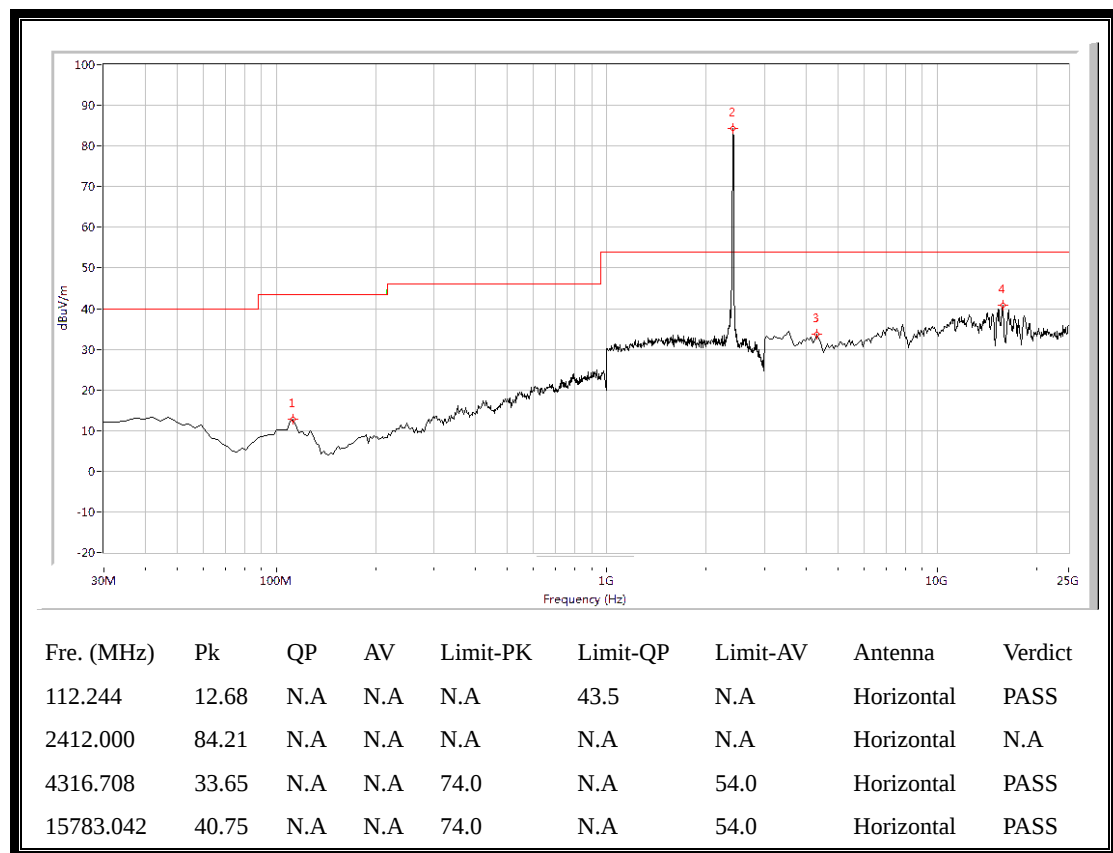
(Plot D.2: Antenna Horizontal, 30MHz to 25GHz)
