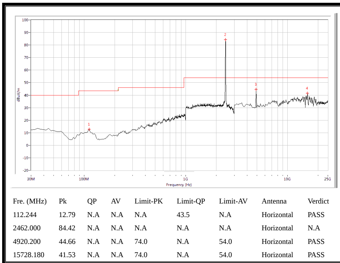
(Plot I.2: Antenna Horizontal, 30MHz to 25GHz)
