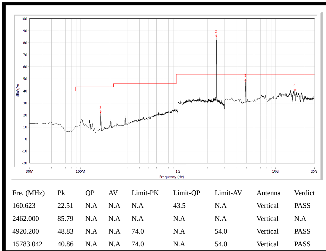
(Plot C.3: Antenna Vertical, 30MHz to 25GHz)
