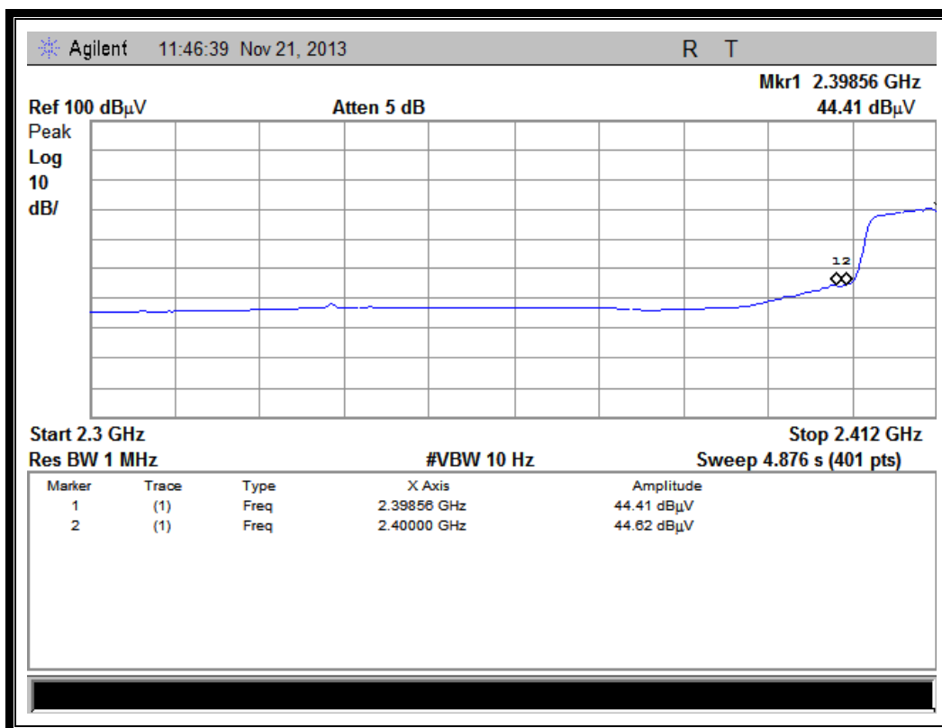
(Plot E2: Channel = 1 AVG @ 802.11n-20)
