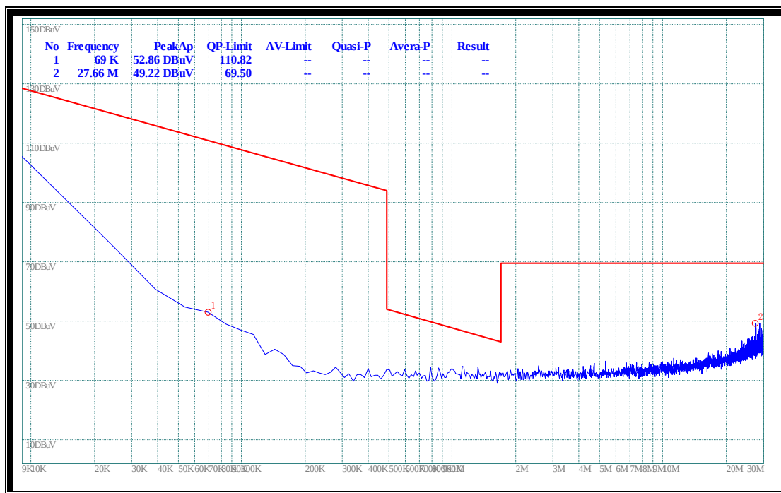
(Plot F.1: 9kHz to 30MHz)
