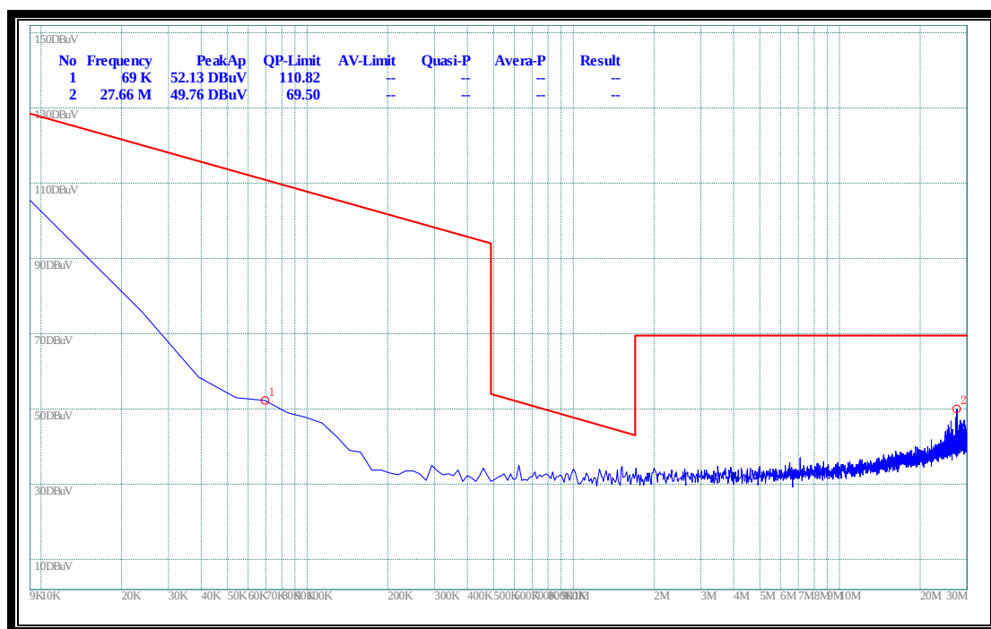
(Plot B.1: 9kHz to 30MHz)
