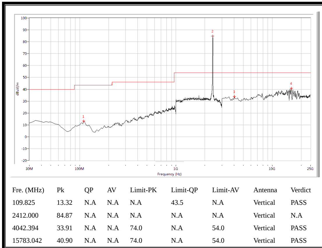
(Plot D.3: Antenna Vertical, 30MHz to 25GHz)
