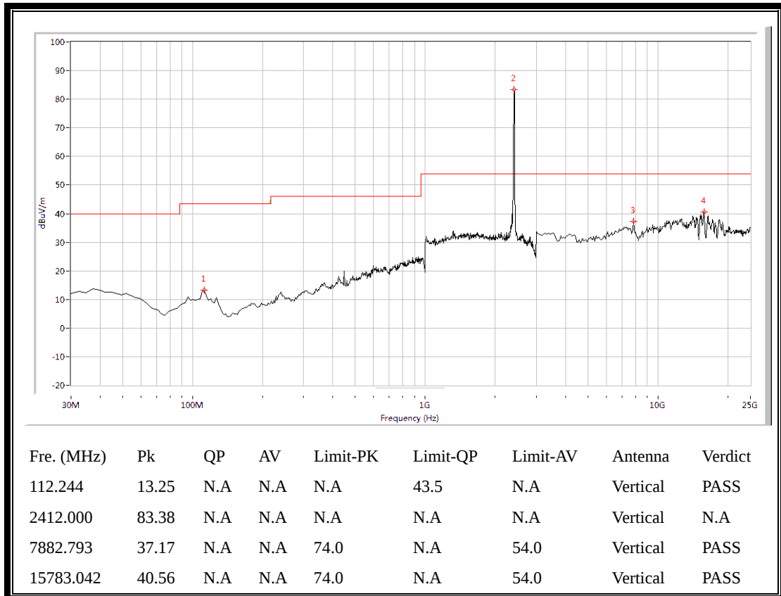
(Plot G.3: Antenna Vertical, 30MHz to 25GHz)
