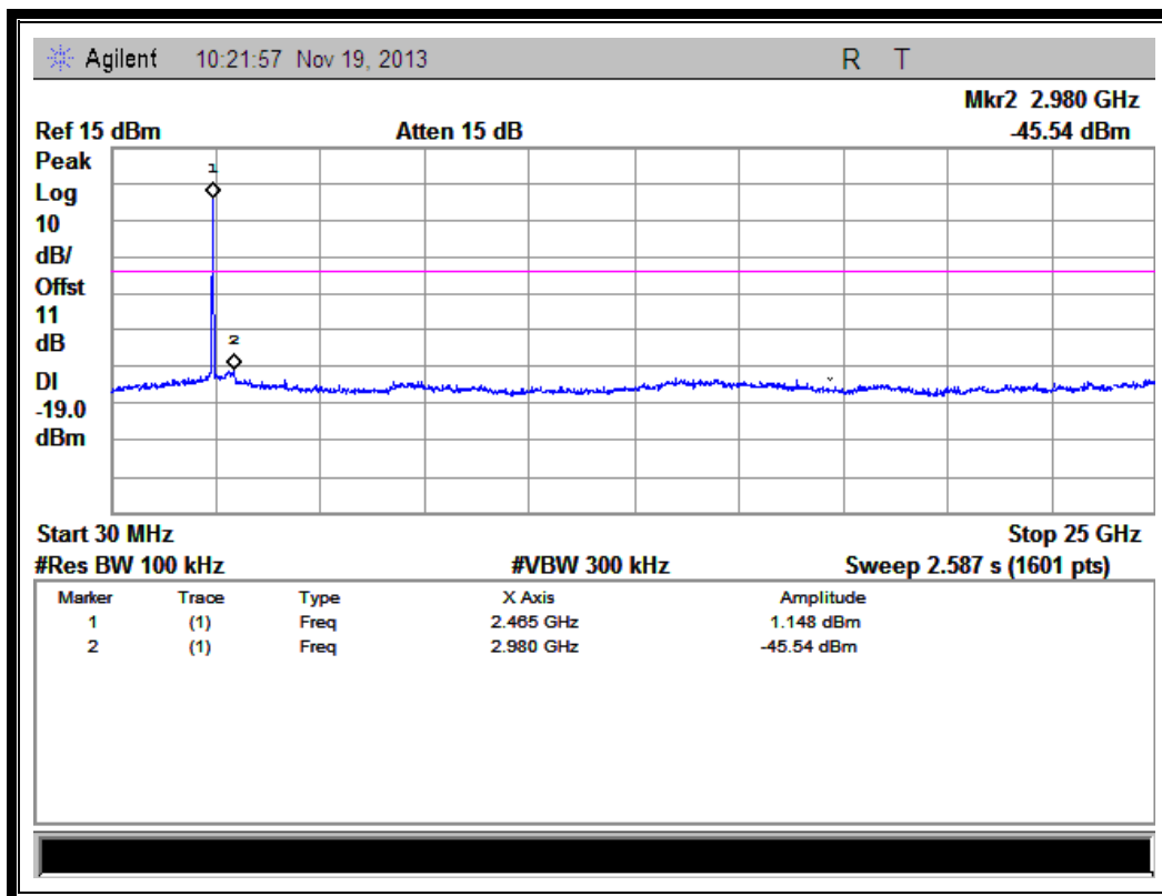
(Plot F.1: Channel = 11, 30MHz to 25GHz)
