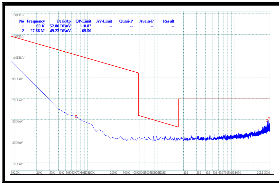
(Plot C.1: 9kHz to 30MHz)
