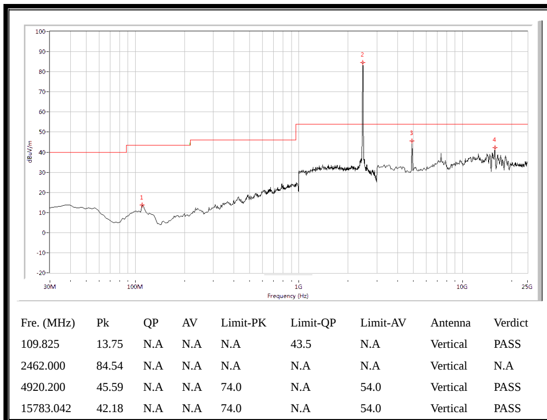
(Plot F.3: Antenna Vertical, 30MHz to 25GHz)
