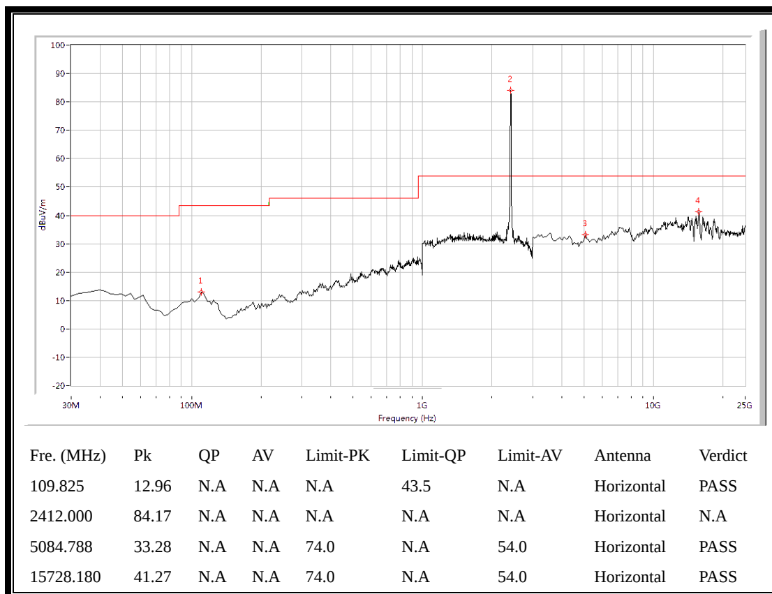
(Plot G.2: Antenna Horizontal, 30MHz to 25GHz)
