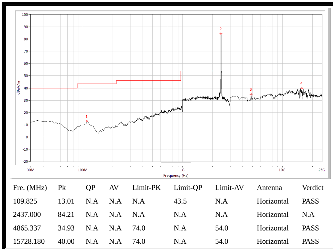
(Plot E.2: Antenna Horizontal, 30MHz to 25GHz)
