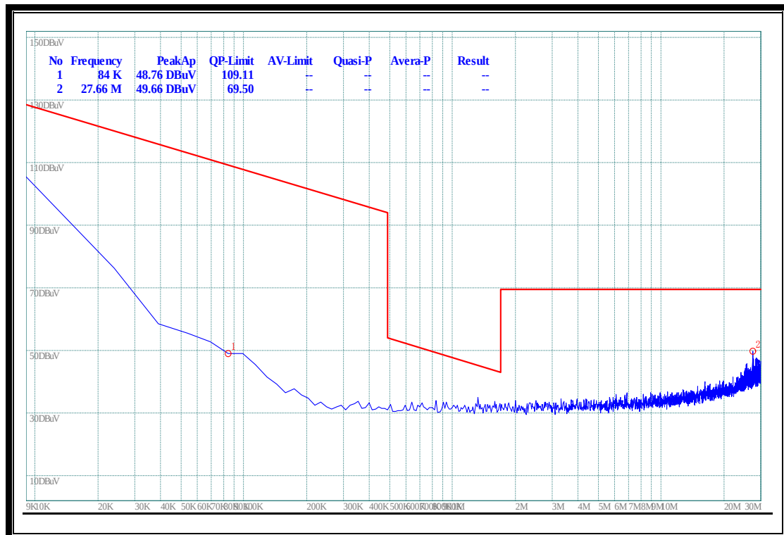
(Plot A.1: 9kHz to 30MHz)
