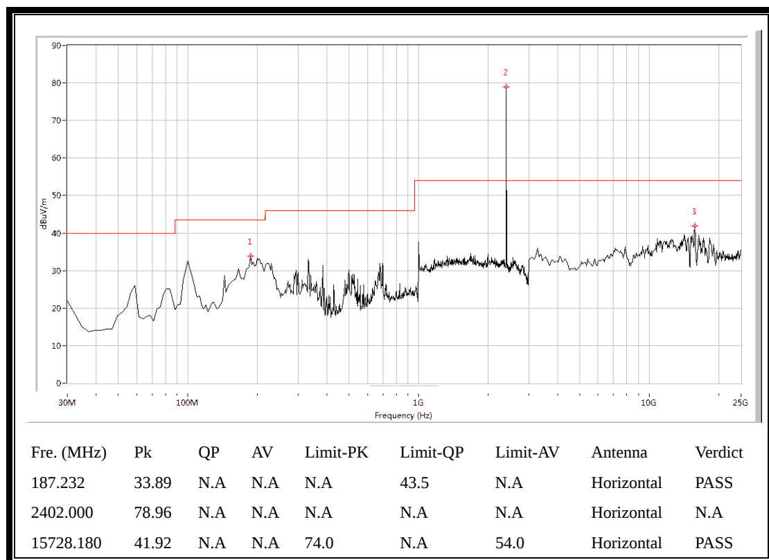
(Plot A.1: 30MHz to 25GHz, Antenna Horizontal @ 1/4-DQPSK, channel 0)
