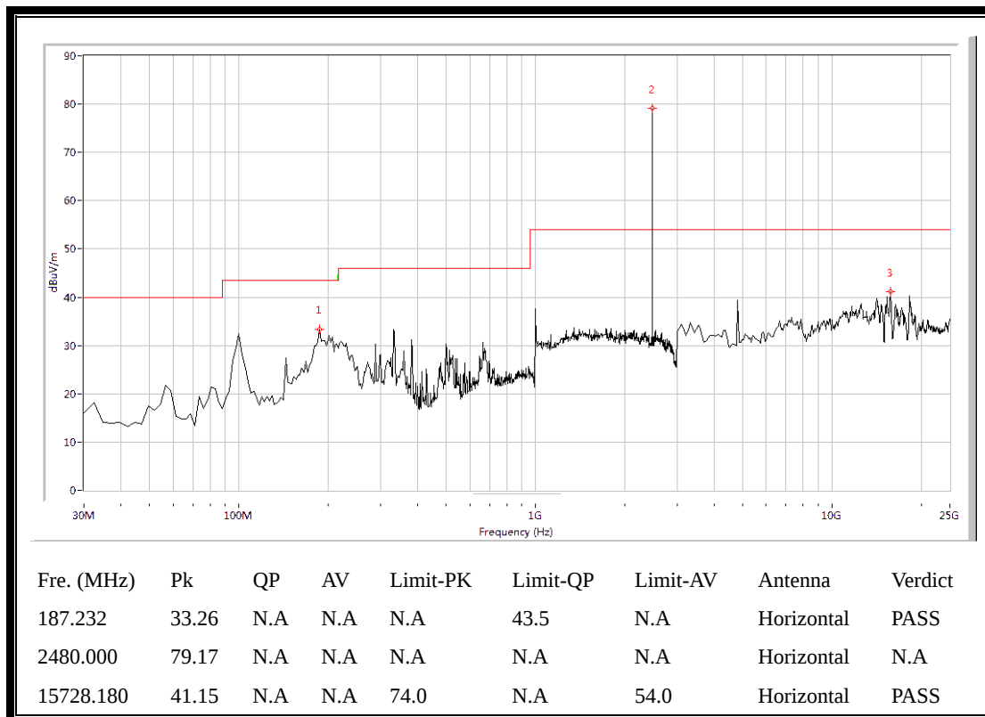
(Plot C.1: 30MHz to 25GHz, Antenna Horizontal @ \pi/4 -DQPSK, channel 78)
