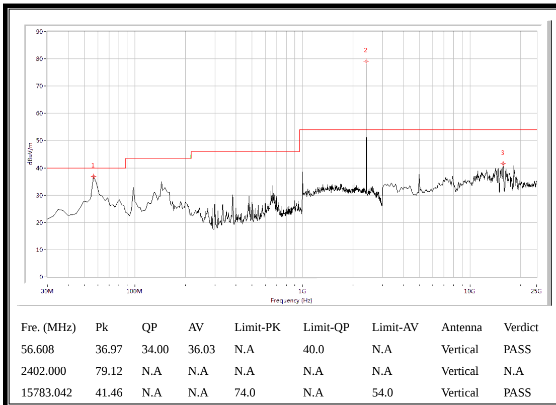
(Plot A.2: 30MHz to 25GHz, Antenna Vertical @ 1/4-DQPSK, channel 0)
