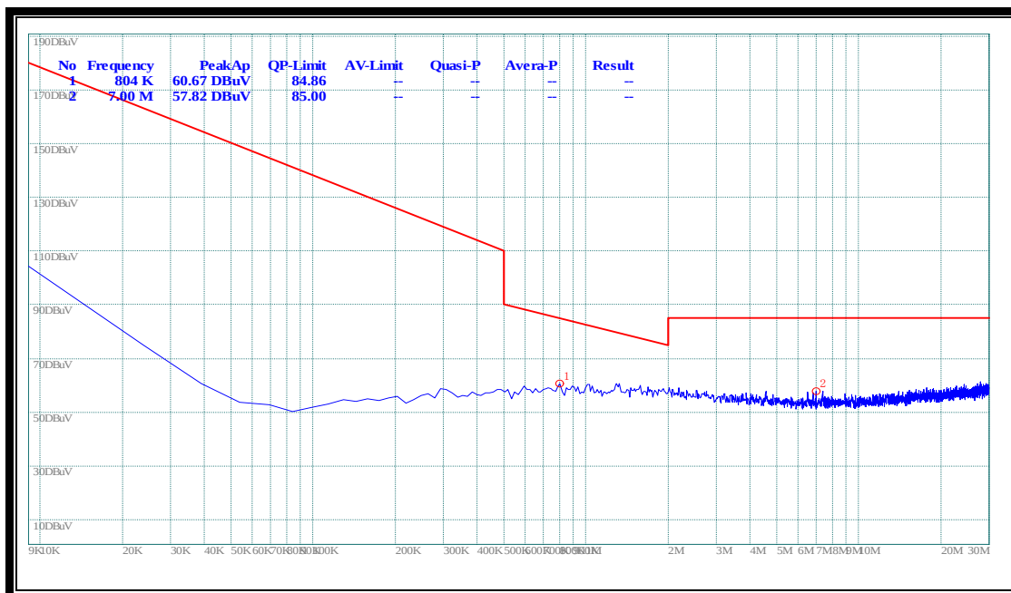
(Plot B.0: 9kHz to 30MHz @ 1/4-DQPSK, channel 39)
