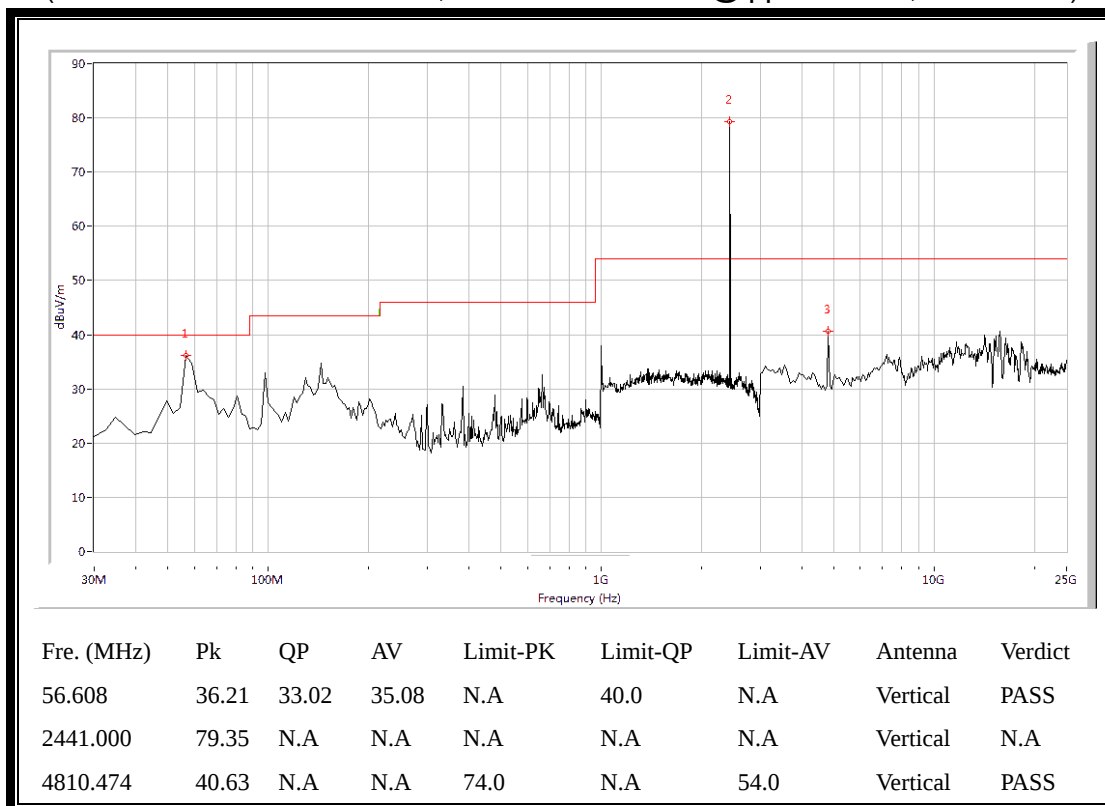
(Plot B.2: 30MHz to 25GHz, Antenna Vertical @ \pi/4 -DQPSK, channel 39)
