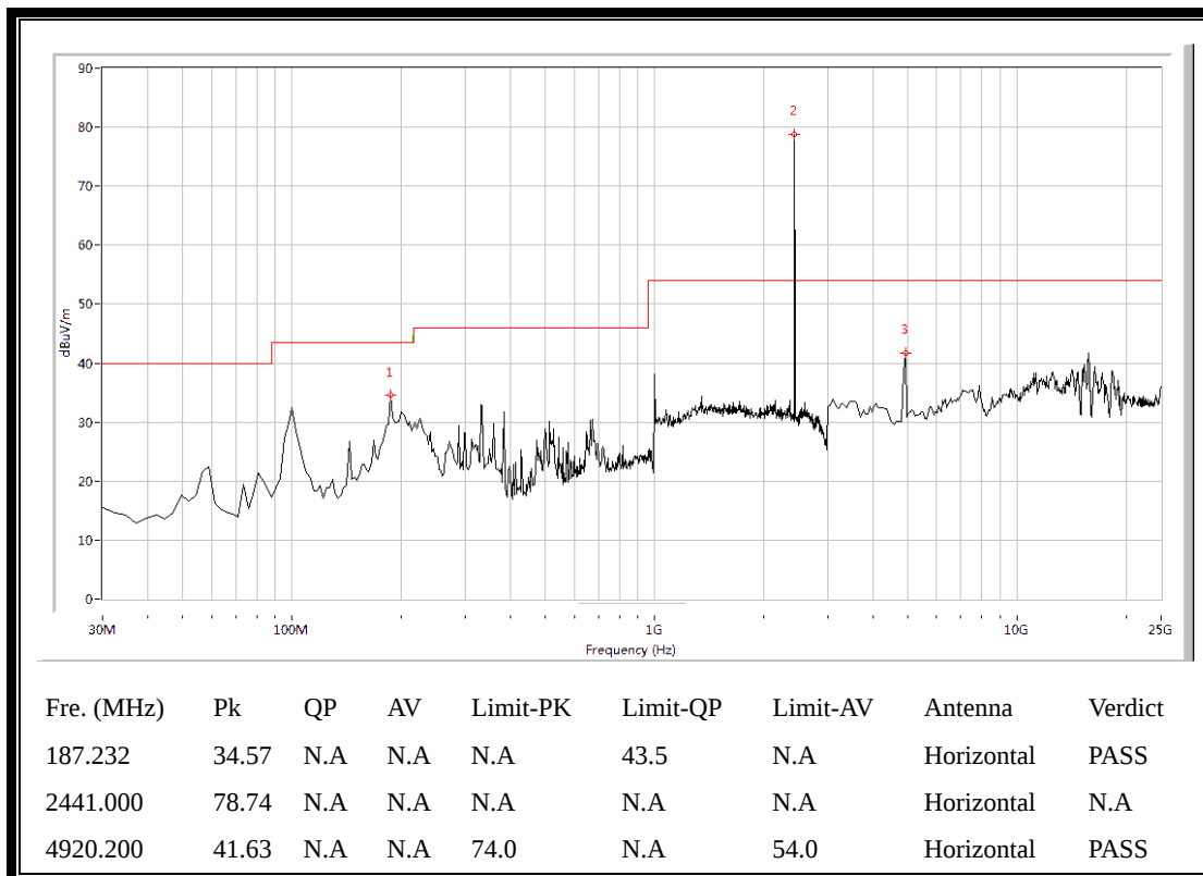
(Plot B.1: 30MHz to 25GHz, Antenna Horizontal @ \pi/4 -DQPSK, channel 39)
