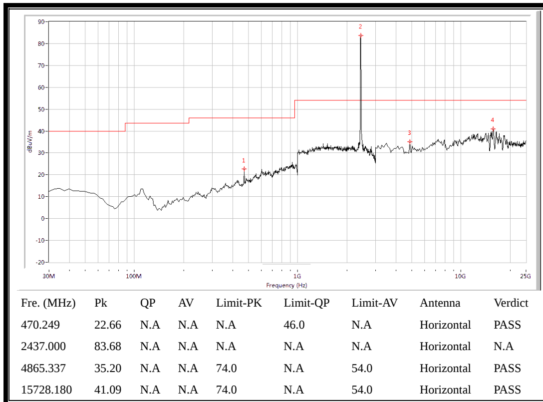
(Plot H.2: Antenna Horizontal, 30MHz to 25GHz)
