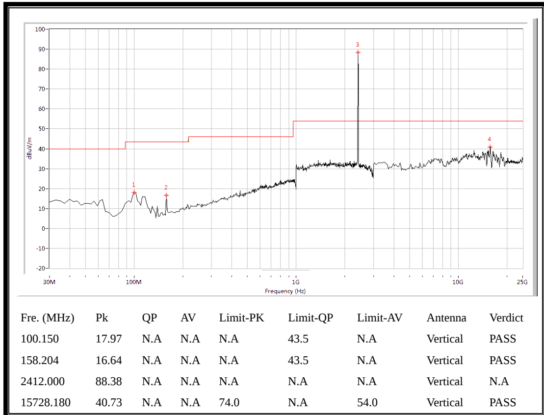
(Plot A.3: Antenna Vertical, 30MHz to 25GHz)
