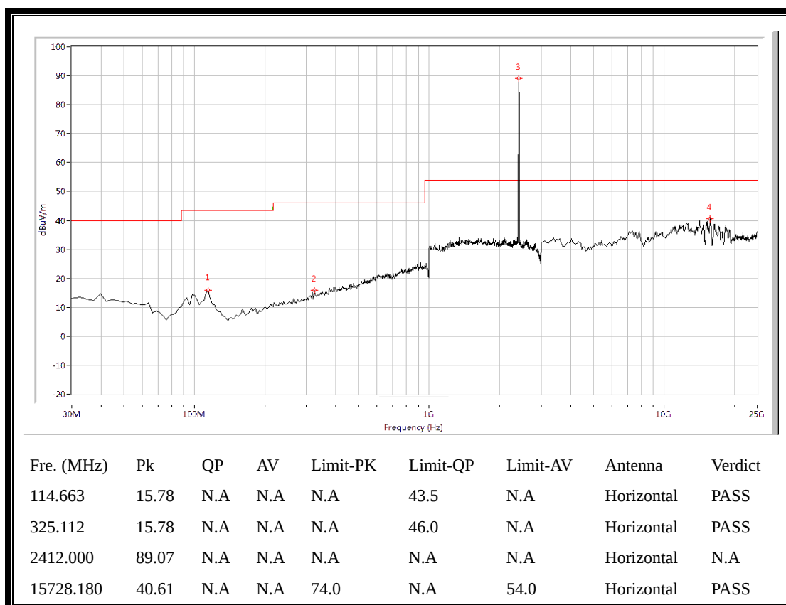
(Plot A.2: Antenna Horizontal, 30MHz to 25GHz)
