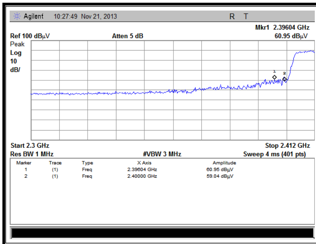
(Plot E1: Channel = 3 PEAK @ 802.11n-40)
