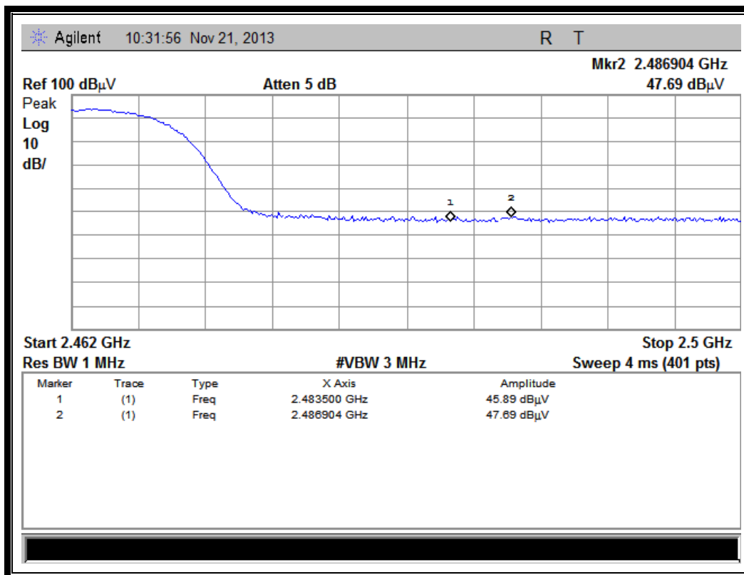
(Plot B1: Channel = 11 PEAK @ 802.11b)
