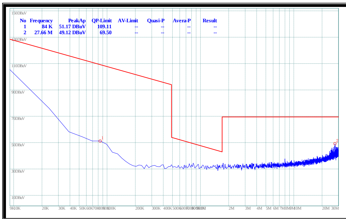
(Plot C.1: 9kHz to 30MHz)
