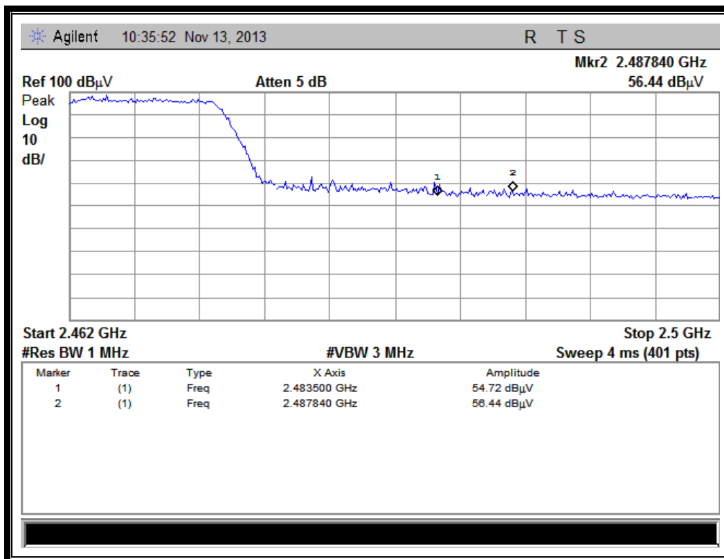
(Plot F1: Channel = 11 PEAK @ 802.11n-20)
