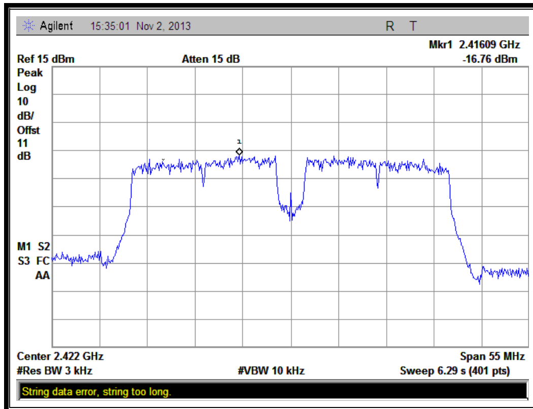
(Plot G: Channel = 3 @ 802.11n-40MHz)
