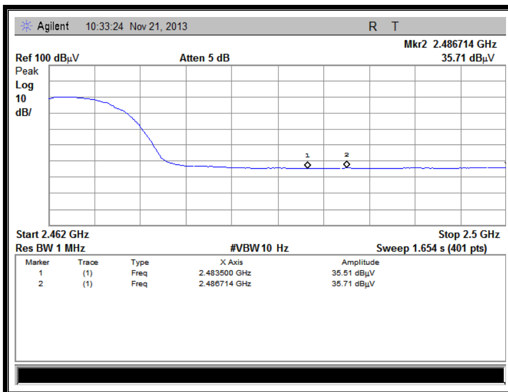
(Plot B2: Channel = 11 AVG @ 802.11b)
