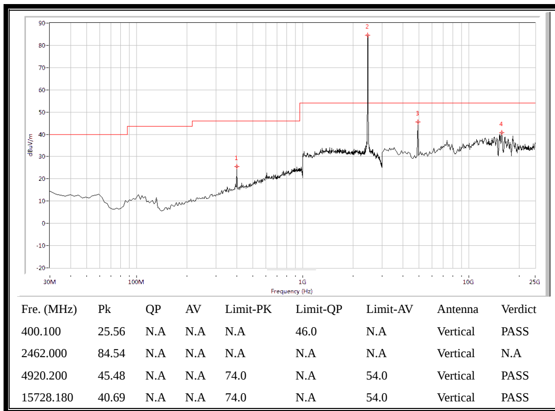
(Plot F.3: Antenna Vertical, 30MHz to 25GHz)
