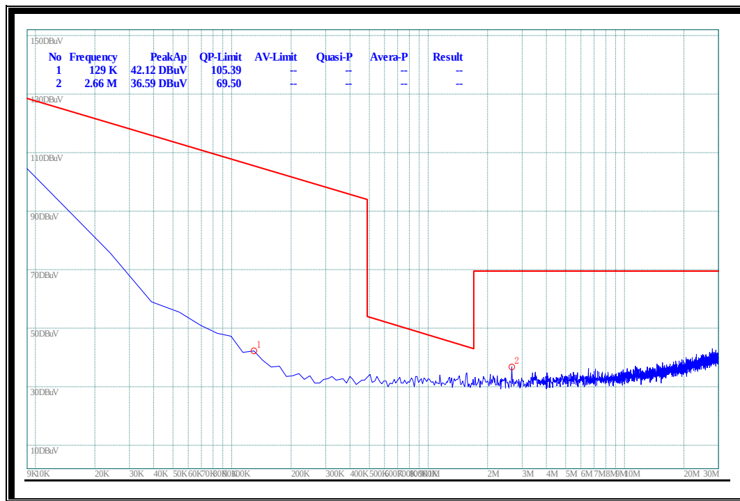
(Plot B.1: 9kHz to 30MHz)
