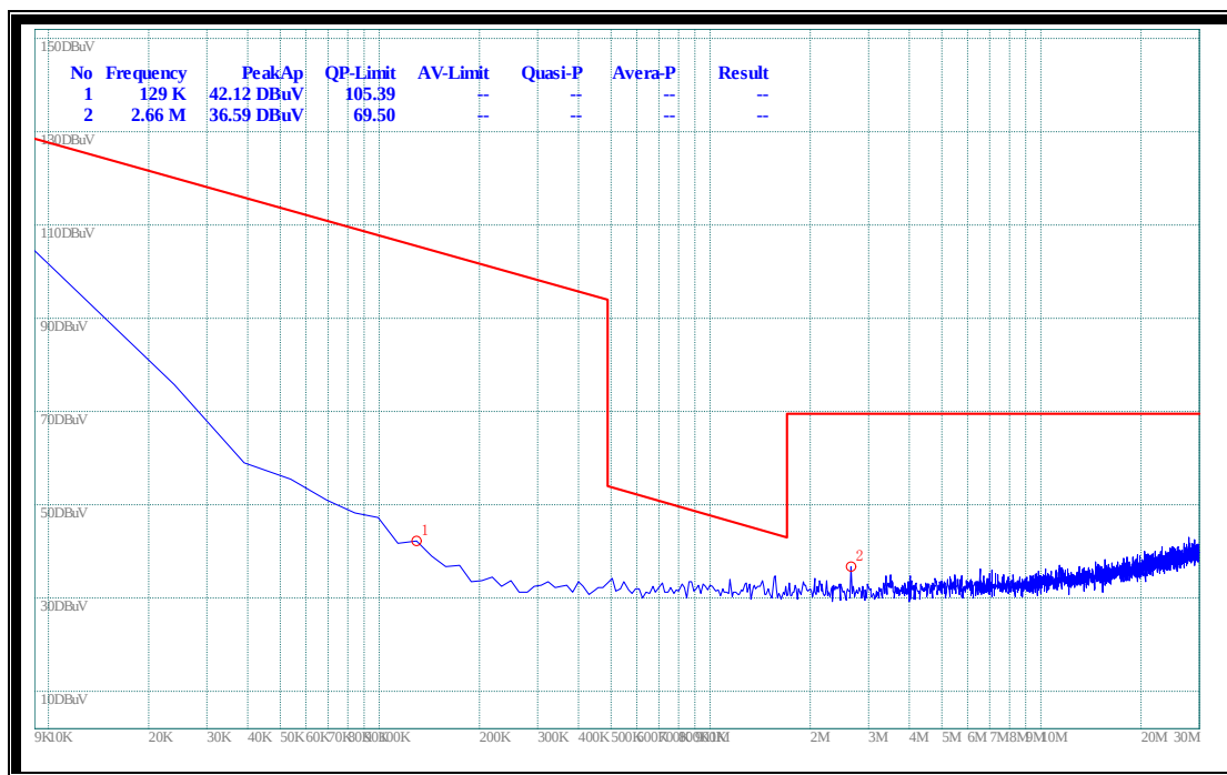
(Plot I.1: 9kHz to 30MHz)
