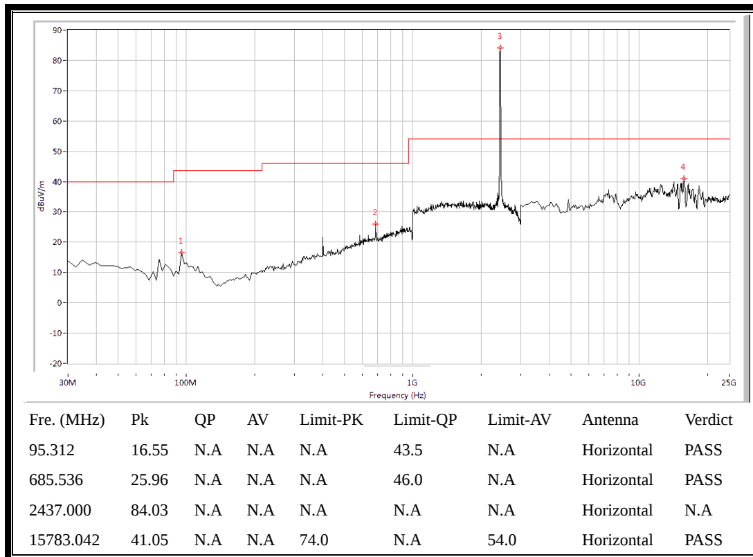
(Plot E.2: Antenna Horizontal, 30MHz to 25GHz)
