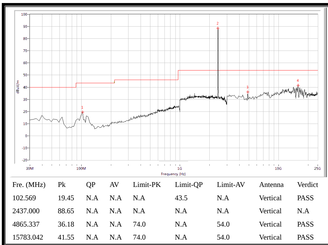
(Plot B.3: Antenna Vertical, 30MHz to 25GHz)
