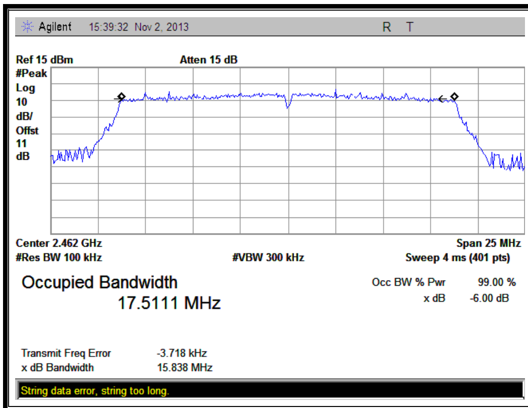
(Plot I: Channel 11: 2462MHz @ 802.11n-20)
