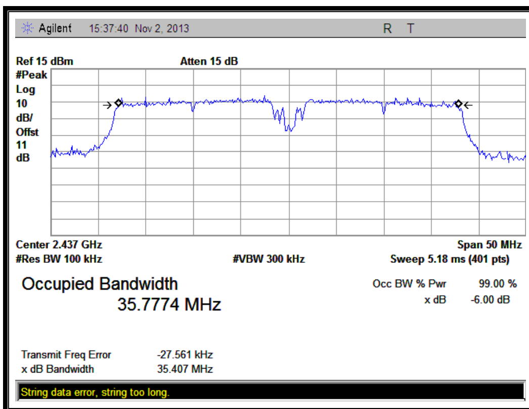
(Plot H: Channel 6: 2437MHz @ 802.11n-40)
