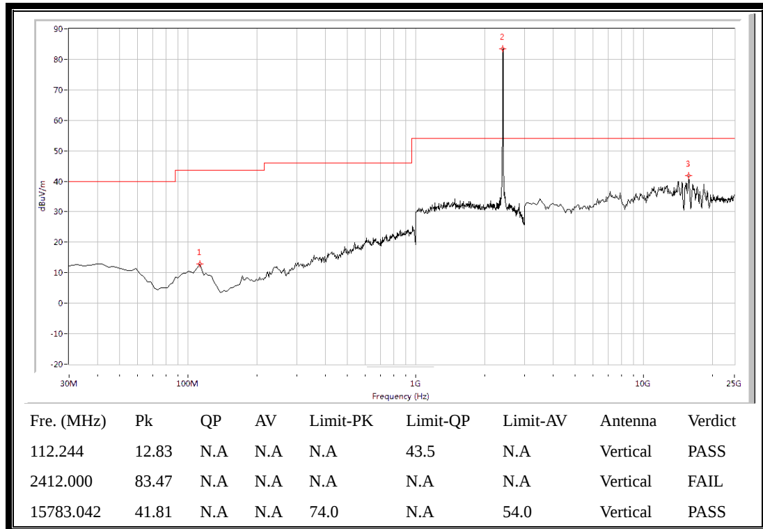
(Plot G.3: Antenna Vertical, 30MHz to 25GHz)
