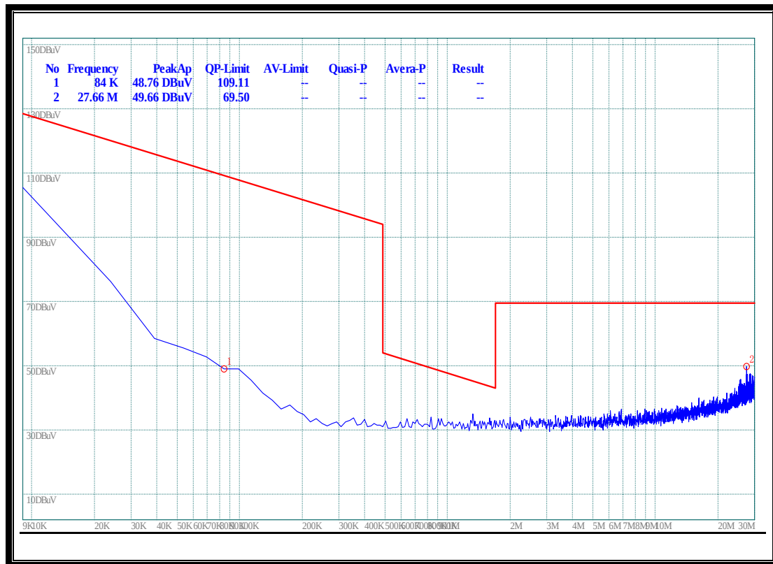
(Plot A.1: 9kHz to 30MHz)
