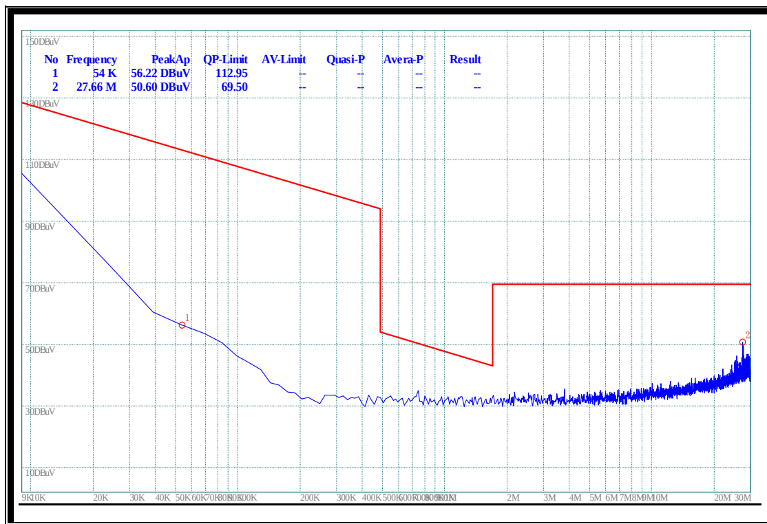
(Plot D.1: 9kHz to 30MHz)
