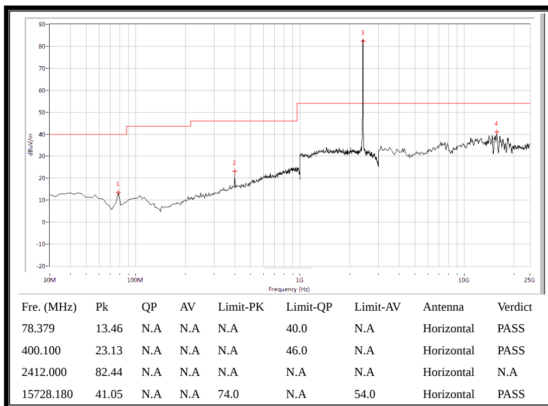
(Plot D.2: Antenna Horizontal, 30MHz to 25GHz)
