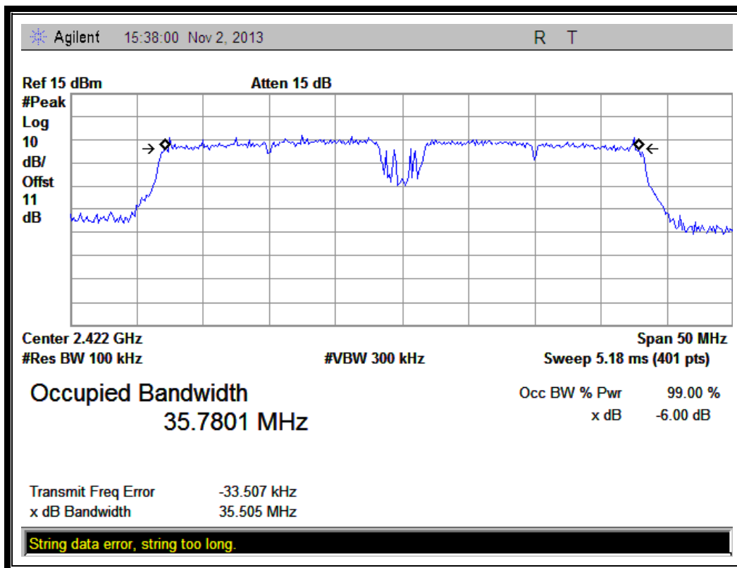
(Plot G: Channel 3: 2422MHz @ 802.11n-40)
