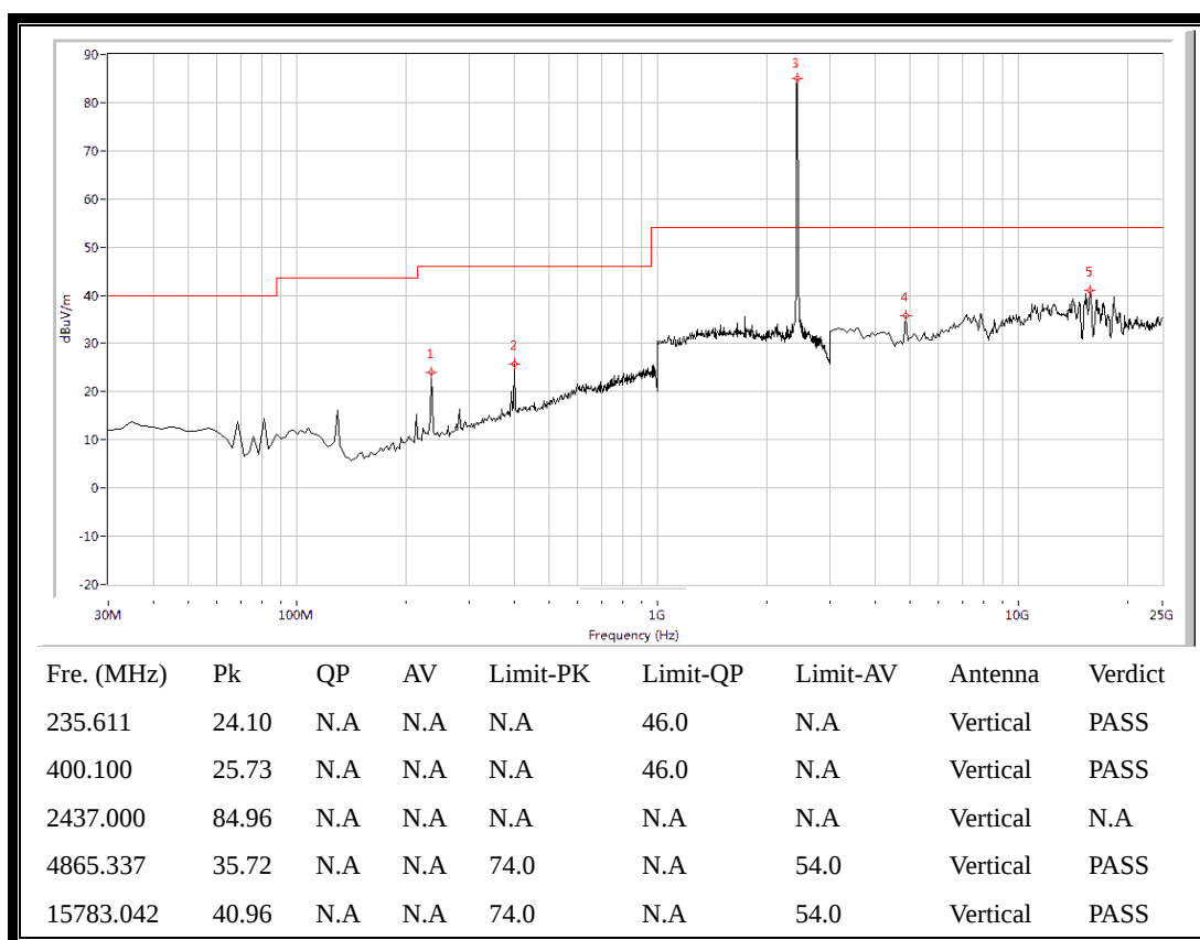
(Plot E.3: Antenna Vertical, 30MHz to 25GHz)
