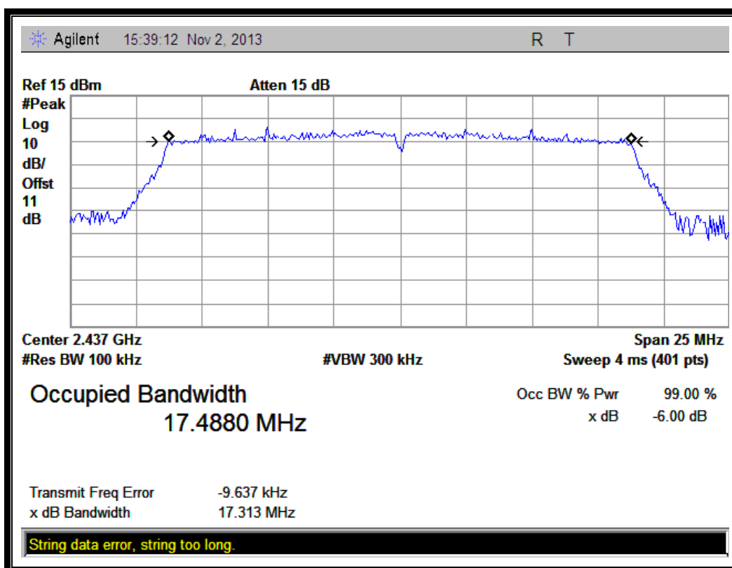
(Plot H: Channel 6: 2437MHz @ 802.11n-20)
