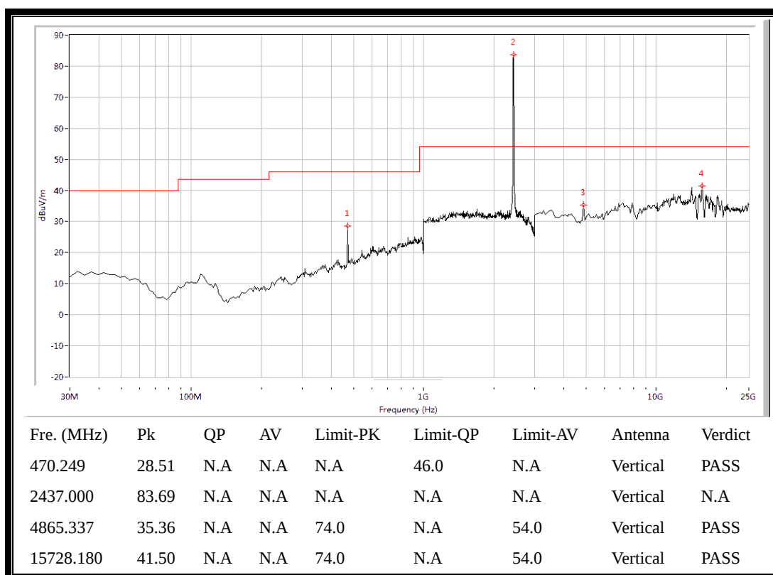
(Plot H.3: Antenna Vertical, 30MHz to 25GHz)
