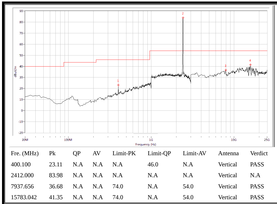
(Plot D.3: Antenna Vertical, 30MHz to 25GHz)
