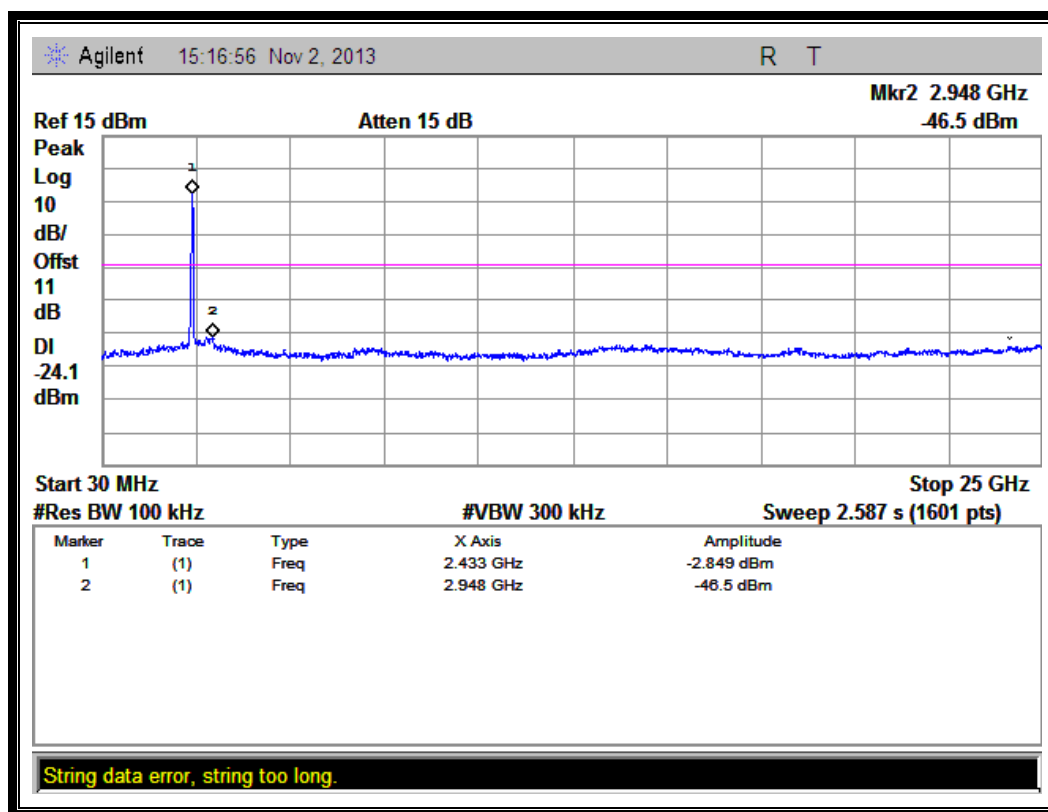
(Plot G.1: Channel = 3, 30MHz to 25GHz)
