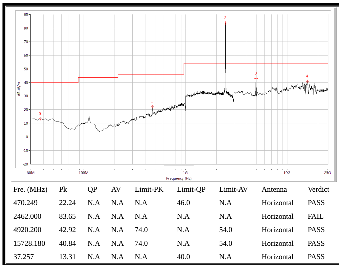
(Plot I.2: Antenna Horizontal, 30MHz to 25GHz)
