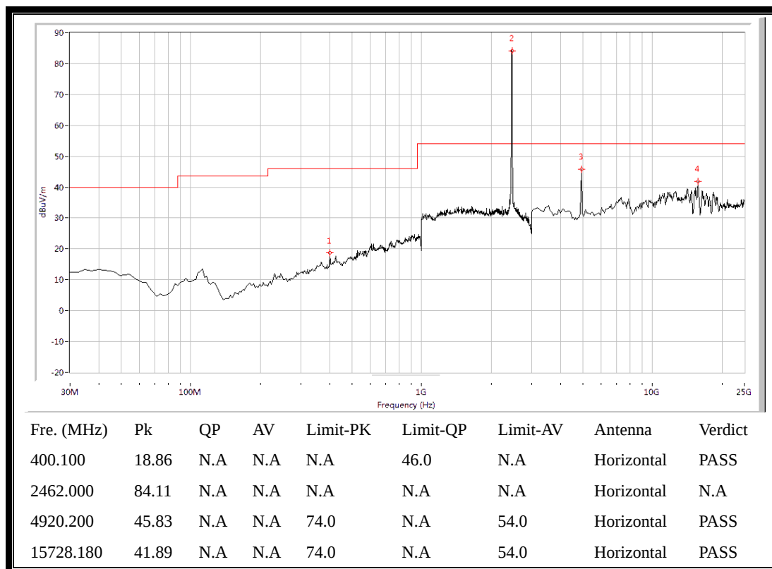
(Plot F.2: Antenna Horizontal, 30MHz to 25GHz)
