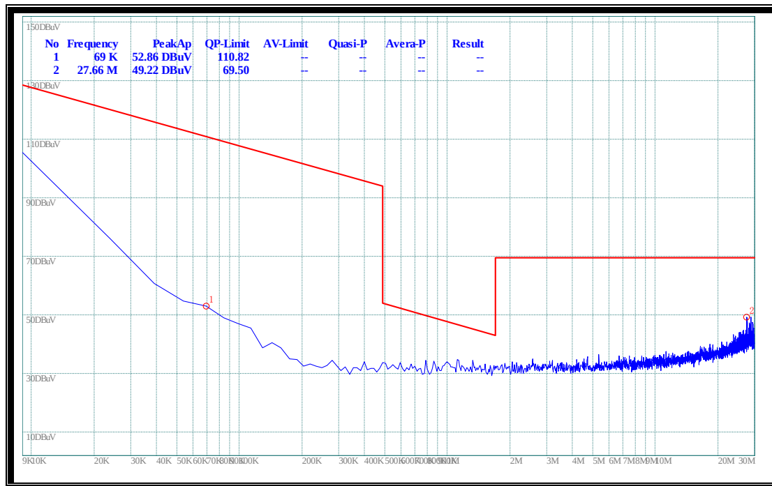
(Plot F.1: 9kHz to 30MHz)
