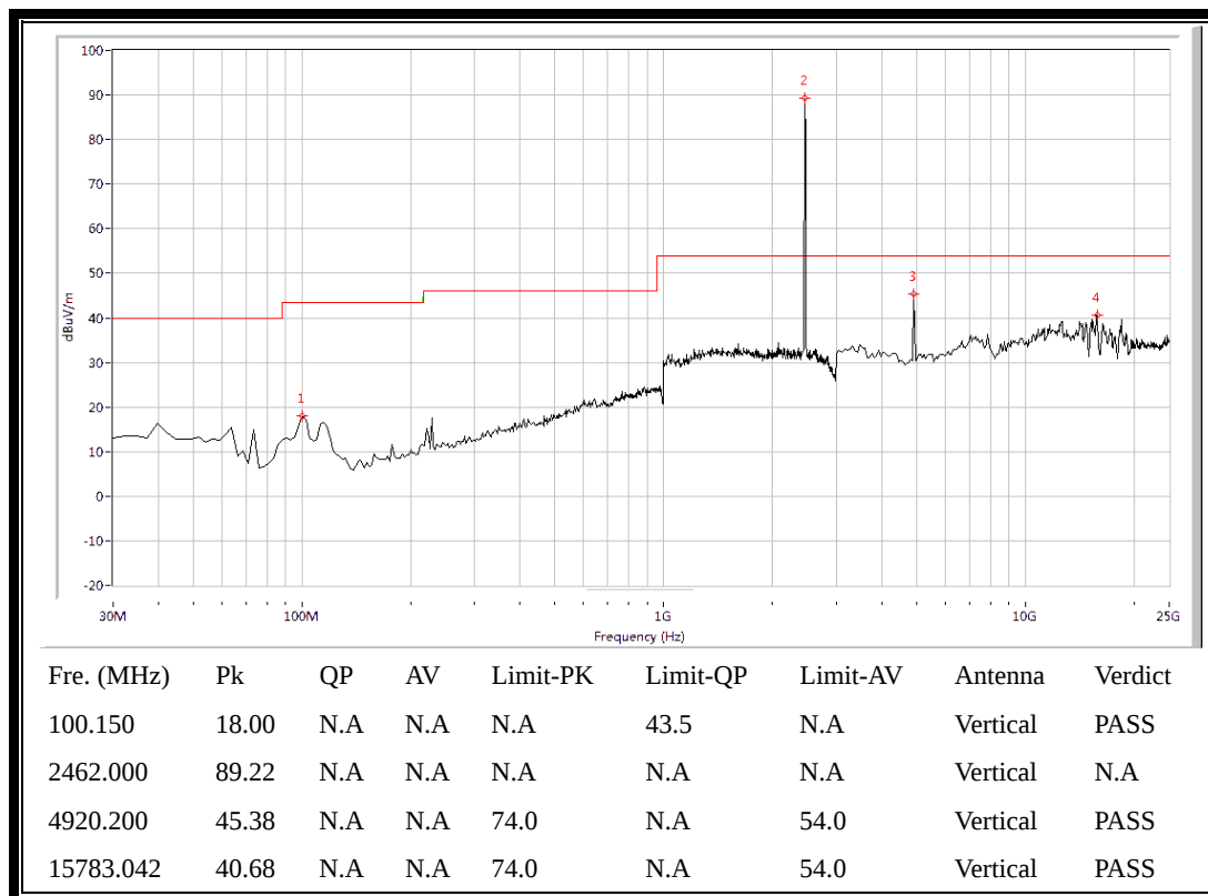
(Plot C.3: Antenna Vertical, 30MHz to 25GHz)
