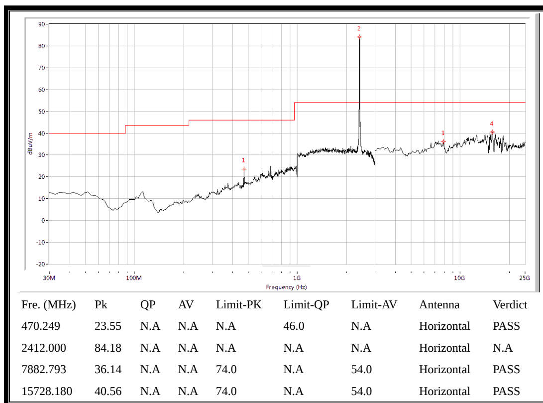
(Plot G.2: Antenna Horizontal, 30MHz to 25GHz)
