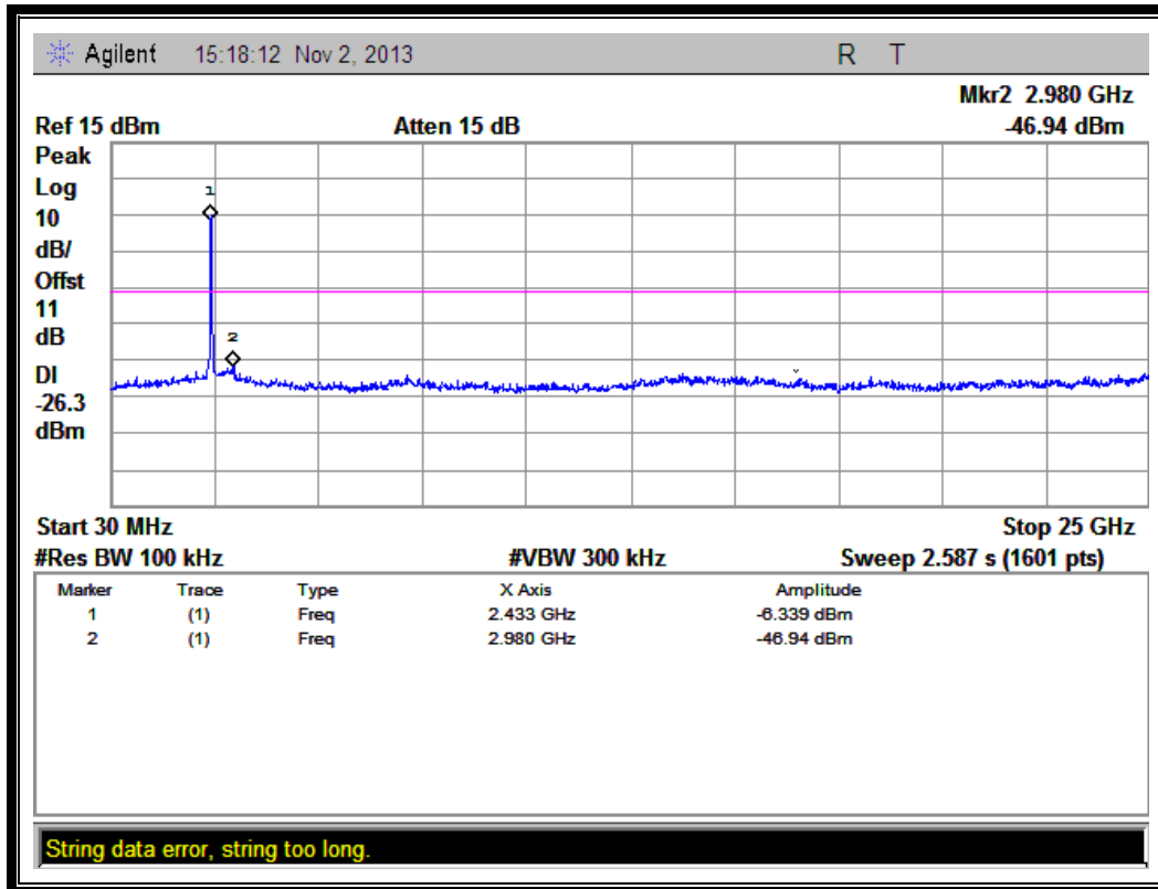
(Plot I.1: Channel = 9, 30MHz to 25GHz)
