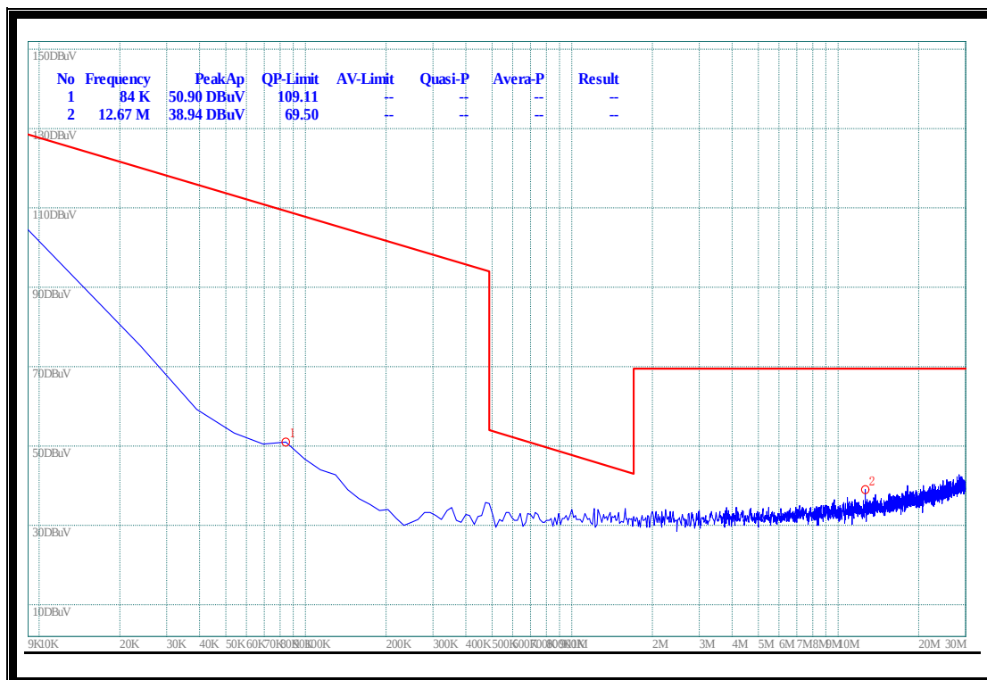
(Plot G.1: 9kHz to 30MHz)
