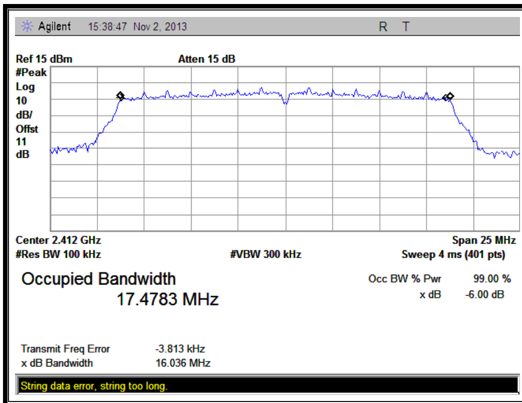
(Plot G: Channel 1: 2412MHz @ 802.11n-20)
