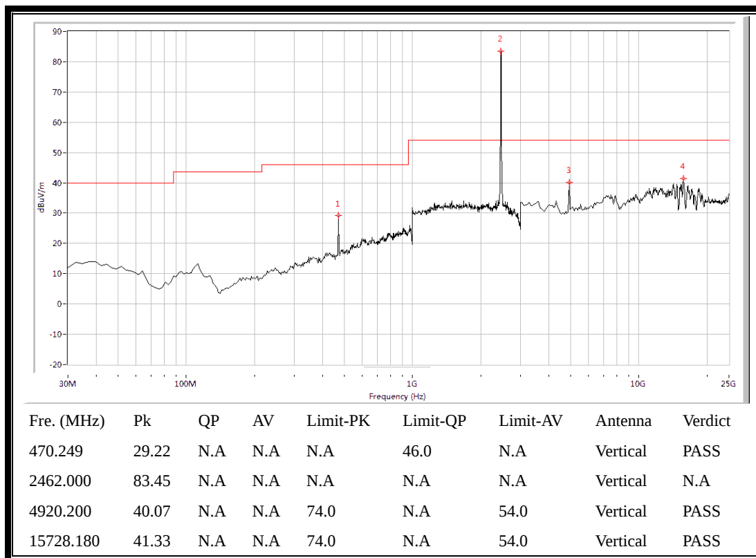
(Plot I.3: Antenna Vertical, 30MHz to 25GHz)
