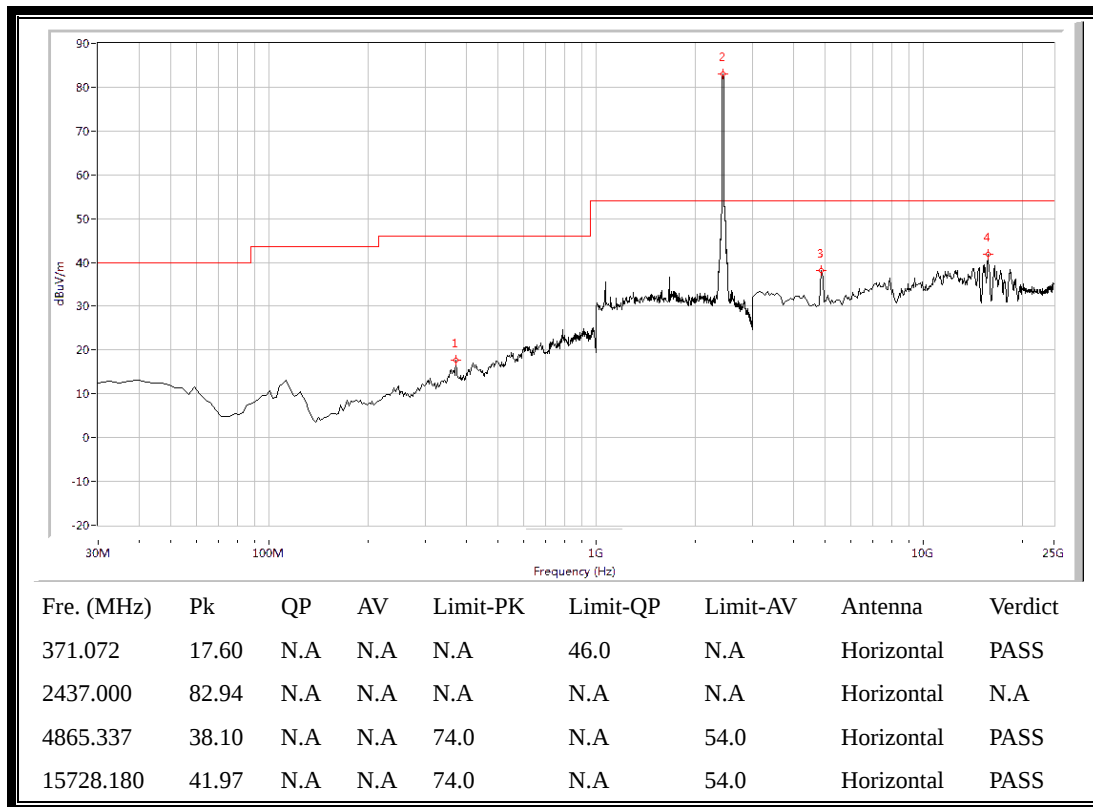
(Plot B.2: Antenna Horizontal, 30MHz to 25GHz)
