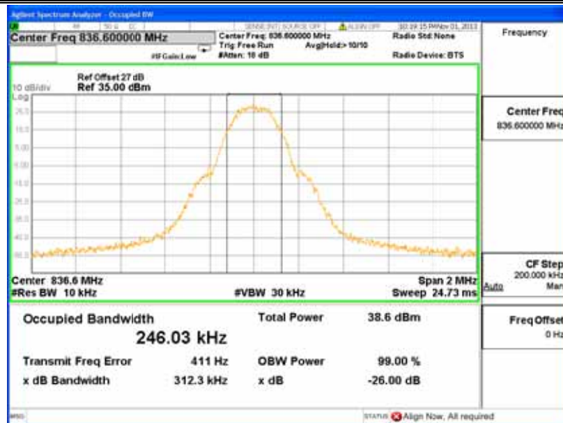
(Plot Z: GPRS 850MHz Channel = 190)
