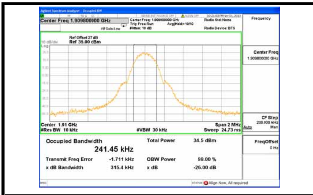
(Plot D1: GPRS 1900MHz Channel = 810)
