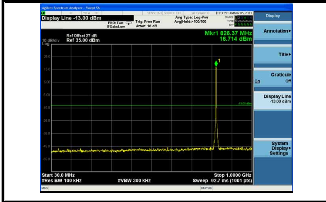
(Plot F 1: HSDPA 850MHz Channel = 4132, 30MHz to 1GHz)
