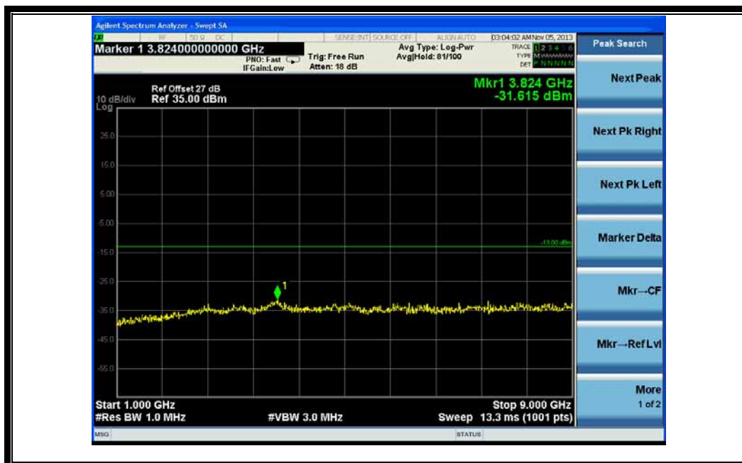
(Plot E3.1: WCDMA850MHz Channel = 4233, 1GHz to 9GHz)
