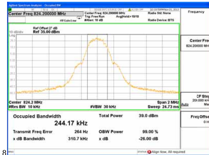
(Plot Y: GPRS 850MHz Channel = 128)
