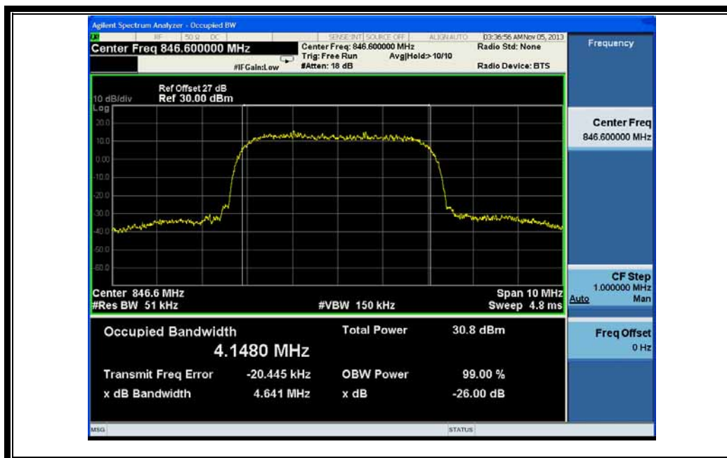
(Plot L: HSDPA 850 MHz Channel = 4233)
