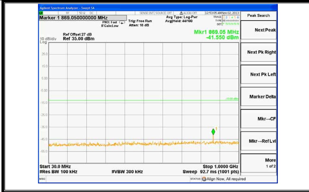
(Plot D1: EDGE 1900MHz Channel = 512, 30MHz to 1GHz)
