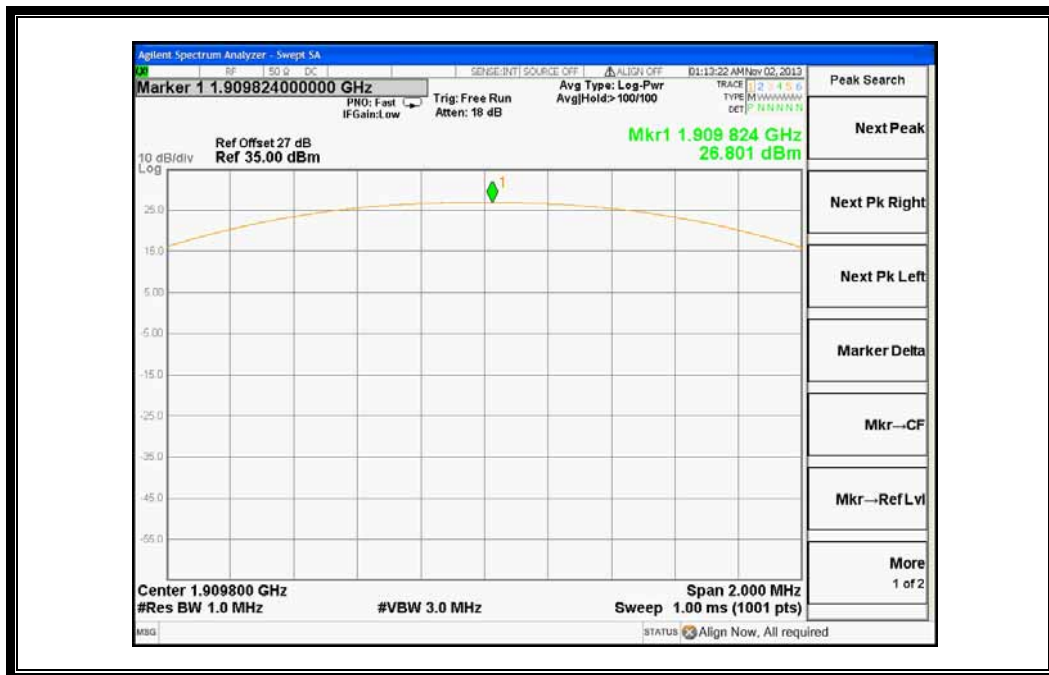
(Plot F3:EGPRS 1900Hz Channel = 810)
