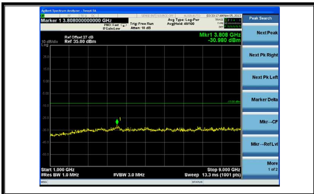
(Plot F3.1: HSDPA850MHz Channel = 4233, 1GHz to 9GHz)
