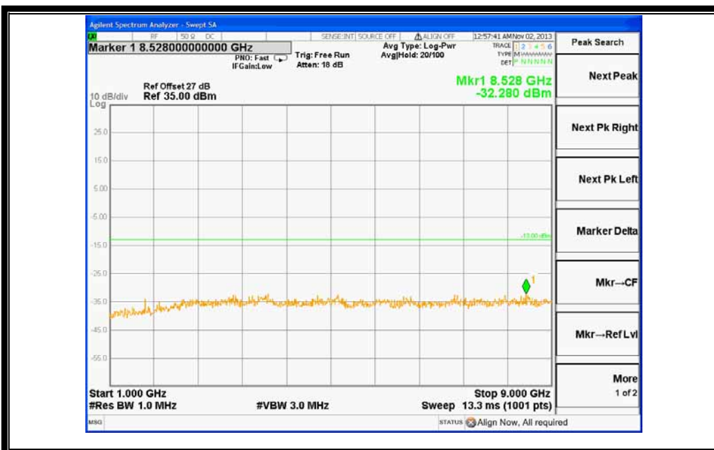
(Plot C1.1: EDGE 850MHz Channel = 128, 1GHz to 9GHz)
