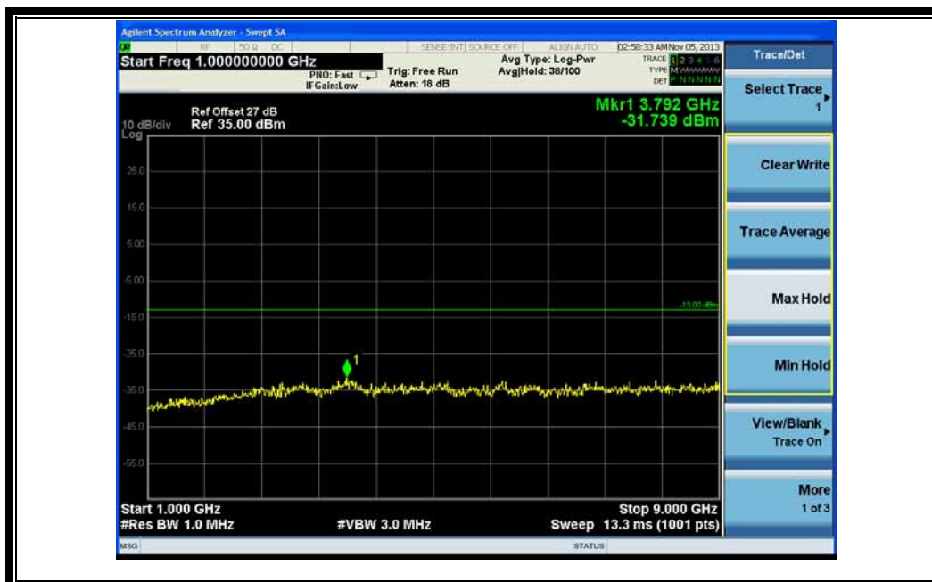
(Plot E1.1: WCDMA850MHz Channel = 4132, 1GHz to 9GHz)
