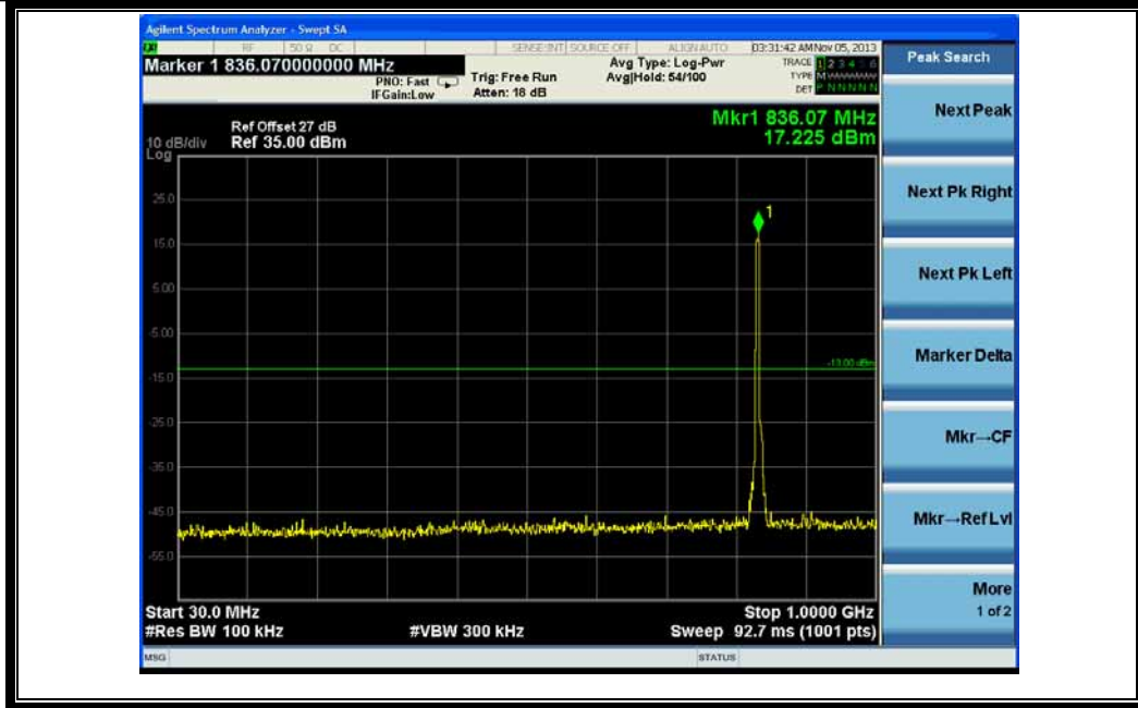
(Plot F 2: HSDPA 850MHz Channel = 4175, 30MHz to 1GHz)
