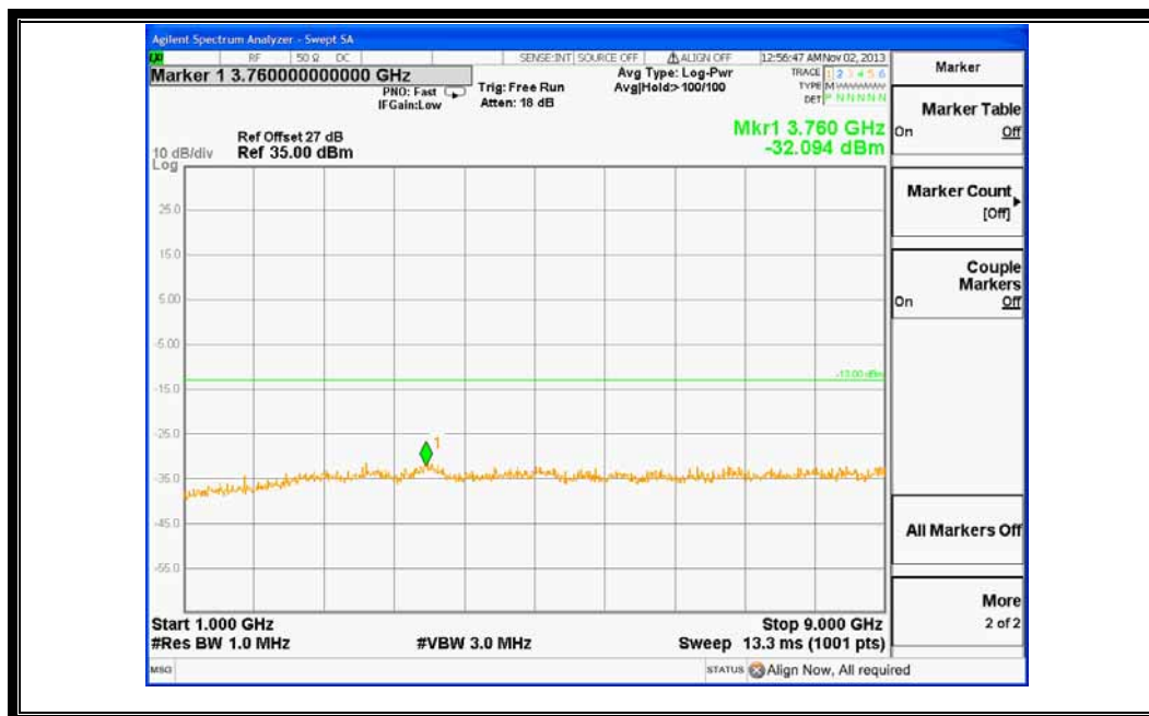
(Plot C3.1: EDGE 850MHz Channel = 251, 1GHz to 9GHz)
