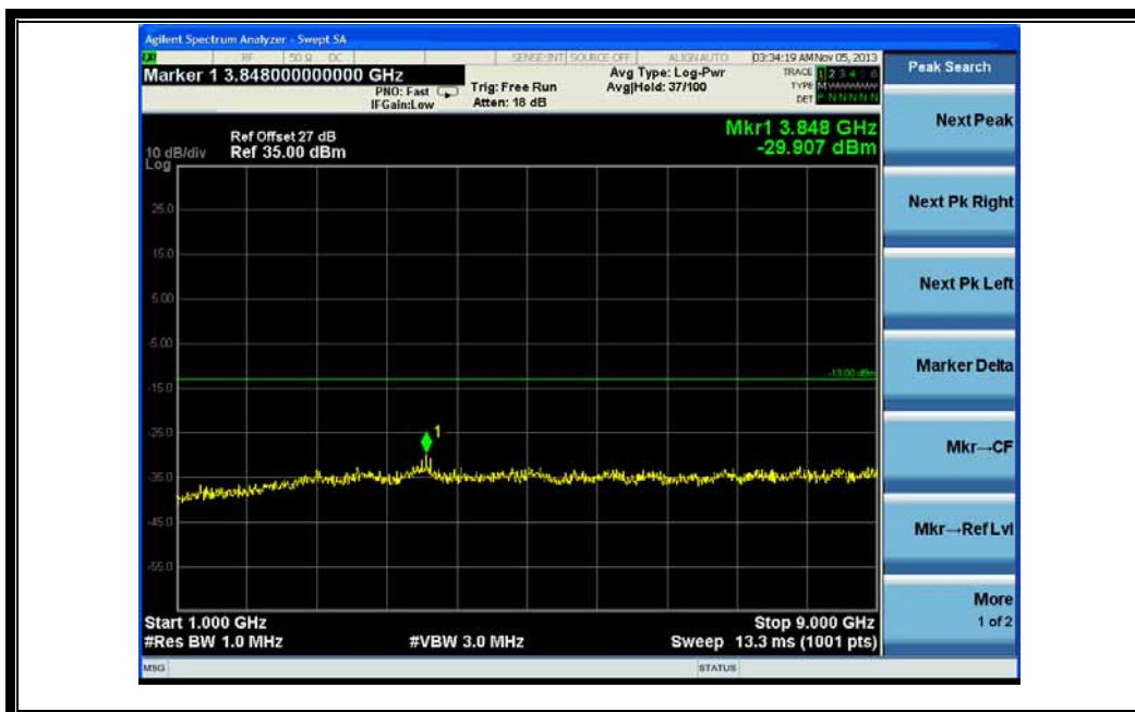
(Plot F1.1: HSDPA 850MHz Channel = 4132, 1GHz to 9GHz)
