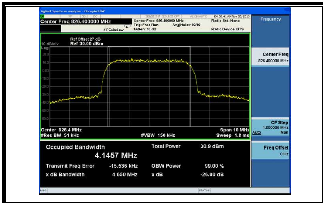
(Plot P: HSPA+ 850 MHz Channel = 4132)
