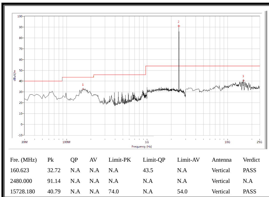
(Plot C.2: 30MHz to 25GHz, Antenna Vertical @ 1/4-DQPSK, channel 78)
