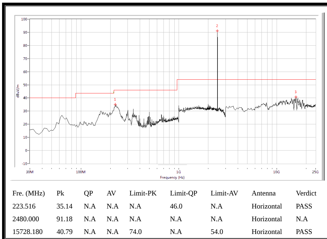
(Plot C.1: 30MHz to 25GHz, Antenna Horizontal @ 1/4-DQPSK, channel 78)
