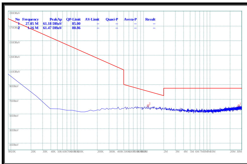
(Plot A.0: 9kHz to 30MHz @ \pi/4 -DQPSK, channel 0)
