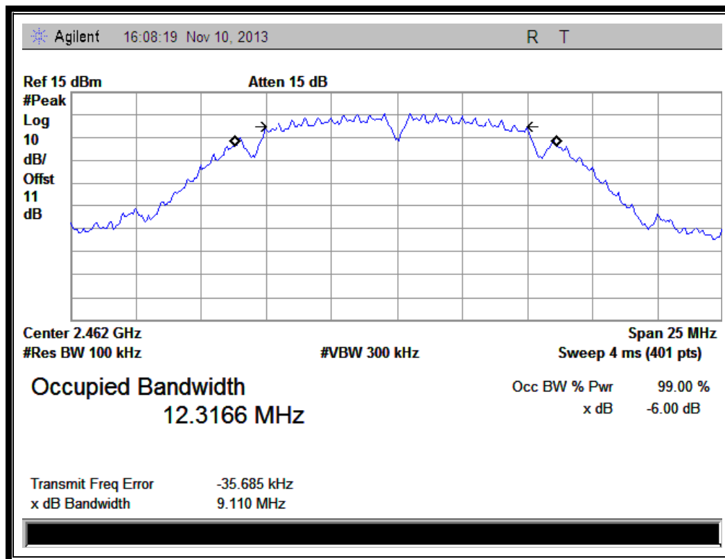
(Plot C: Channel 11: 2462MHz @ 802.11b)
