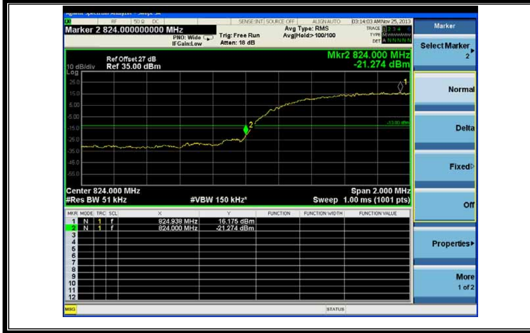
(Plot O: HSPA+ 850 Channel = 4132)
