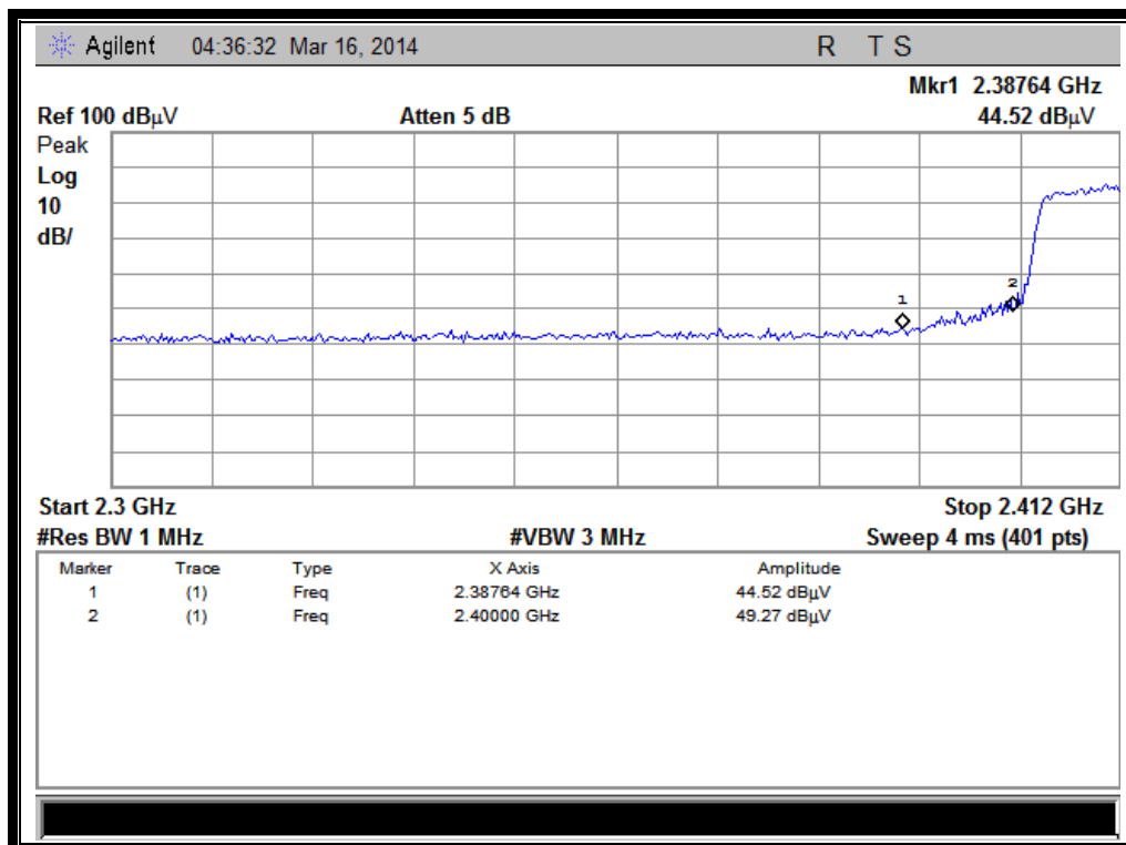
(Plot E1: Channel = 1 PEAK @ 802.11n-20MHz)
