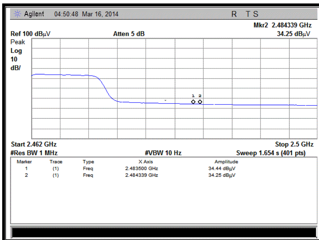
(Plot F2: Channel = 11 AVG @ 802.11n-20MHz)
