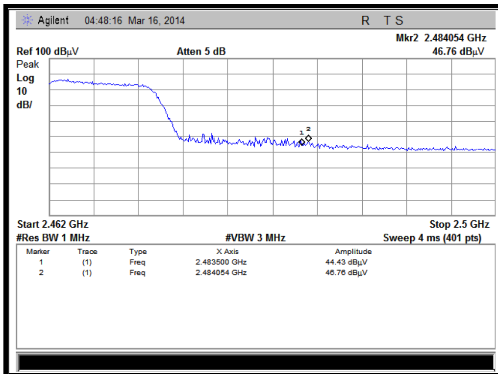
(Plot F1: Channel = 11 PEAK @ 802.11n-20MHz)
