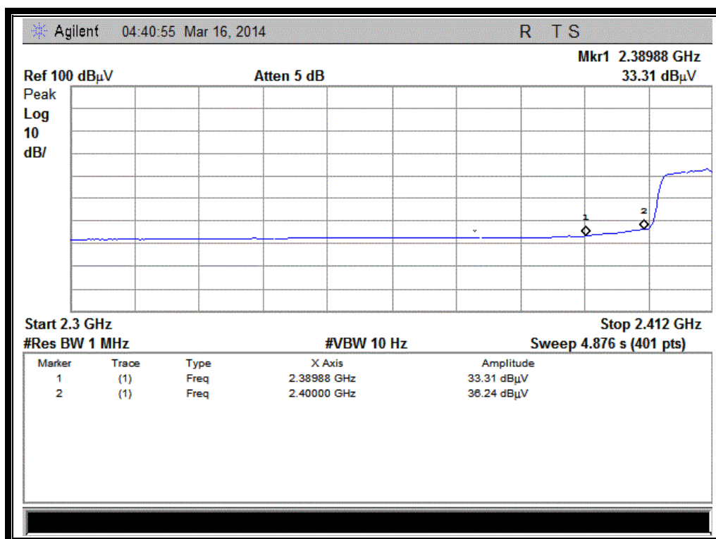
(Plot E2: Channel = 1 AVG @ 802.11n-20MHz)
