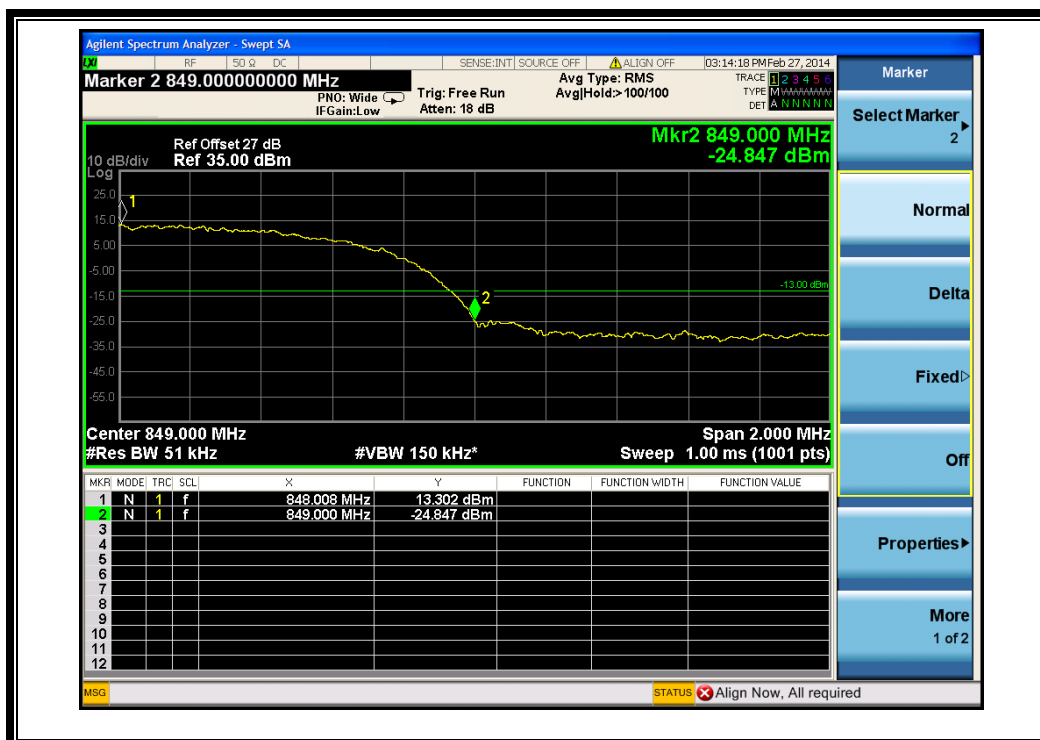
(Plot P: HSPA+ 850 Channel = 4233)
