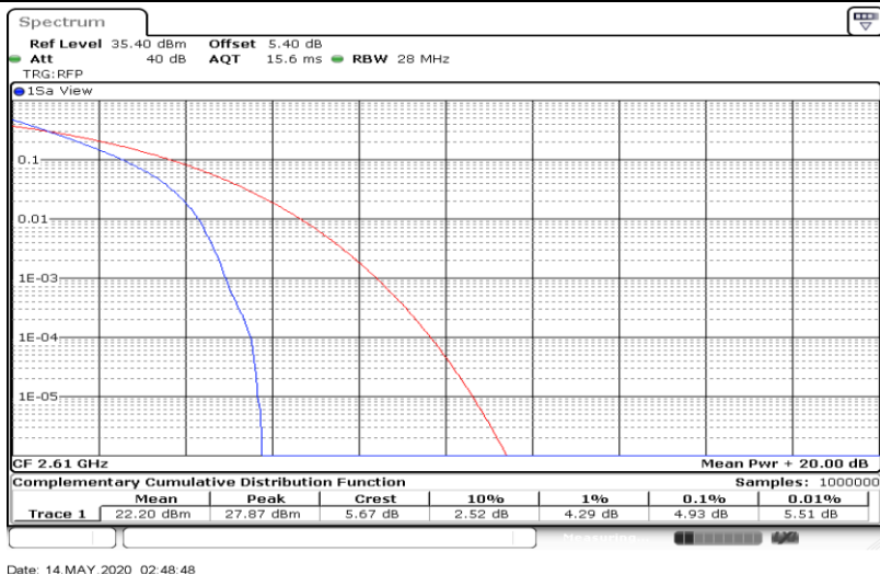
Band38-20MHz-16QAM-37850-27RB#0
