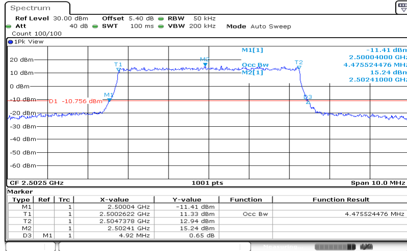
Band7-5MHz-QPSK-20775-25RB#0-4.476
