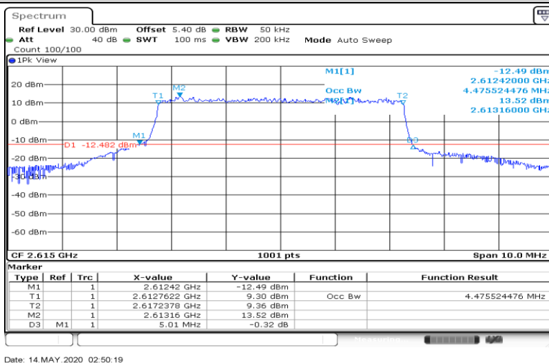
Band41-5MHz-QPSK-40840-25RB#0-4.476
