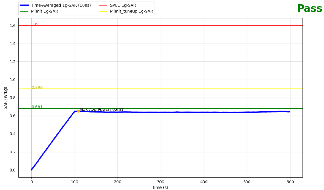
Figure 6-19 Time-averaged SAR measurement for BT TA-SAR test scenario 1-1
