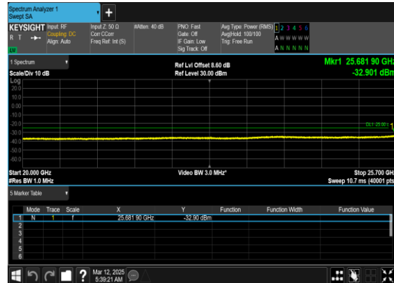
N7(40M)_DFT-s- OFDM_BPSK_Edge_1RB_Left_High_CH
