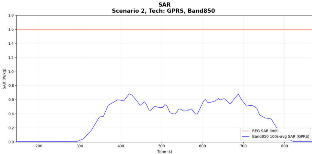
Figure 7-3 Time-averaged SAR
