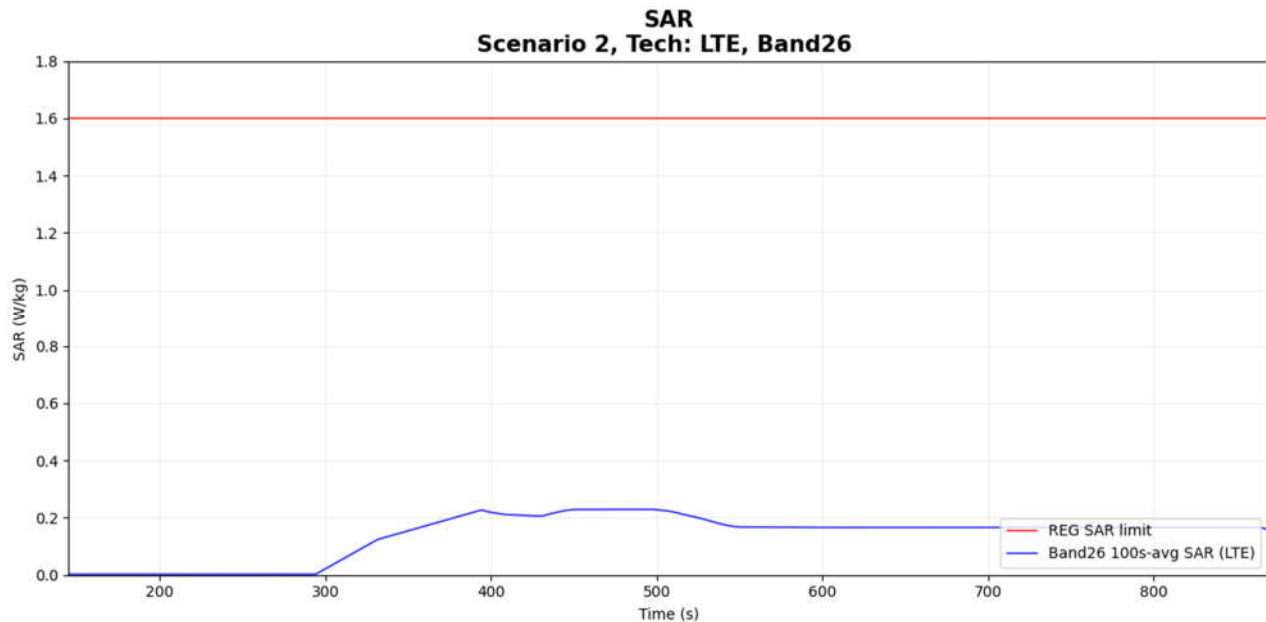
Figure 7-10 Time-averaged SAR
