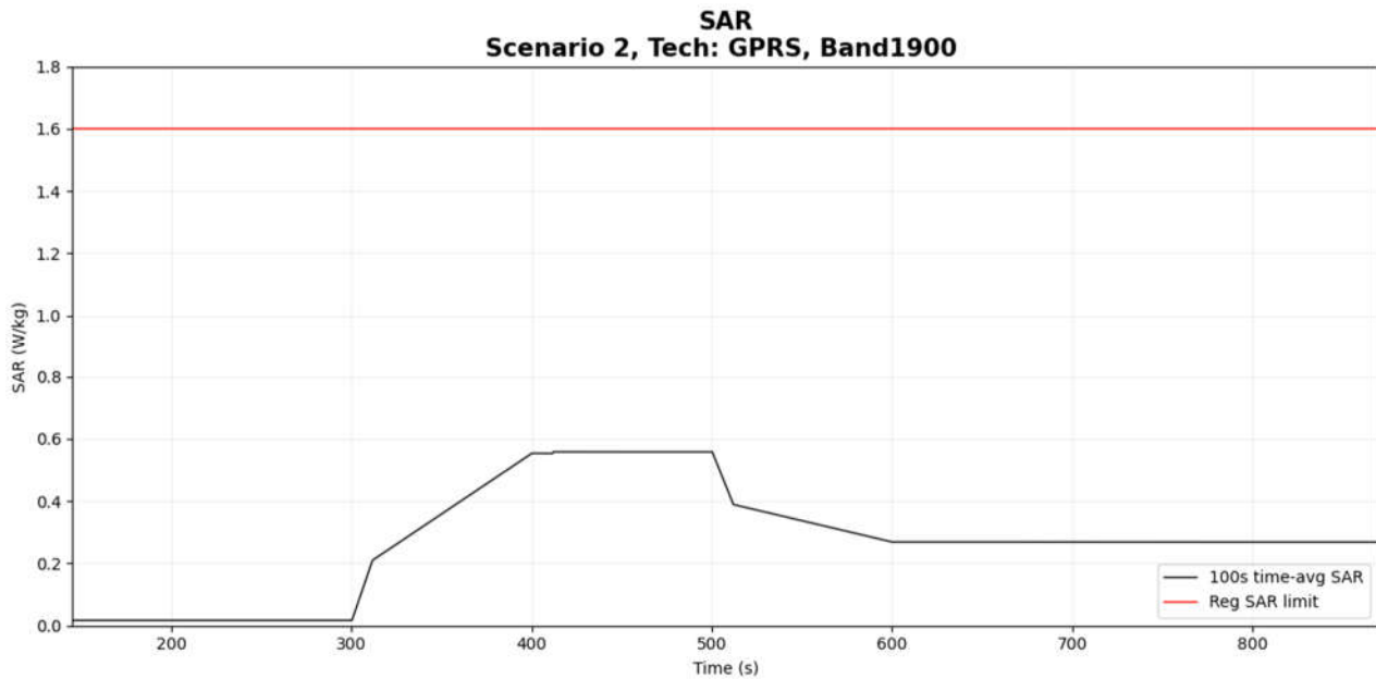
Figure 6- 7 Time-averaged SAR
