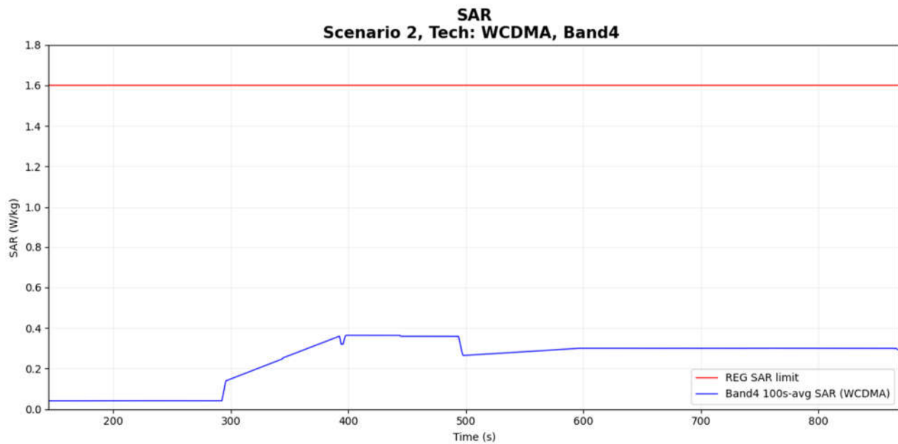
Figure 7-8 Time-averaged SAR
