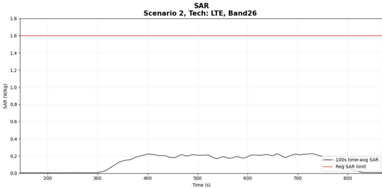
Figure 6- 14 Time-averaged SAR
