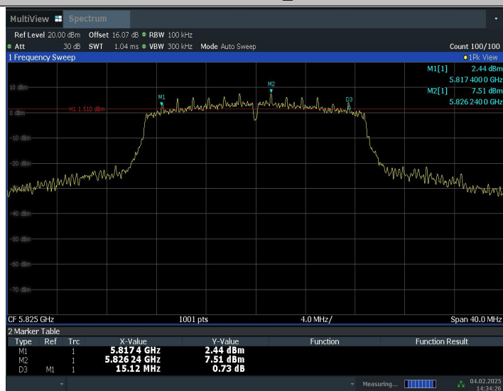
11AC20SISO_5825
