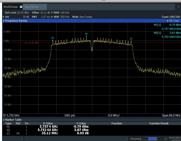
11AC40SISO_5755
