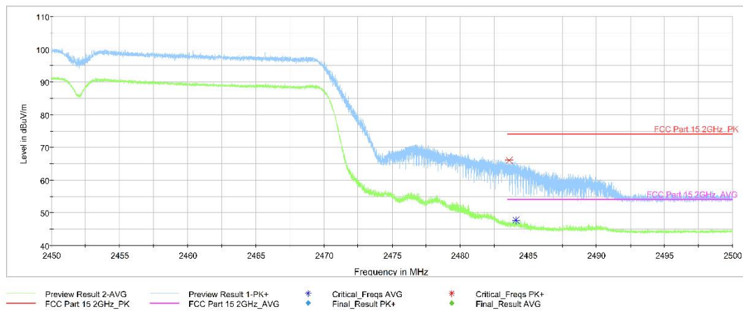
Fig.8 Transmitter Spurious Emission - Radiated (Power): 802.11n-HT40, ch9, 2.45 GHz - 2.50GHz
