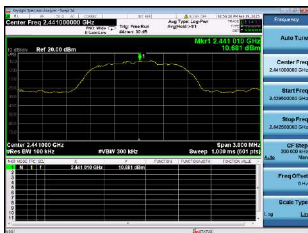
8-DPSK MIDDLE CHANNEL, CARRIER LEVEL
