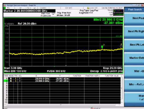
8-DPSK LOW CHANNEL, SPURIOUS 3 GHz ~ 25 GHz
