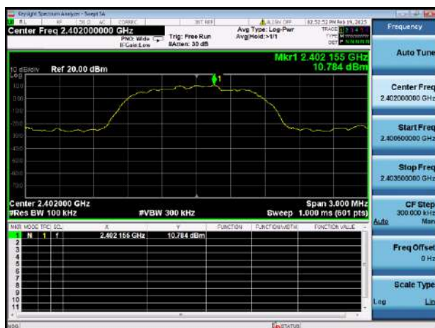
8-DPSK LOW CHANNEL, CARRIER LEVEL
