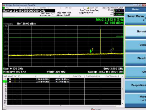
8-DPSK LOW CHANNEL, SPURIOUS 30 MHz ~ 3 GHz
