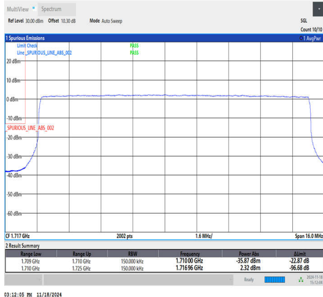
Band66_15MHz_64QAM_132047_75RB#0
