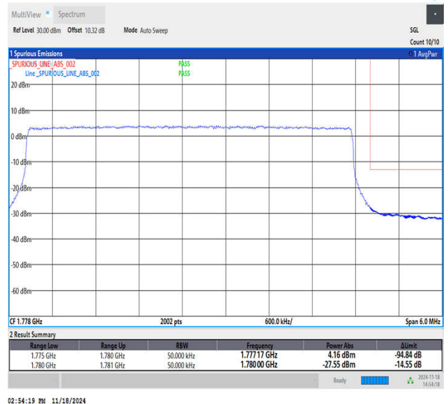
Band66_5MHz_16QAM_132647_25RB#0
