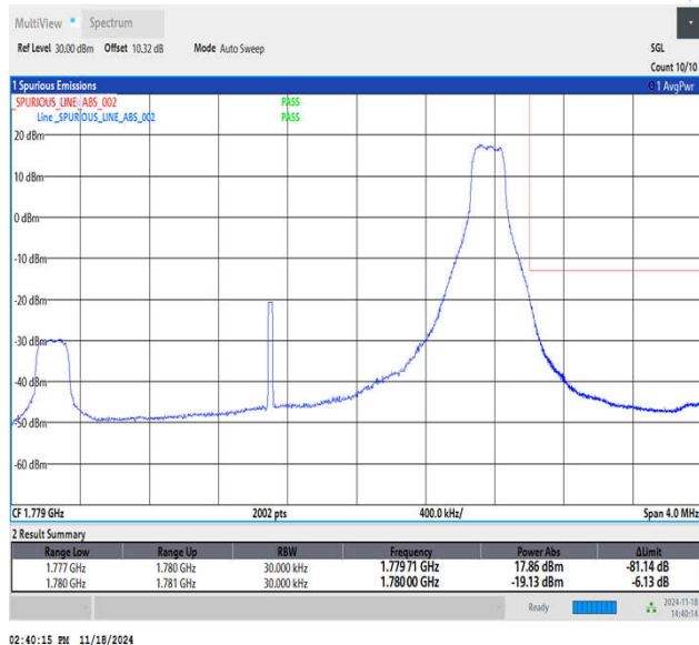
Band66_3MHz_QPSK_132657_1RB#14
