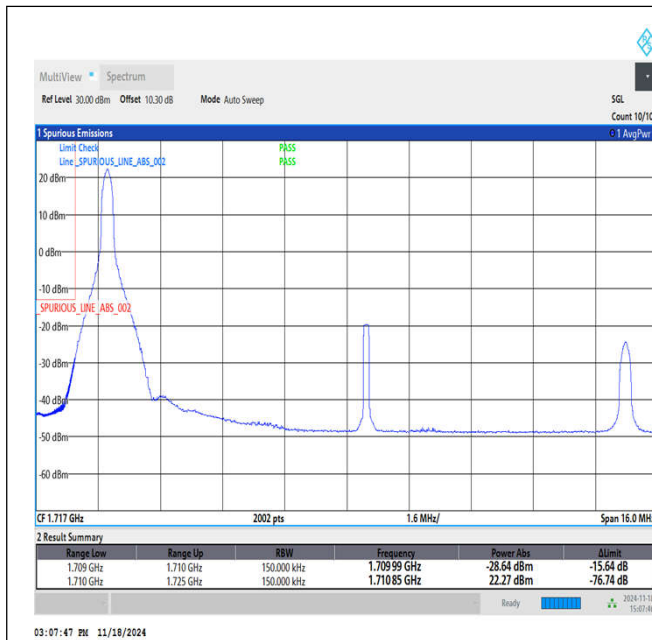
Band66_15MHz_16QAM_132047_1RB#0
