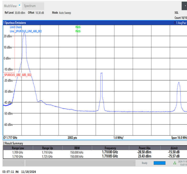
Band66_15MHz_QPSK_132047_1RB#0
