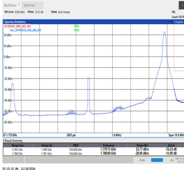
Band66_15MHz_16QAM_132597_1RB#74
