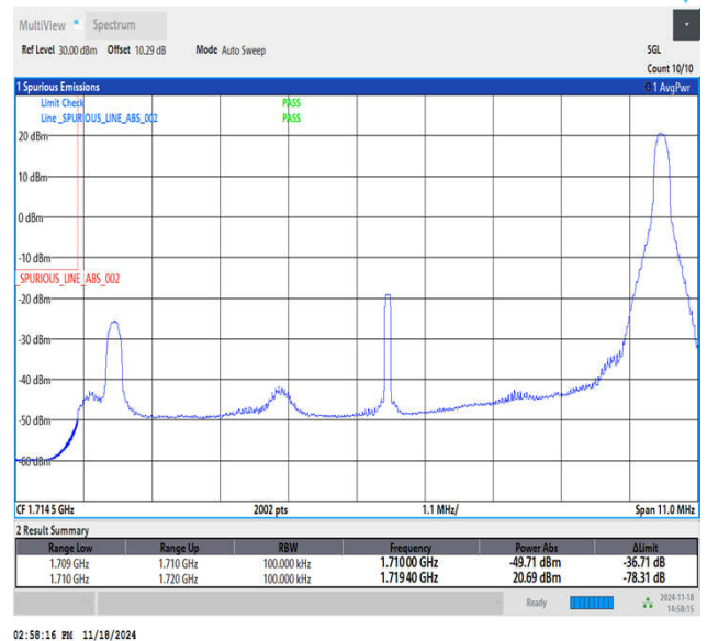
Band66_10MHz_16QAM_132022_1RB#49
