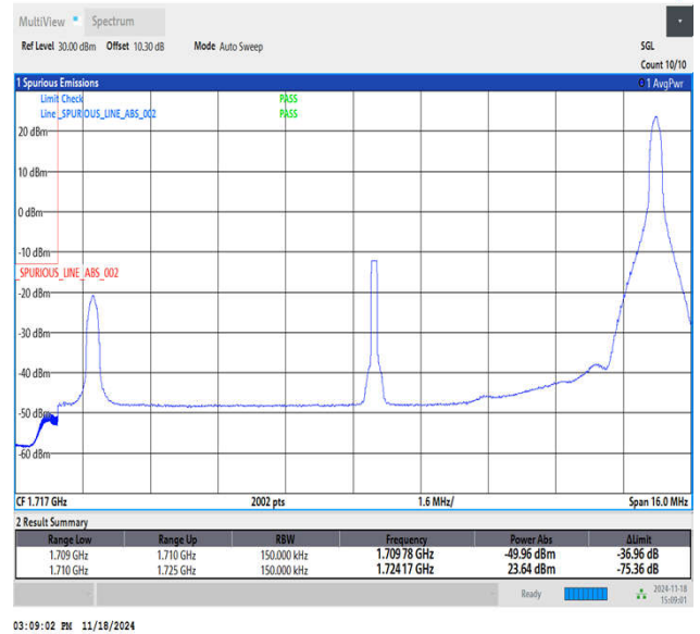
Band66_15MHz_QPSK_132047_1RB#74
