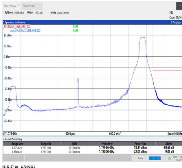
Band66_5MHz_16QAM_132647_1RB#24
