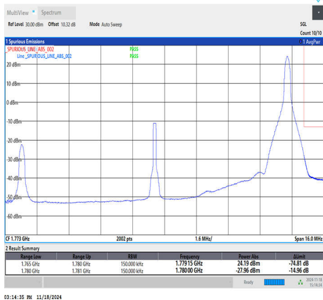
Band66_15MHz_QPSK_132597_1RB#74
