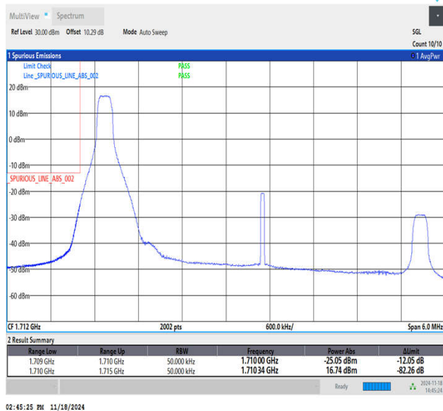
Band66_5MHz_64QAM_131997_1RB#0
