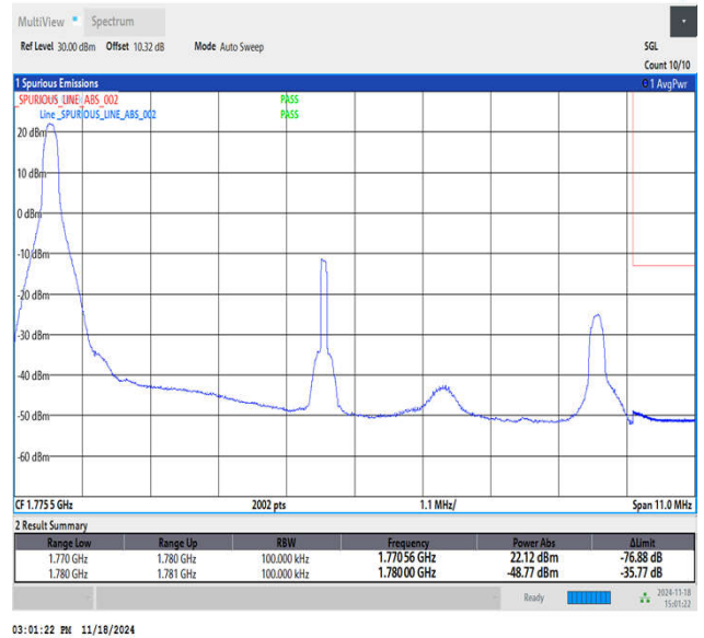
Band66_10MHz_QPSK_132622_1RB#0
