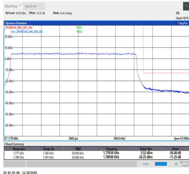
Band66_3MHz_QPSK_132657_15RB#0
