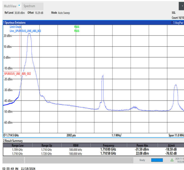
Band66_10MHz_QPSK_132022_1RB#0
