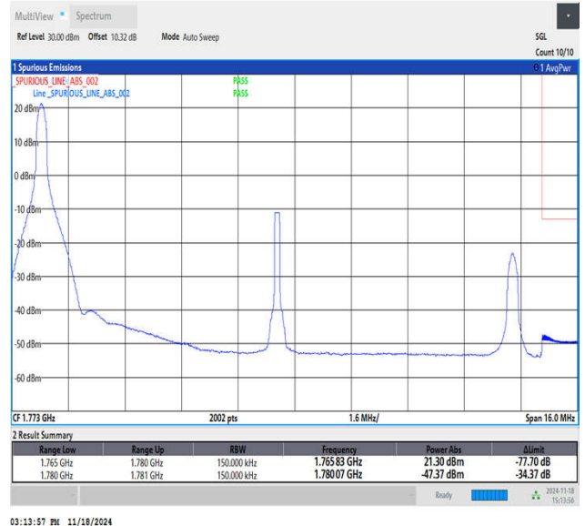
Band66_15MHz_64QAM_132597_1RB#0
