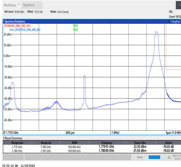
Band66_10MHz_QPSK_132622_1RB#49
