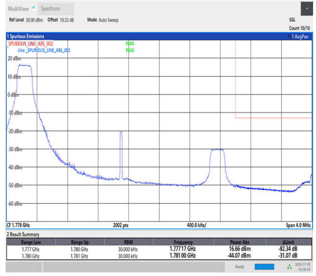
Band66_3MHz_16QAM_132657_1RB#0
