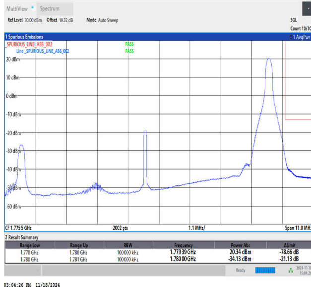
Band66_10MHz_64QAM_132622_1RB#49
