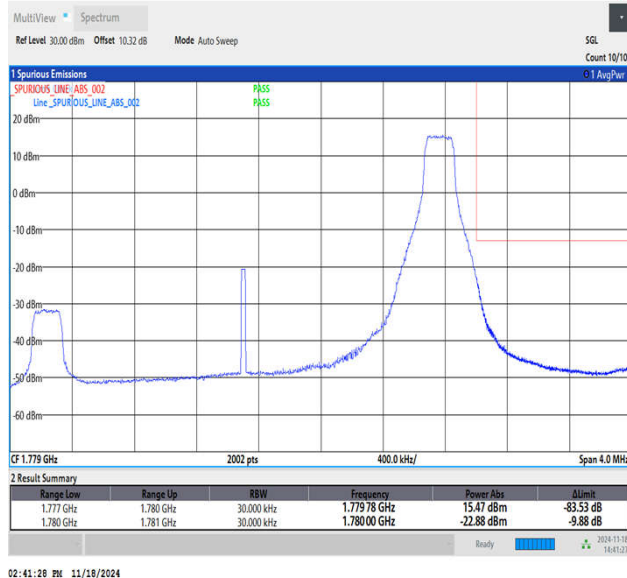
Band66_3MHz_64QAM_132657_1RB#14
