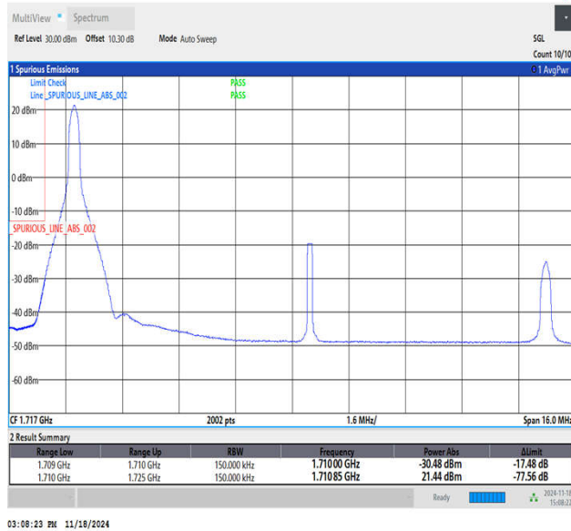
Band66_15MHz_64QAM_132047_1RB#0
