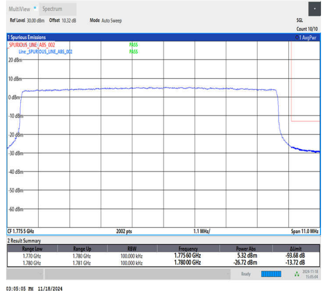
Band66_10MHz_QPSK_132622_50RB#0
