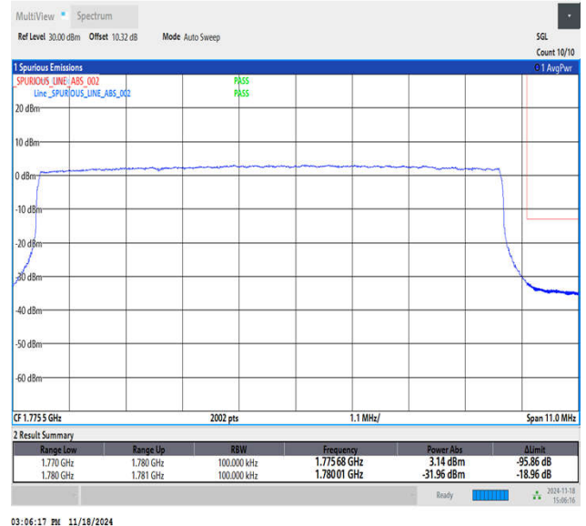
Band66_10MHz_64QAM_132622_50RB#0
