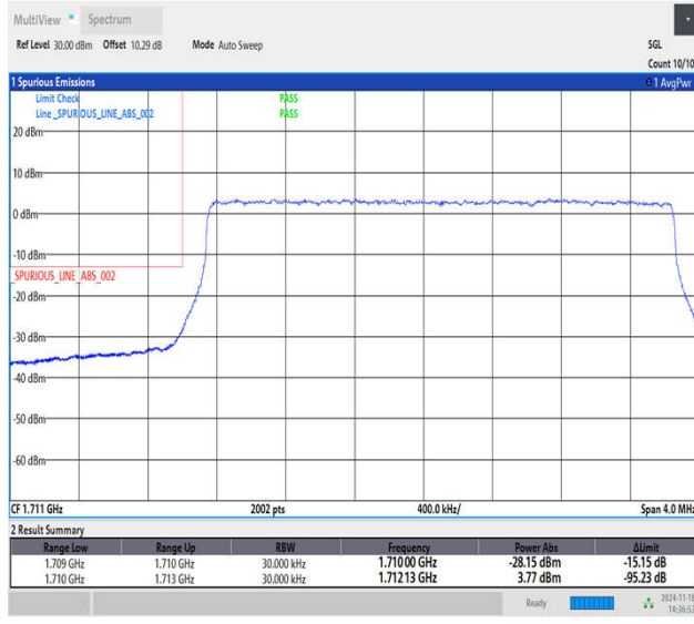
Band66_3MHz_16QAM_131987_15RB#0
