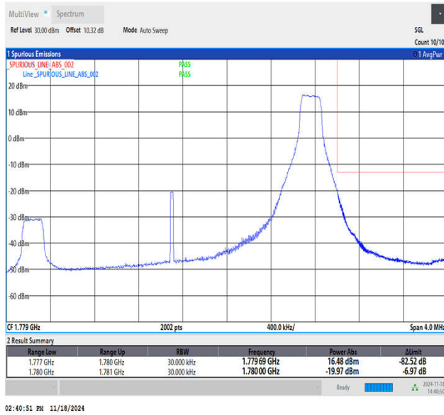
Band66_3MHz_16QAM_132657_1RB#14
