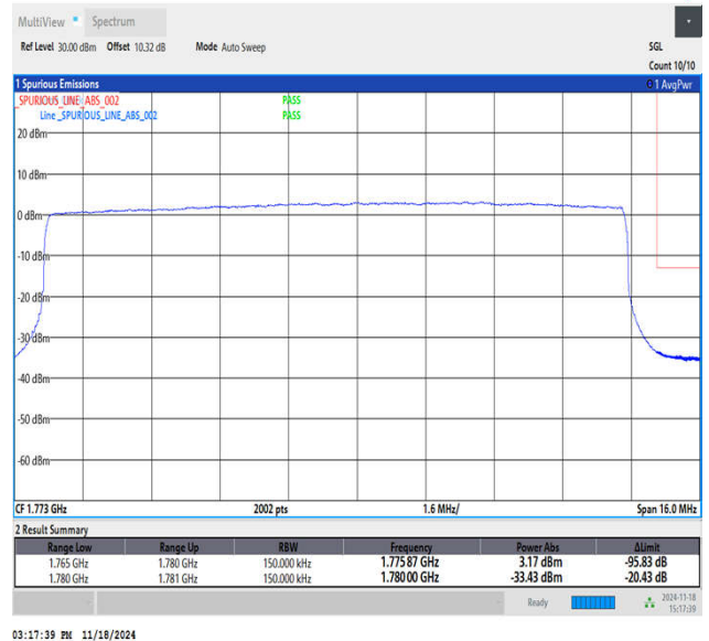
Band66_15MHz_64QAM_132597_75RB#0
