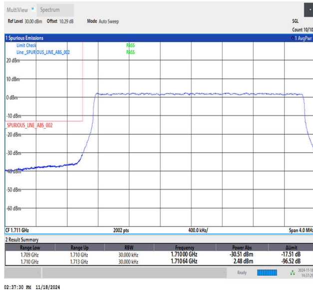
Band66_3MHz_64QAM_131987_15RB#0
