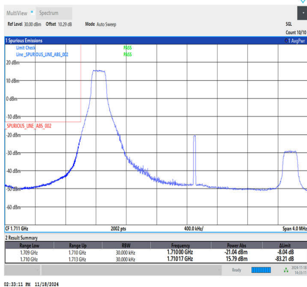
Band66_3MHz_16QAM_131987_1RB#0
