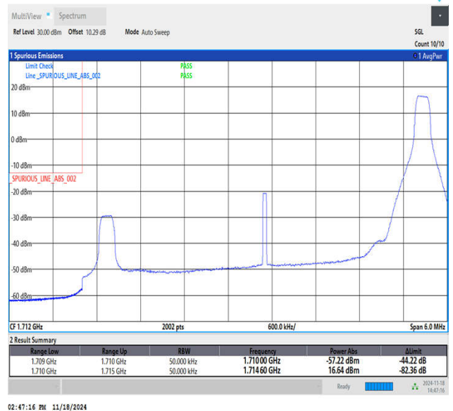
Band66_5MHz_64QAM_131997_1RB#24
