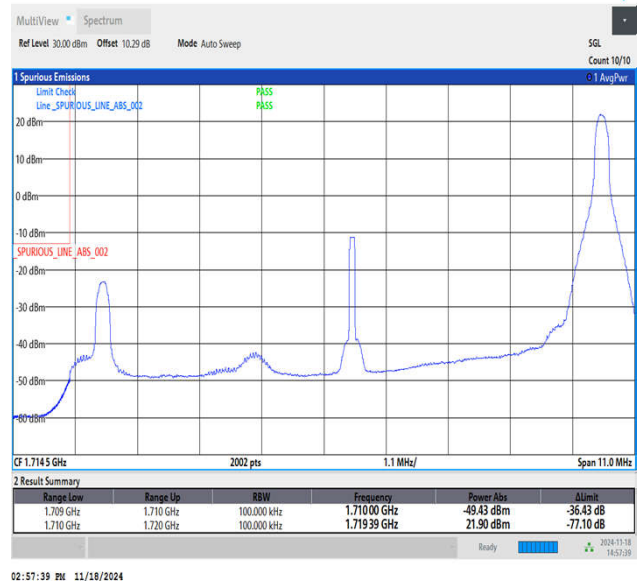
Band66_10MHz_QPSK_132022_1RB#49
