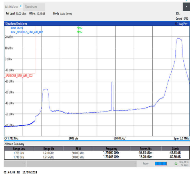
Band66_5MHz_QPSK_131997_1RB#24
