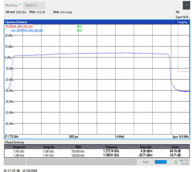
Band66_15MHz_16QAM_132597_75RB#0
