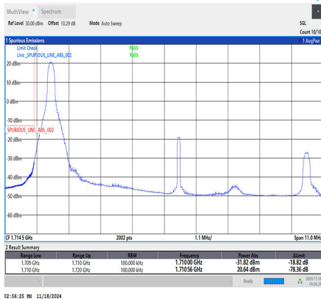
Band66_10MHz_16QAM_132022_1RB#0
