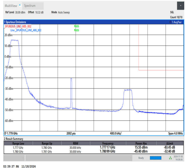
Band66_3MHz_64QAM_132657_1RB#0
