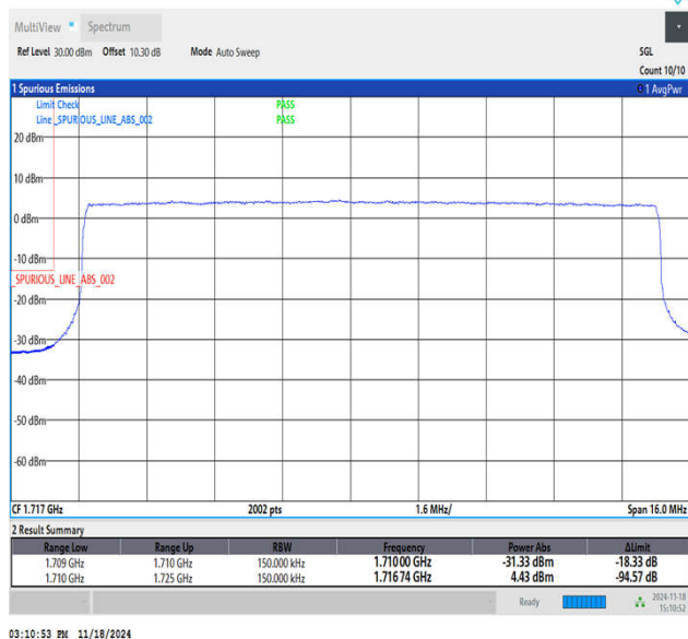
Band66_15MHz_QPSK_132047_75RB#0
