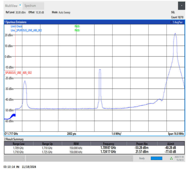
Band66_15MHz_64QAM_132047_1RB#74
