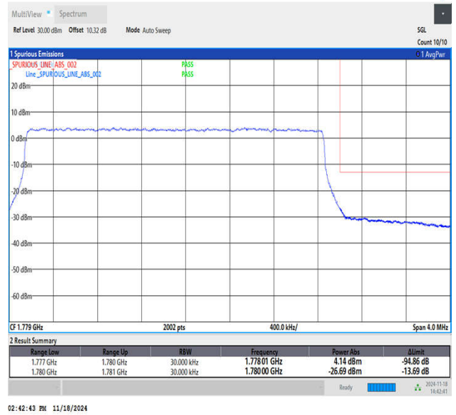
Band66_3MHz_16QAM_132657_15RB#0
