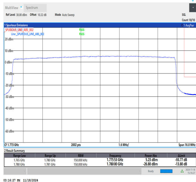
Band66_15MHz_QPSK_132597_75RB#0
