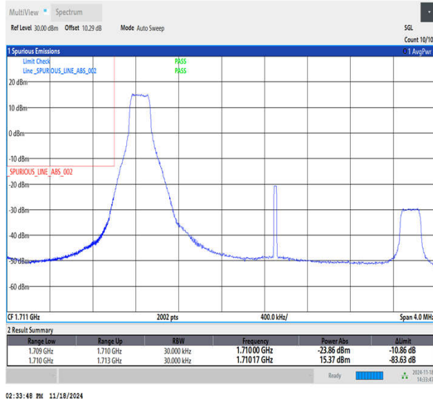
Band66_3MHz_64QAM_131987_1RB#0
