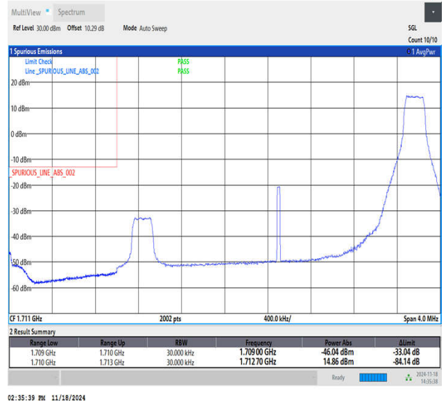
Band66_3MHz_64QAM_131987_1RB#14
