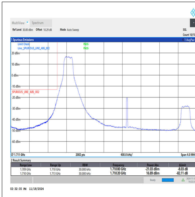
Band66_3MHz_QPSK_131987_1RB#0
