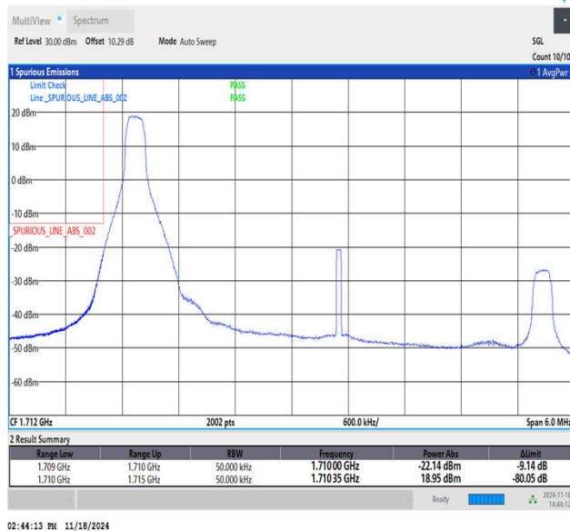
Band66_5MHz_QPSK_131997_1RB#0
