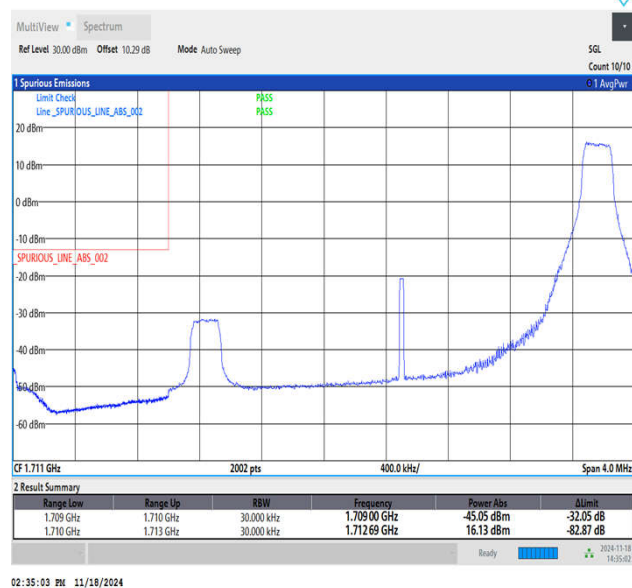
Band66_3MHz_16QAM_131987_1RB#14
