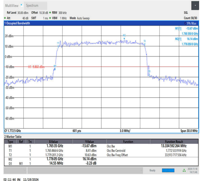
Band66-15MHz-16QAM-132597-75RB#0-PASS
