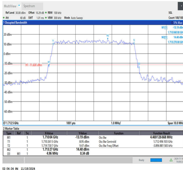
Band66-5MHz-64QAM-131997-25RB#0-PASS
