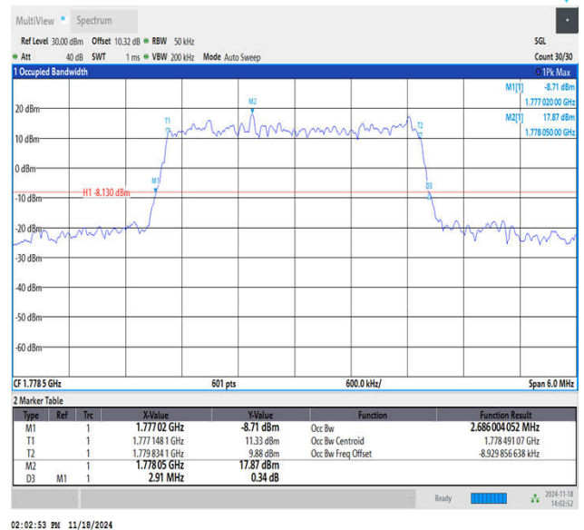
Band66-3MHz-QPSK-132657-15RB#0-PASS
