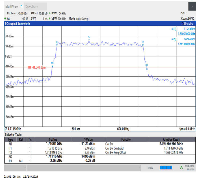
Band66-3MHz-QPSK-131987-15RB#0-PASS
