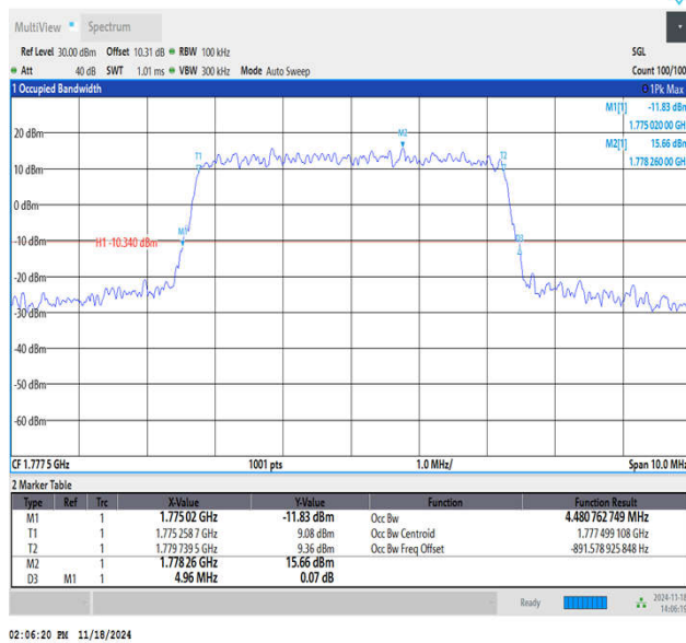
Band66-5MHz-64QAM-132647-25RB#0-PASS
