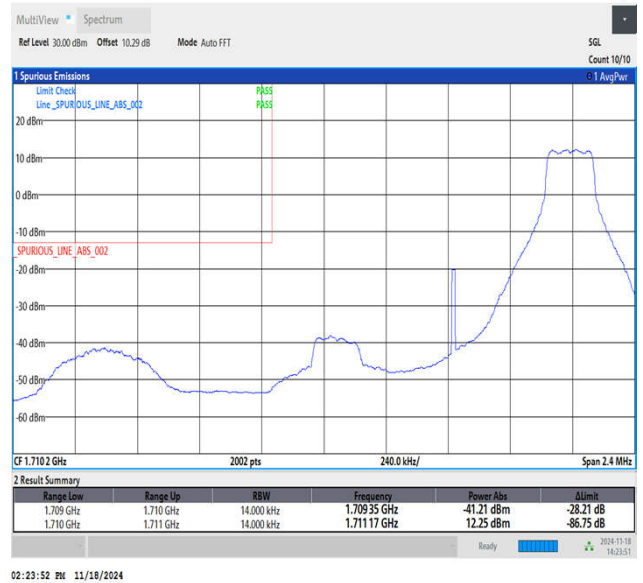
Band66_1.4MHz_64QAM_131979_1RB#5
