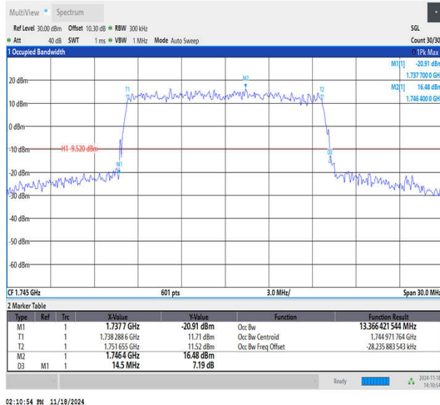
Band66-15MHz-16QAM-132322-75RB#0-PASS
