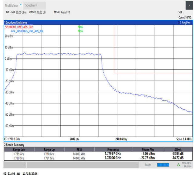
Band66_1.4MHz_16QAM_132665_6RB#0
