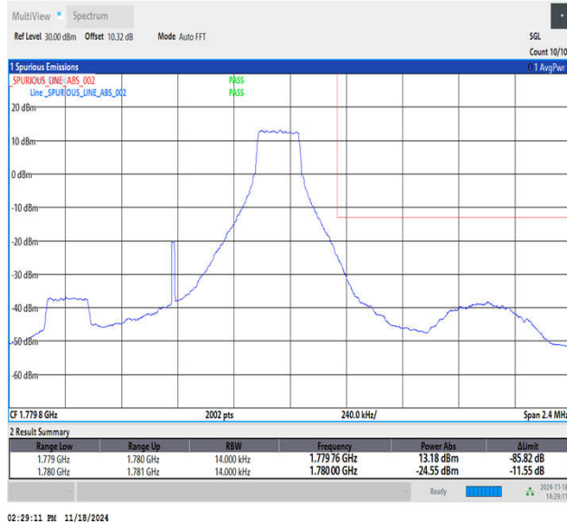
Band66_1.4MHz_16QAM_132665_1RB#5
