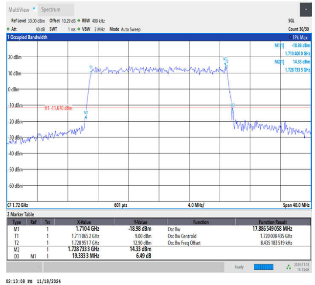
Band66-20MHz-64QAM-132072-100RB#0-PASS
