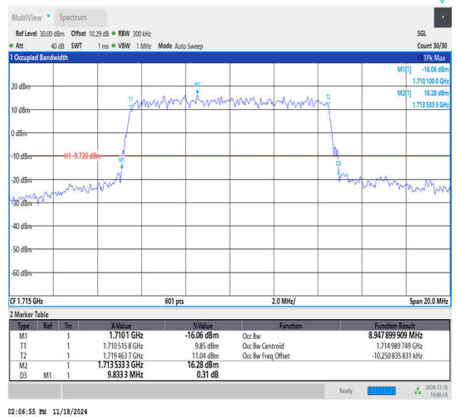
Band66-10MHz-QPSK-132022-50RB#0-PASS
