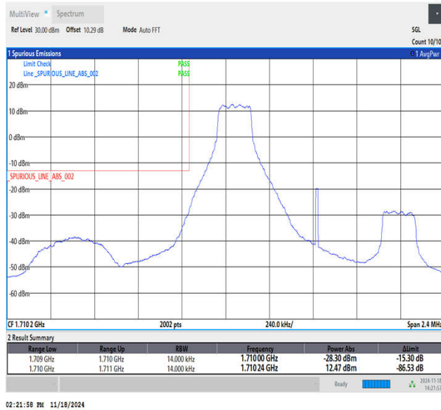
Band66_1.4MHz_64QAM_131979_1RB#0
