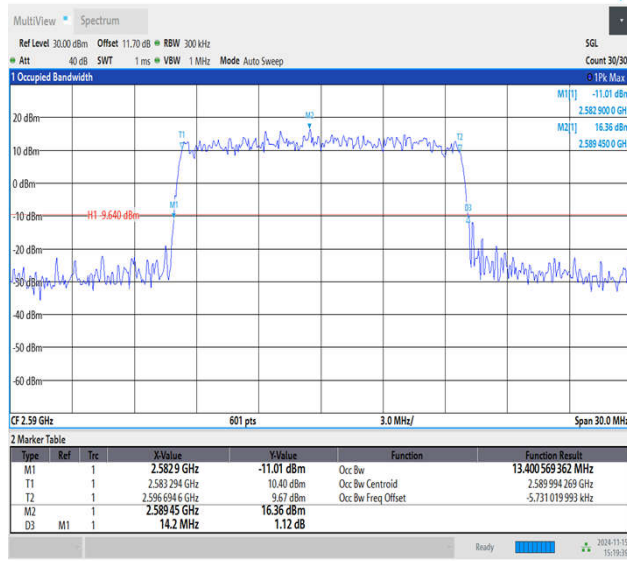
41(2535-2655)-15MHz-16QAM-40590-75RB#0-PASS
