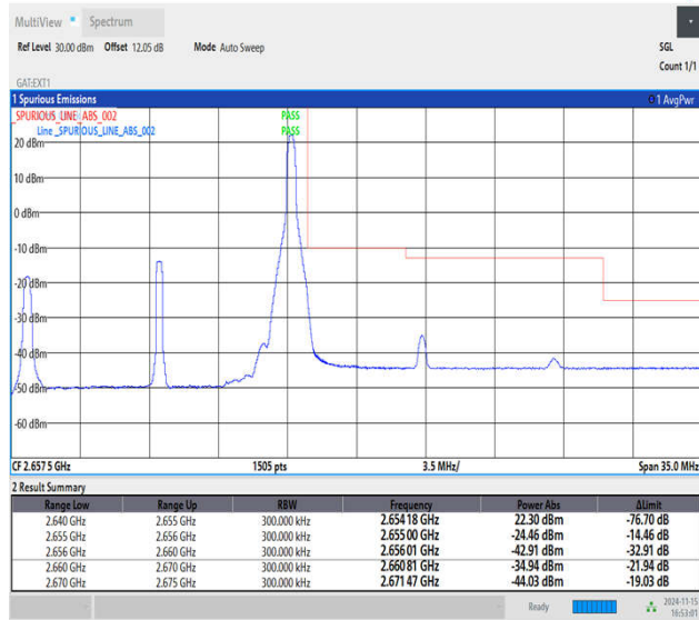
Band41_15MHz_64QAM_41165_1RB#74
