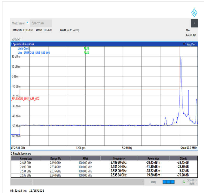
Band41_5MHz_16QAM_40065_1RB#0
