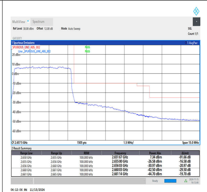
Band41_5MHz_64QAM_41215_1RB#0
