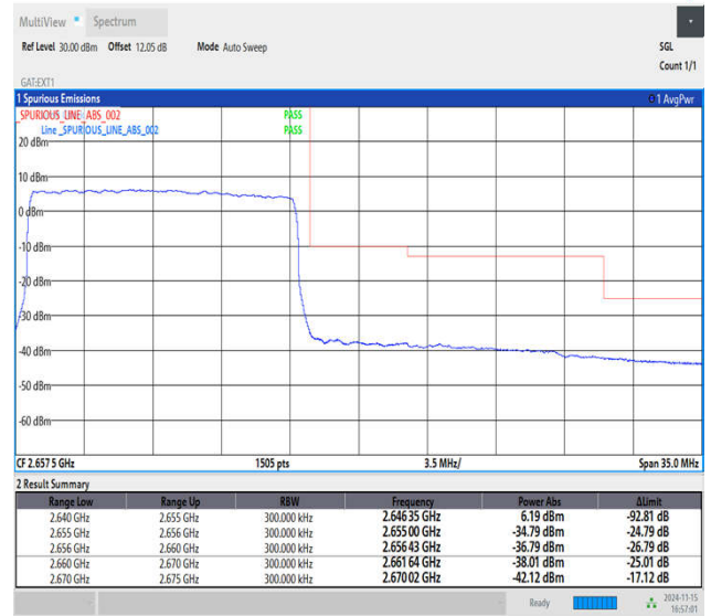
Band41_15MHz_64QAM_41165_75RB#0
