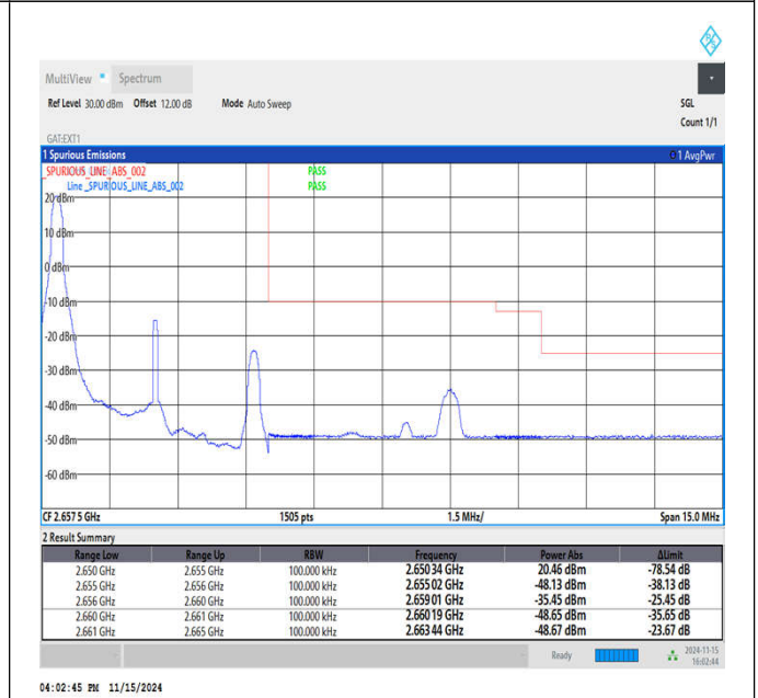
Band41_5MHz_16QAM_41215_1RB#0
