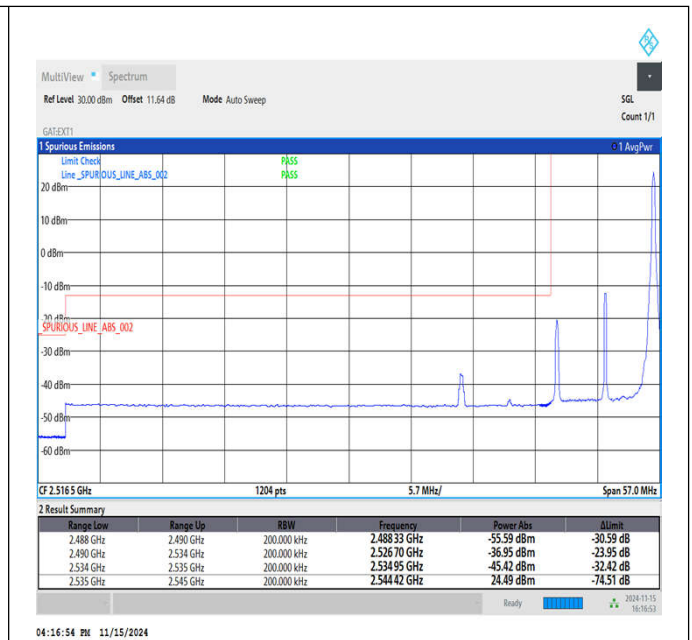
Band41_10MHz_QPSK_40090_1RB#49
