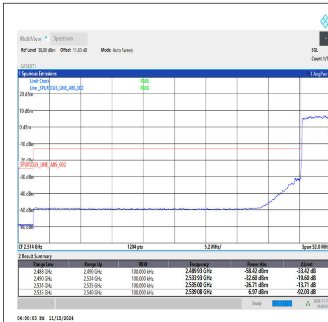
Band41_5MHz_64QAM_40065_25RB#0
