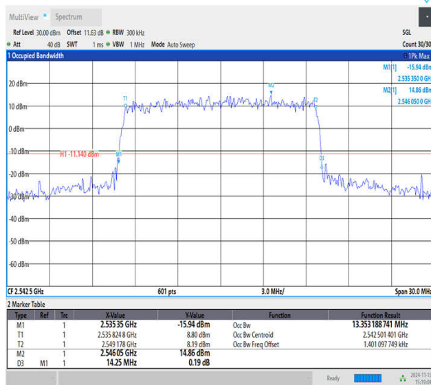
41(2535-2655)-15MHz-64QAM-40115-75RB#0-PASS
