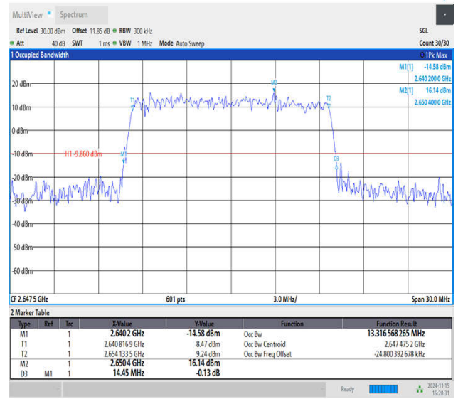
41(2535-2655)-15MHz-16QAM-41165-75RB#0-PASS
