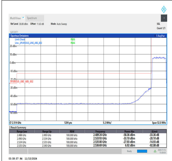
Band41_5MHz_16QAM_40065_25RB#0
