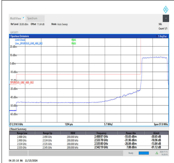
Band41_10MHz_QPSK_40090_50RB#0
