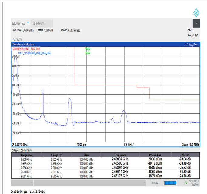
Band41_5MHz_64QAM_41215_1RB#0
