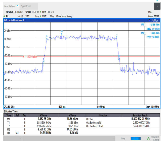
41(2535-2655)-15MHz-64QAM-40590-75RB#0-PASS
