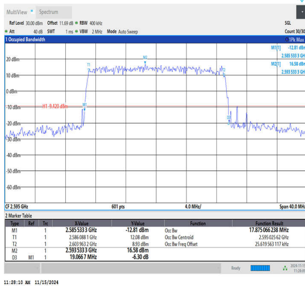
Band38-20MHz-QPSK-38000-100RB#0-PASS
