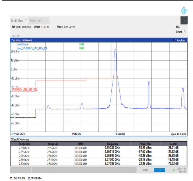
Band38_15MHz_64QAM_37825_1RB#0
