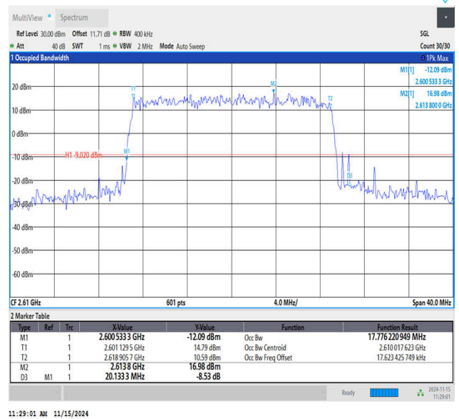
Band38-20MHz-QPSK-38150-100RB#0-PASS
