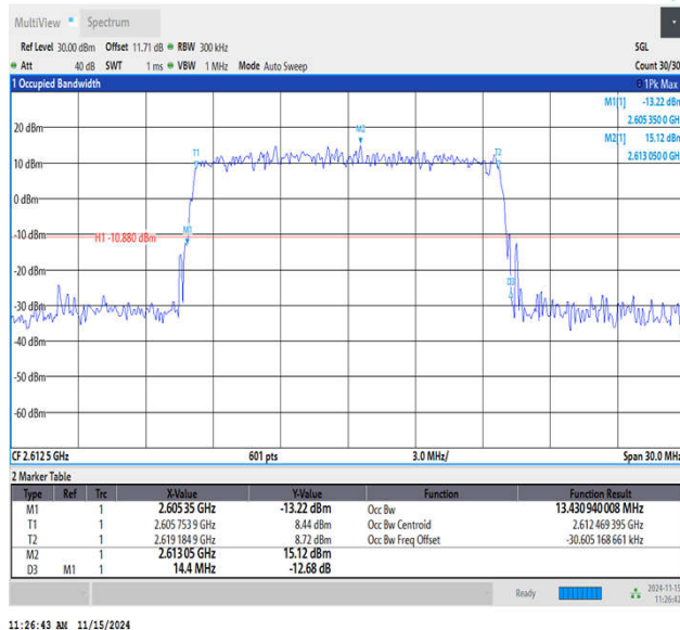
Band38-15MHz-64QAM-38175-75RB#0-PASS
