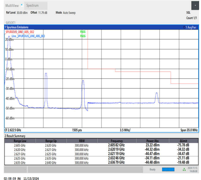
Band38_15MHz_64QAM_38175_1RB#0
