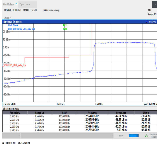
Band38_15MHz_64QAM_37825_75RB#0
