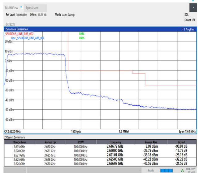
Band38_5MHz_QPSK_38225_25RB#0
