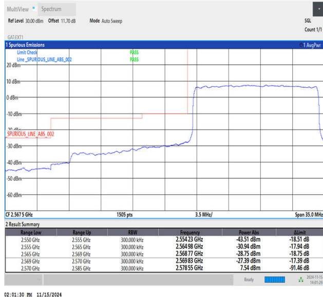
Band38_15MHz_QPSK_37825_75RB#0
