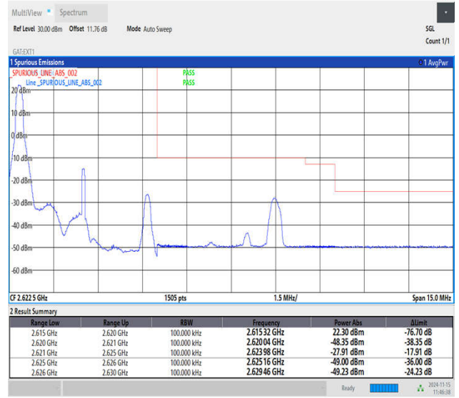
Band38_5MHz_QPSK_38225_1RB#0
