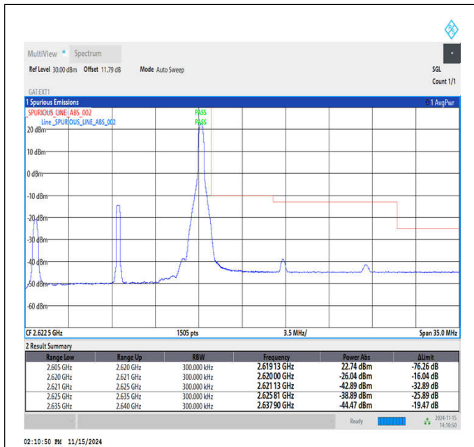
Band38_15MHz_16QAM_38175_1RB#74
