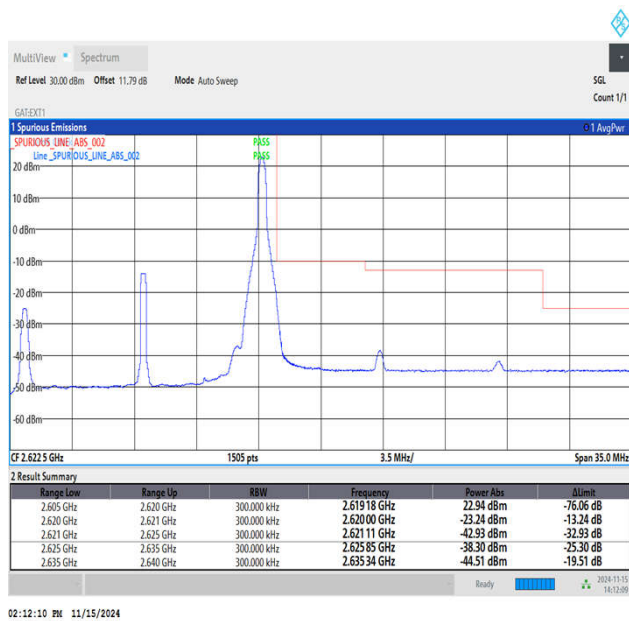
Band38_15MHz_64QAM_38175_1RB#74
