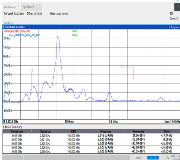
Band38_5MHz_QPSK_38225_1RB#24
