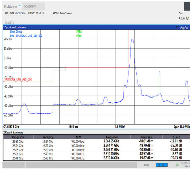
Band38_5MHz_16QAM_37775_1RB#0
