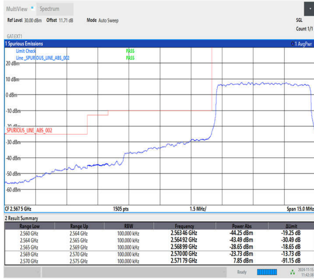
Band38_5MHz_QPSK_37775_25RB#0
