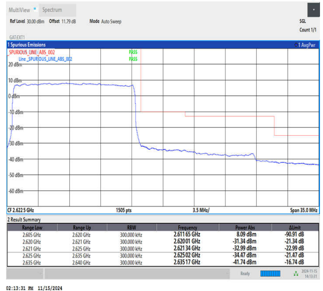
Band38_15MHz_QPSK_38175_75RB#0
