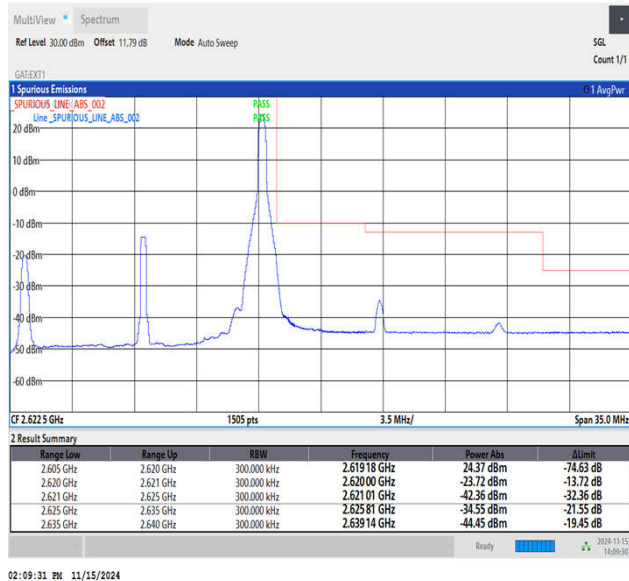
Band38_15MHz_QPSK_38175_1RB#74
