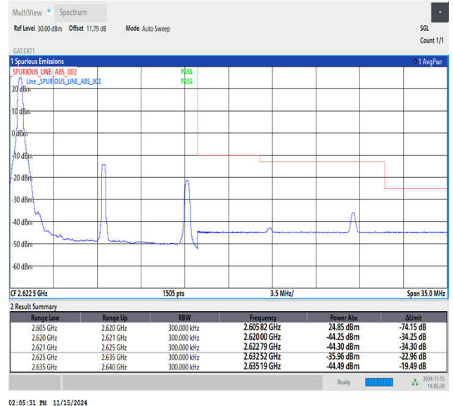
Band38_15MHz_QPSK_38175_1RB#0
