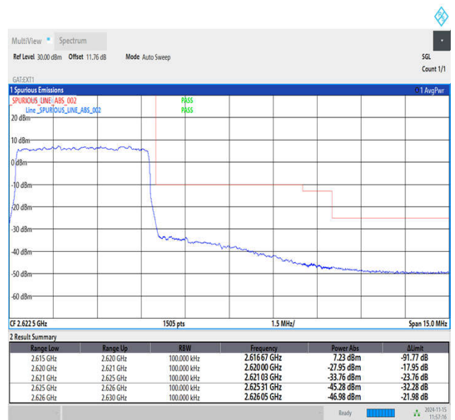
Band38_5MHz_64QAM_38225_1RB#0
