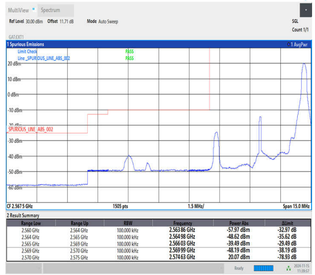
Band38_5MHz_16QAM_37775_1RB#24
