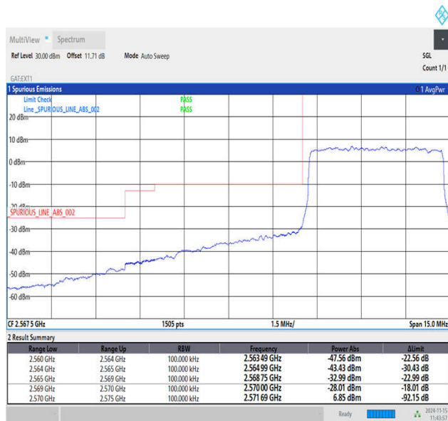
Band38_5MHz_16QAM_37775_1RB#0
