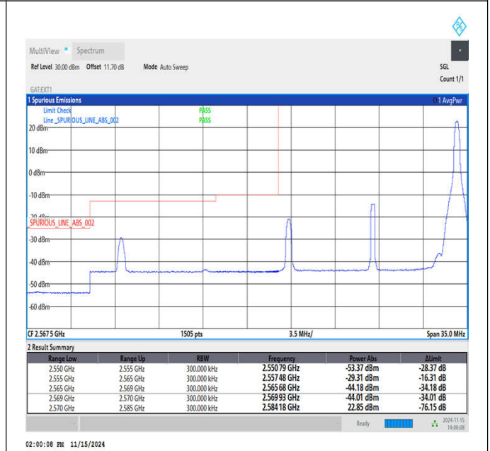
Band38_15MHz_64QAM_37825_1RB#74
