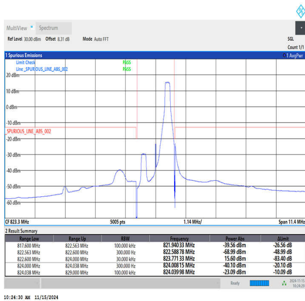
Band26_1.4MHz_64QAM_26783_1RB#5
