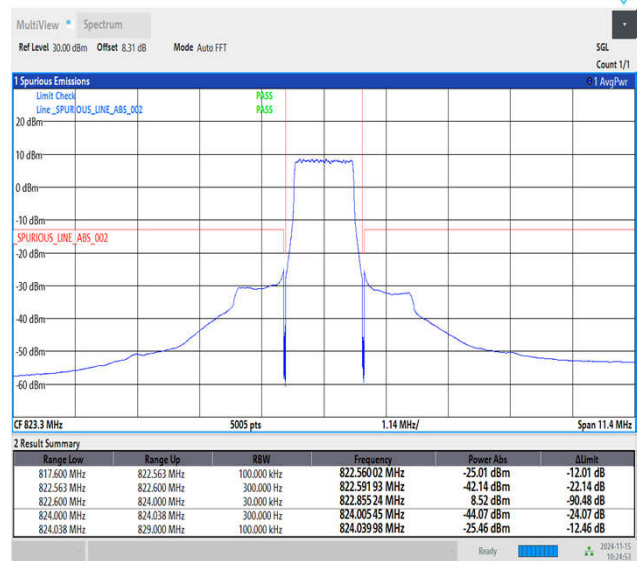
Band26_1.4MHz_QPSK_26783_6RB#0
