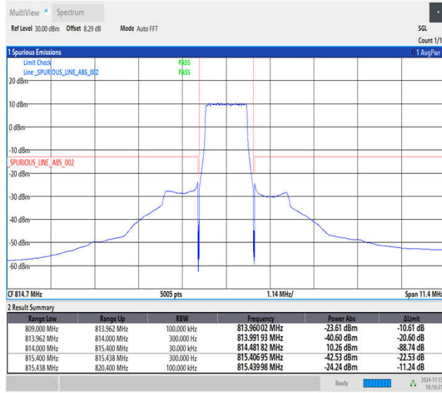
Band26_1.4MHz_QPSK_26697_6RB#0
