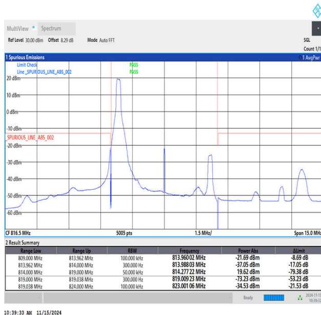
Band26_5MHz_16QAM_26715_1RB#0
