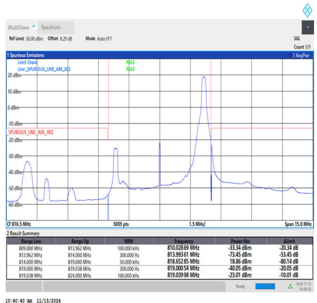
Band26_5MHz_16QAM_26715_1RB#24
