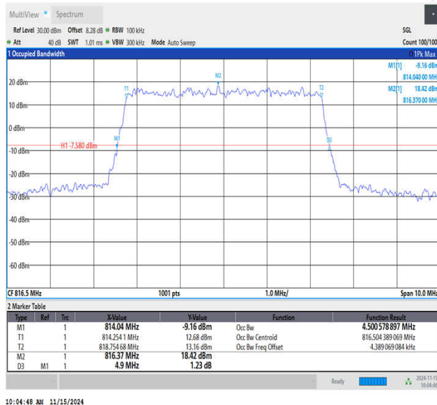
26(814-824)-5MHz-QPSK-26715-25RB#0-PASS
