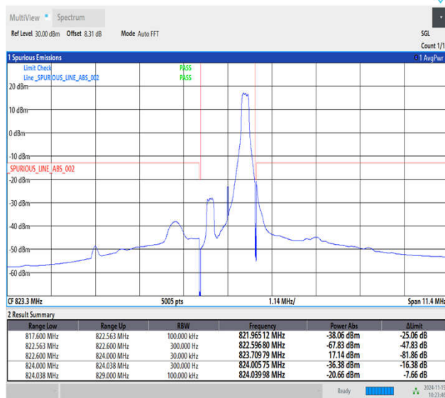
Band26_1.4MHz_QPSK_26783_1RB#5
