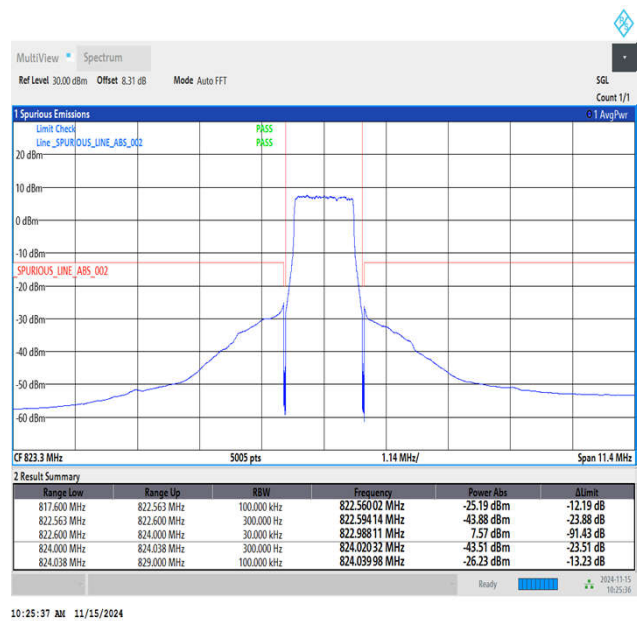
Band26_1.4MHz_64QAM_26783_6RB#0
