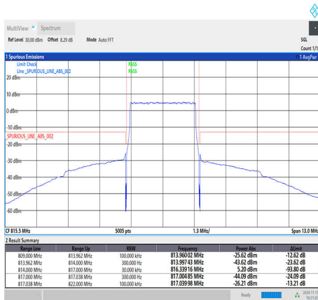
Band26_3MHz_64QAM_26705_1RB#0
