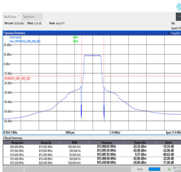
Band26_1.4MHz_16QAM_26697_1RB#0
