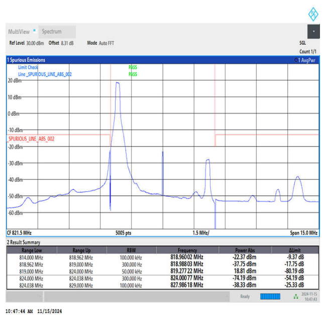
Band26_5MHz_16QAM_26765_1RB#0
