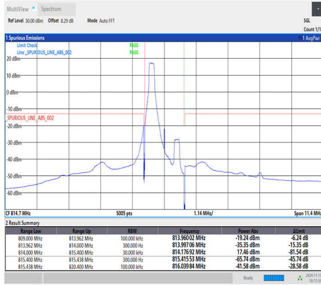
Band26_1.4MHz_16QAM_26697_1RB#0
