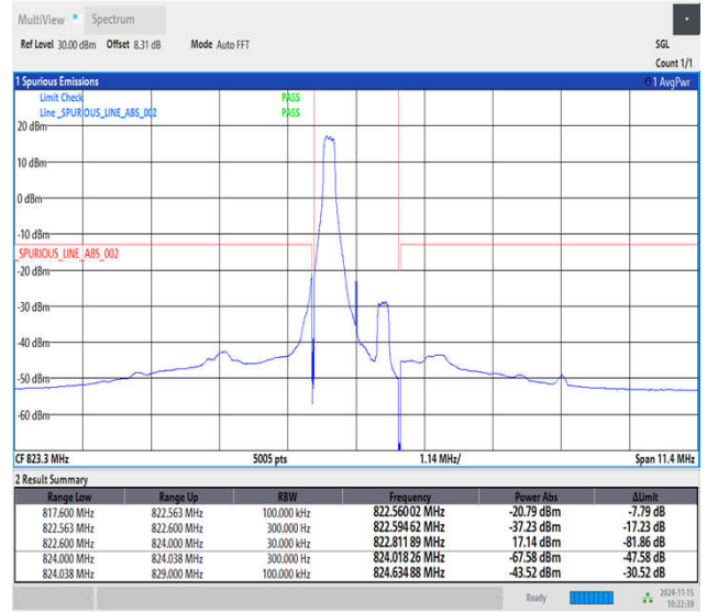
Band26_1.4MHz_QPSK_26783_1RB#0
