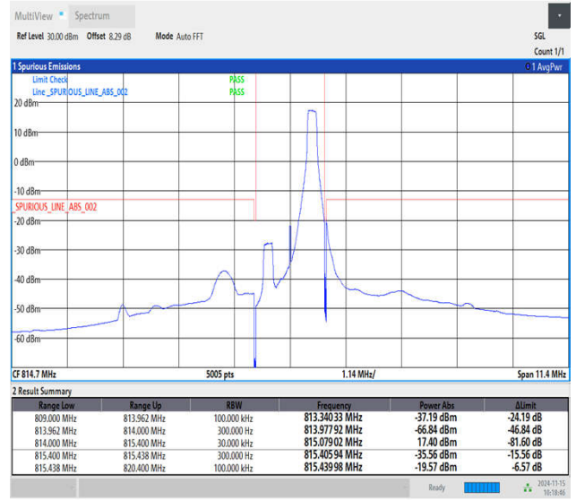
Band26_1.4MHz_16QAM_26697_1RB#5
