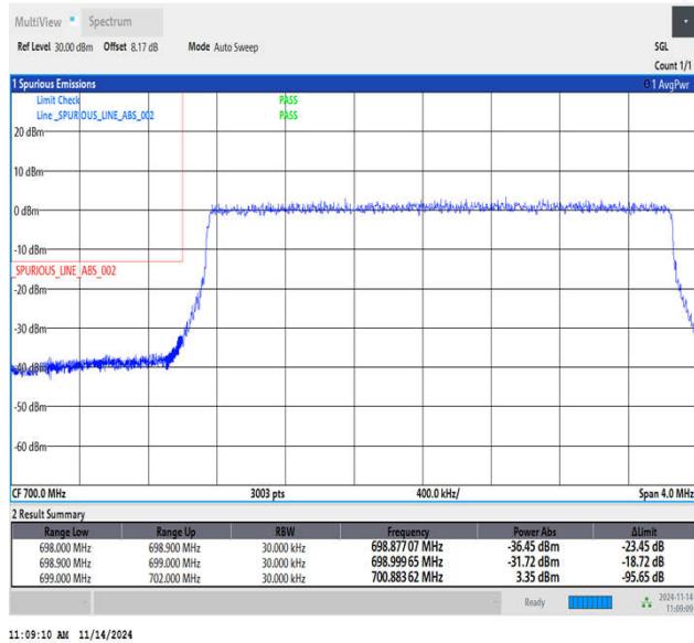
Band12_3MHz_64QAM_23025_15RB#0
