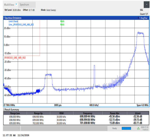
Band12_3MHz_16QAM_23025_1RB#14
