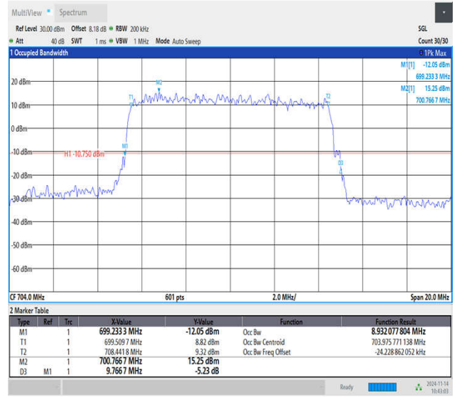
Band12-10MHz-QPSK-23060-50RB#0-PASS
