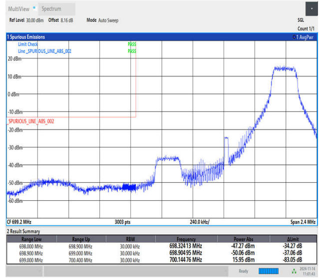
Band12_1.4MHz_16QAM_23017_1RB#5
