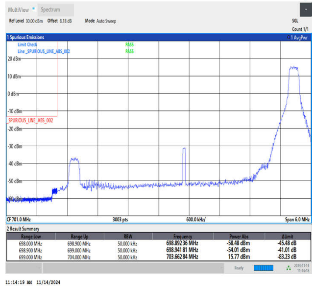
Band12_5MHz_64QAM_23035_1RB#24
