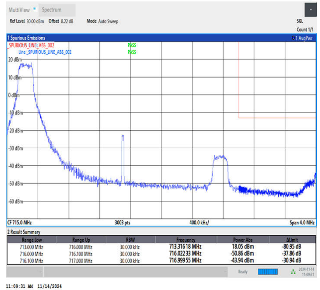
Band12_3MHz_QPSK_23165_1RB#0
