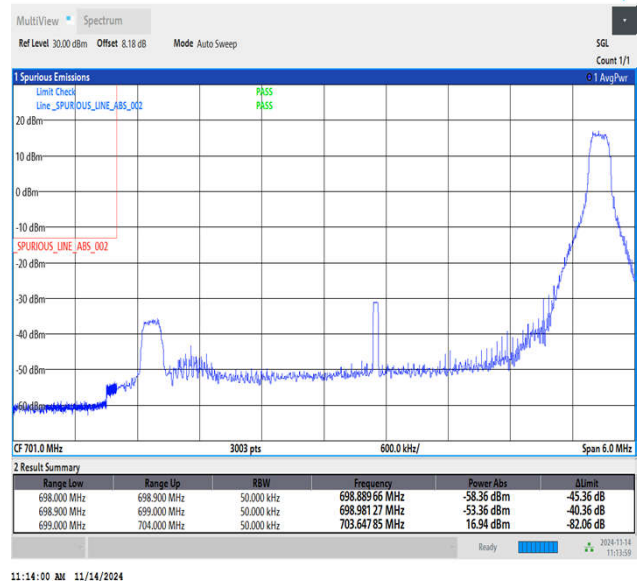
Band12_5MHz_16QAM_23035_1RB#24
