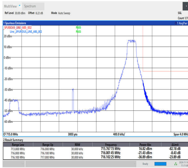
Band12_3MHz_64QAM_23165_1RB#14
