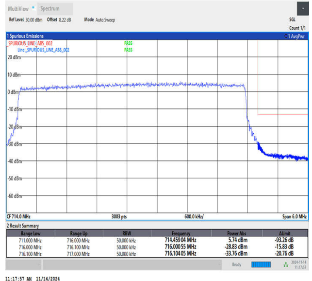
Band12_5MHz_16QAM_23155_25RB#0
