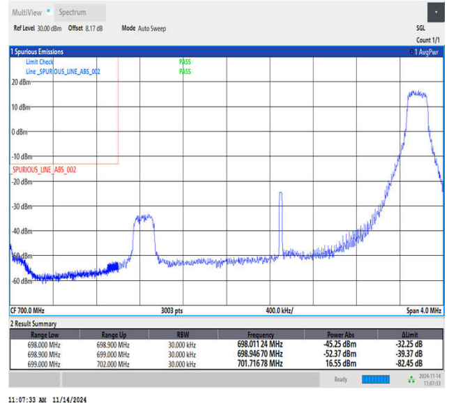
Band12_3MHz_QPSK_23025_1RB#14
