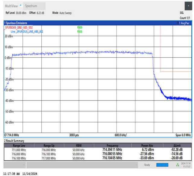
Band12_5MHz_QPSK_23155_25RB#0
