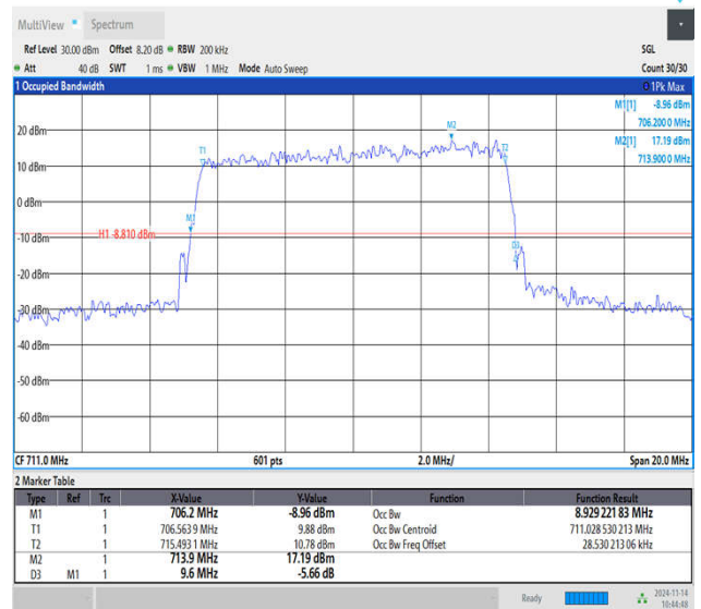
Band12-10MHz-QPSK-23130-50RB#0-PASS
