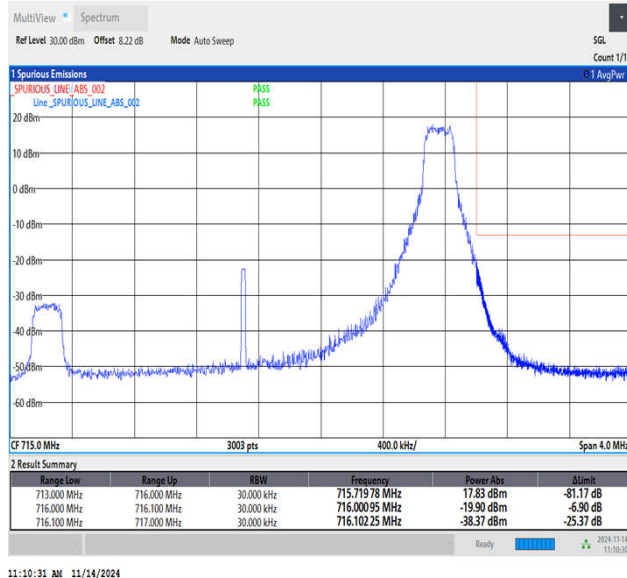
Band12_3MHz_QPSK_23165_1RB#14
