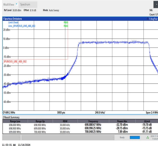
Band12_1.4MHz_64QAM_23017_6RB#0
