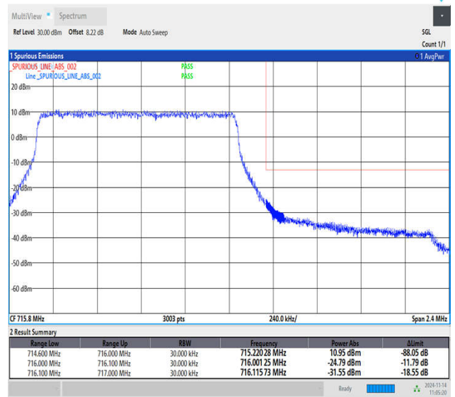
Band12_1.4MHz_QPSK_23173_6RB#0
