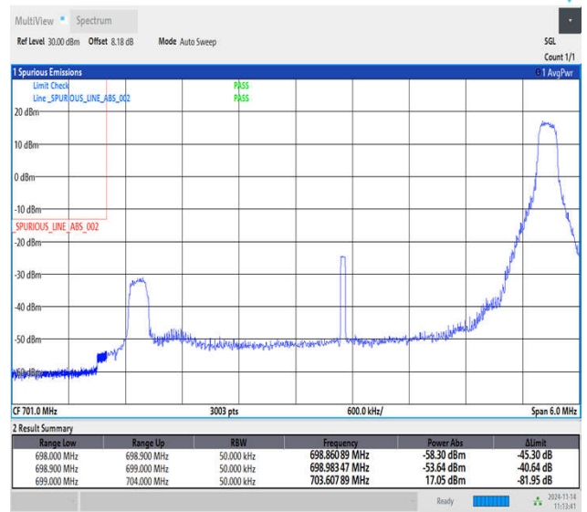
Band12_5MHz_QPSK_23035_1RB#24
