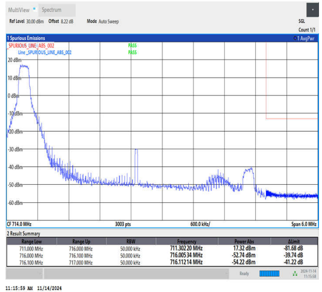
Band12_5MHz_16QAM_23155_1RB#0
