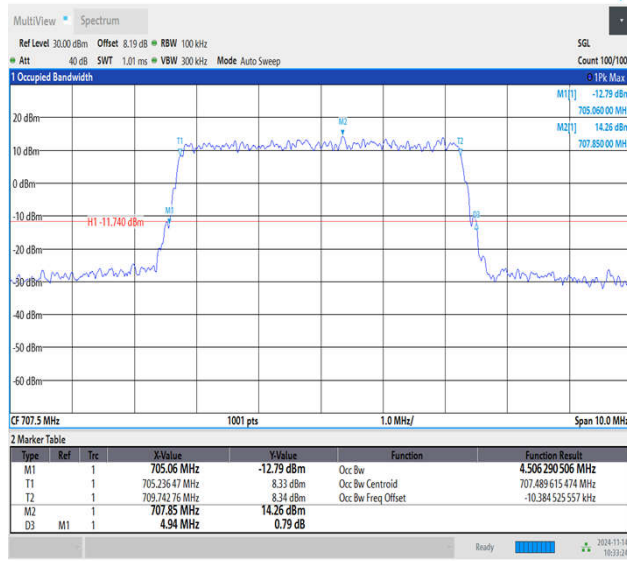
Band12-5MHz-16QAM-23095-25RB#0-PASS
