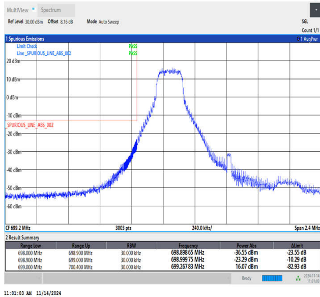
Band12_1.4MHz_64QAM_23017_1RB#0
