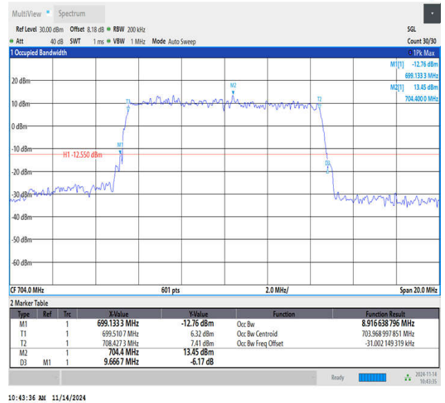
Band12-10MHz-64QAM-23060-50RB#0-PASS
