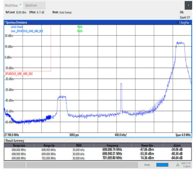
Band12_3MHz_64QAM_23025_1RB#14
