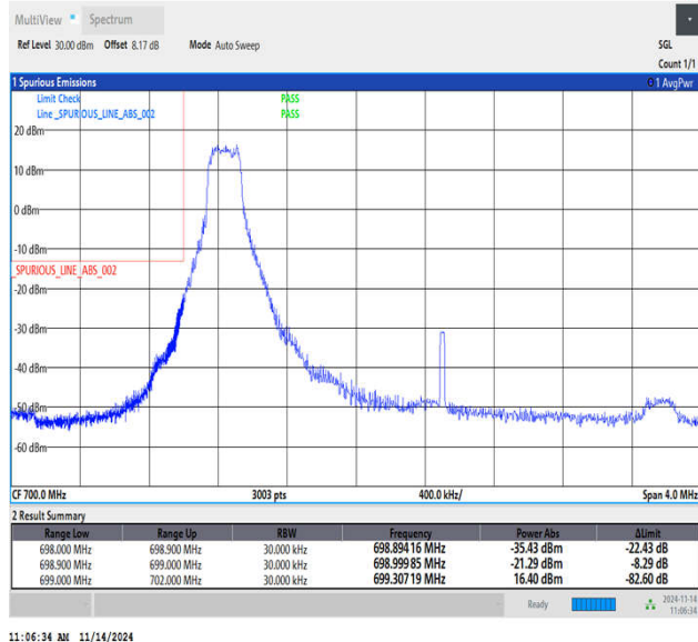
Band12_3MHz_QPSK_23025_1RB#0
