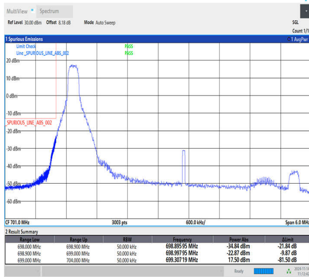
Band12_5MHz_QPSK_23035_1RB#0
