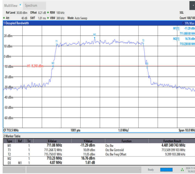
Band12-5MHz-64QAM-23155-25RB#0-PASS
