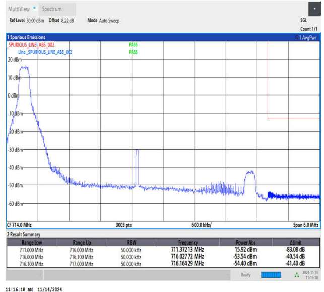
Band12_5MHz_64QAM_23155_1RB#0
