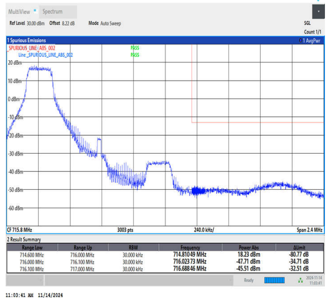
Band12_1.4MHz_16QAM_23173_1RB#0
