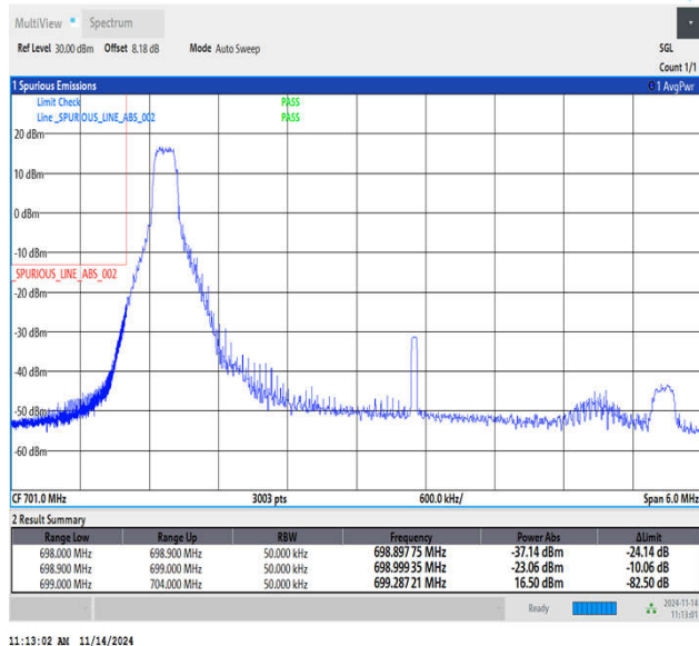
Band12_5MHz_16QAM_23035_1RB#0
