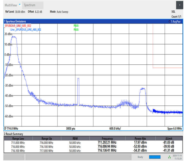
Band12_5MHz_QPSK_23155_1RB#0
