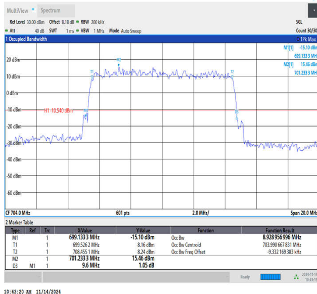
Band12-10MHz-16QAM-23060-50RB#0-PASS
