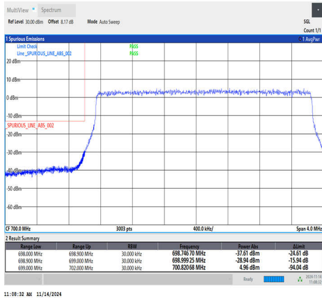
Band12_3MHz_QPSK_23025_15RB#0
