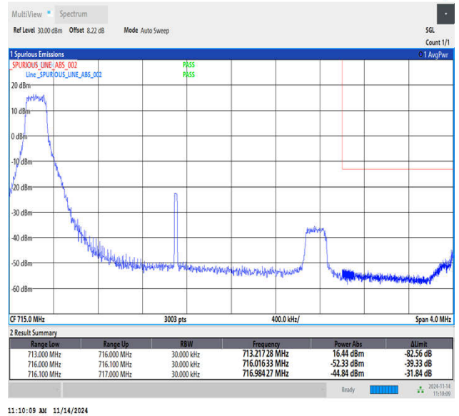
Band12_3MHz_64QAM_23165_1RB#0
