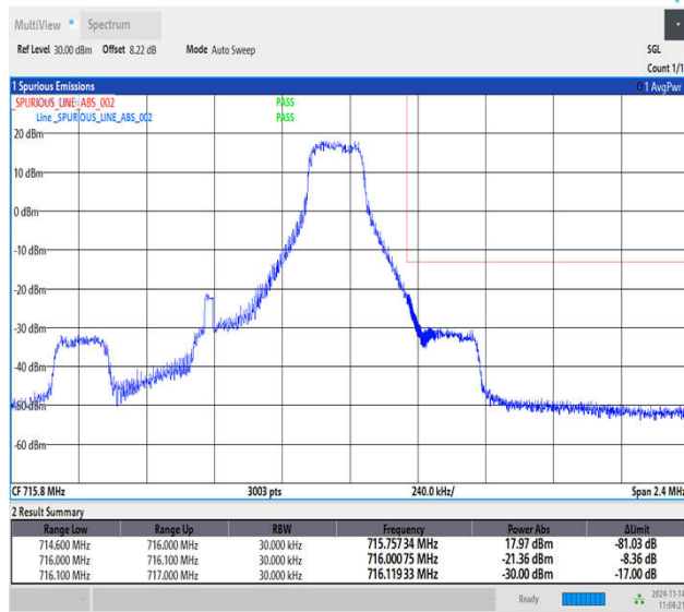
Band12_1.4MHz_QPSK_23173_1RB#5
