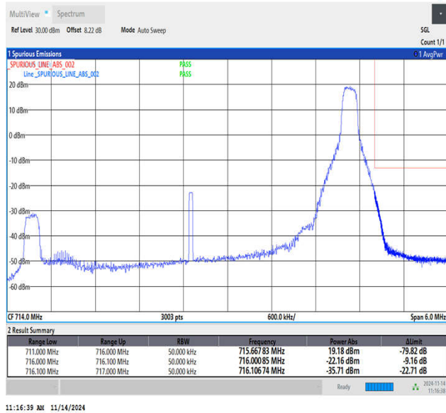
Band12_5MHz_QPSK_23155_1RB#24
