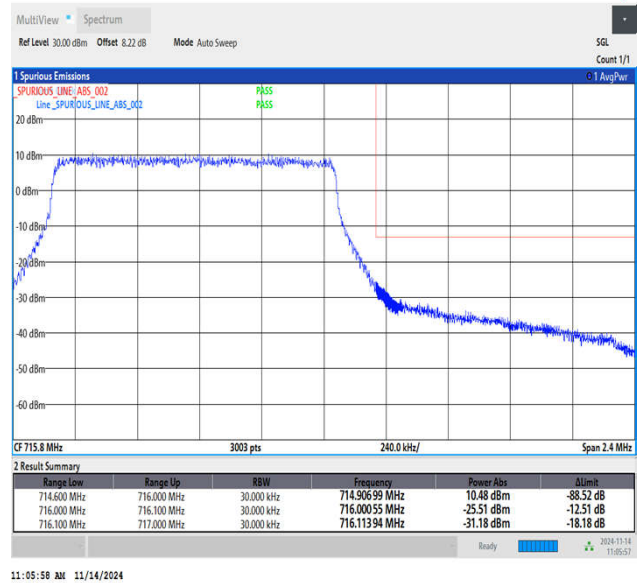
Band12_1.4MHz_64QAM_23173_6RB#0
