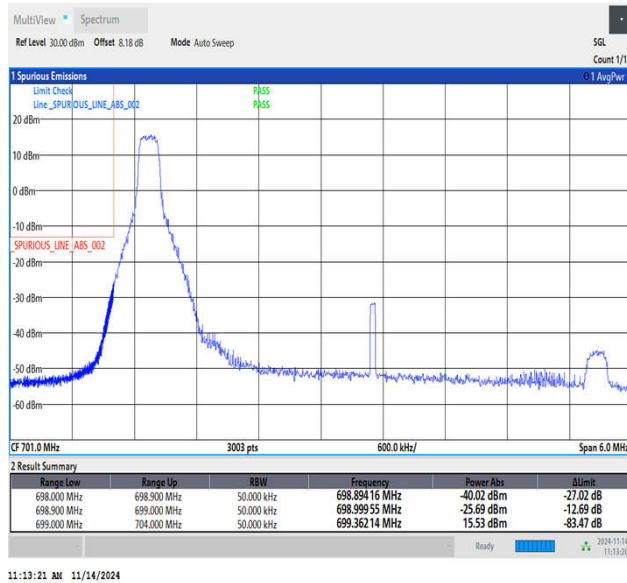
Band12_5MHz_64QAM_23035_1RB#0
