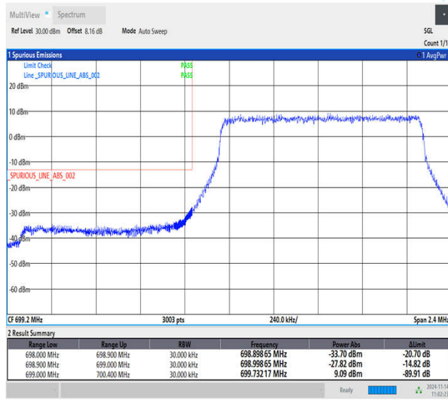
Band12_1.4MHz_QPSK_23017_6RB#0
