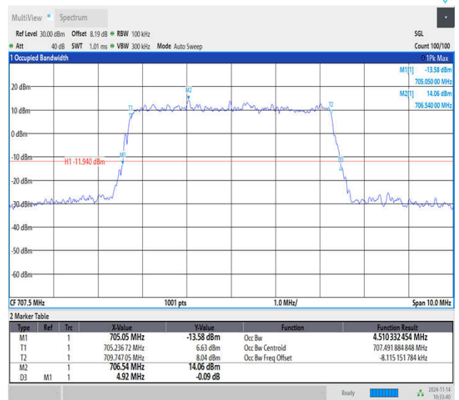
Band12-5MHz-64QAM-23095-25RB#0-PASS
