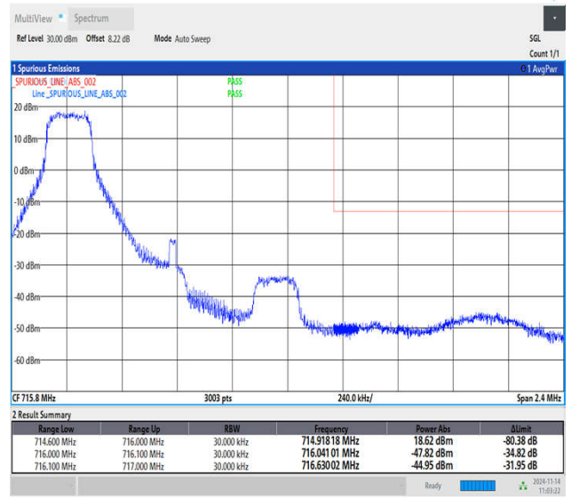
Band12_1.4MHz_QPSK_23173_1RB#0
