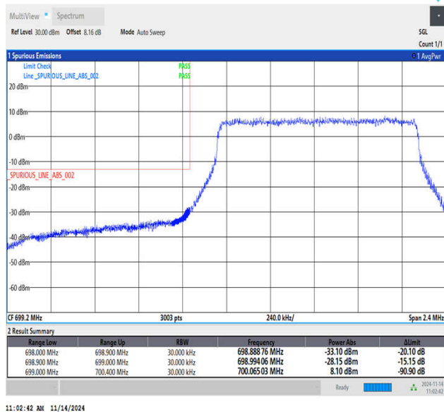
Band12_1.4MHz_16QAM_23017_6RB#0
