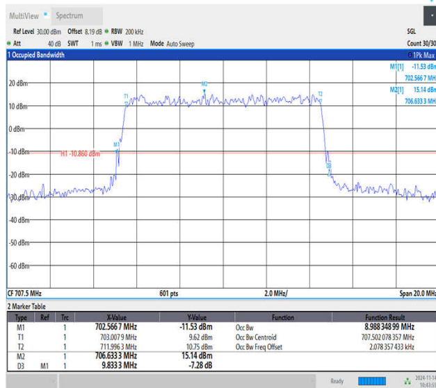
Band12-10MHz-QPSK-23095-50RB#0-PASS
