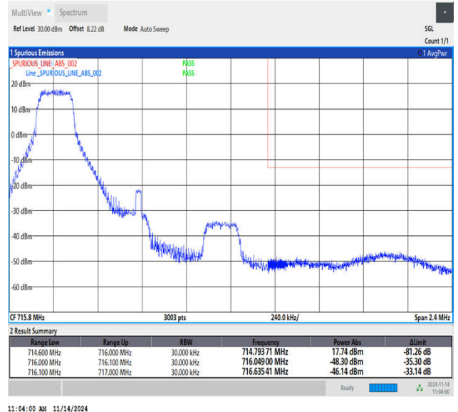
Band12_1.4MHz_64QAM_23173_1RB#0
