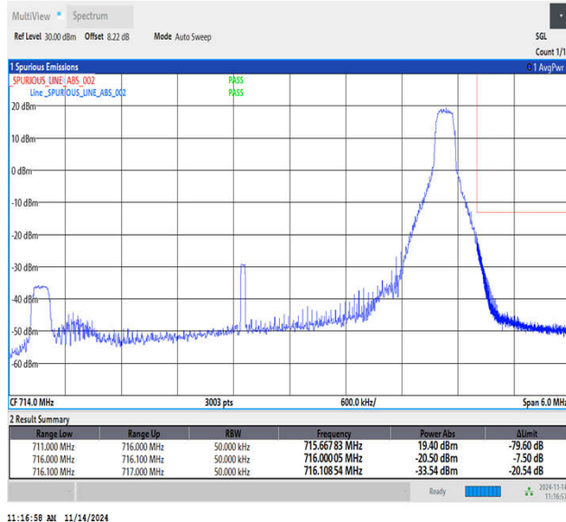
Band12_5MHz_16QAM_23155_1RB#24
