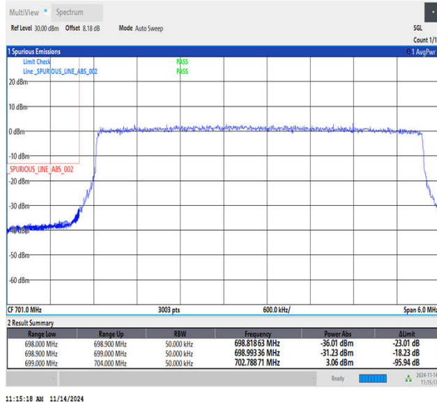
Band12_5MHz_64QAM_23035_25RB#0
