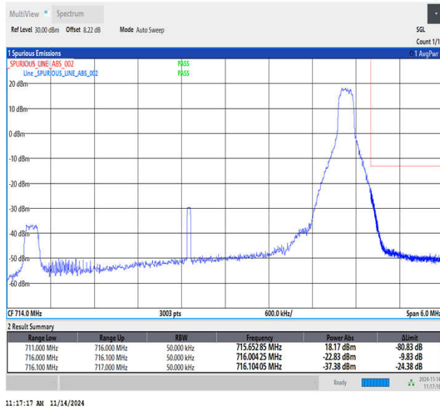
Band12_5MHz_64QAM_23155_1RB#24
