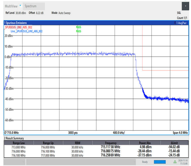
Band12_3MHz_64QAM_23165_15RB#0
