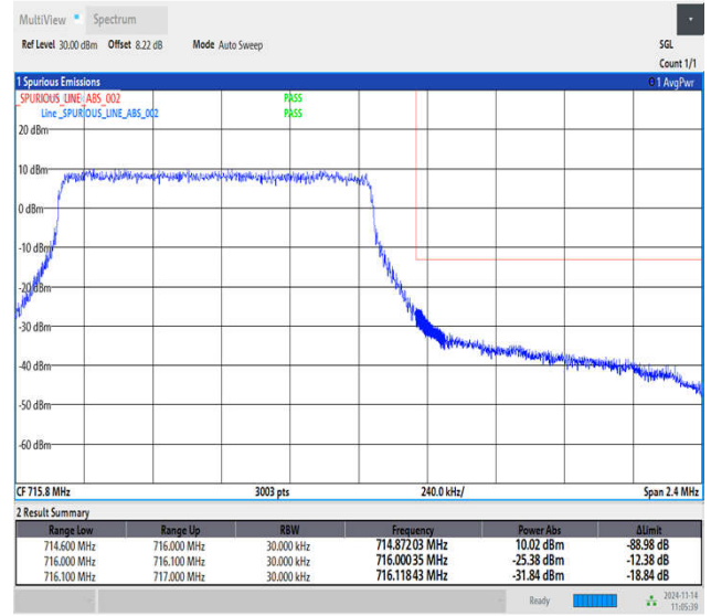
Band12_1.4MHz_16QAM_23173_6RB#0
