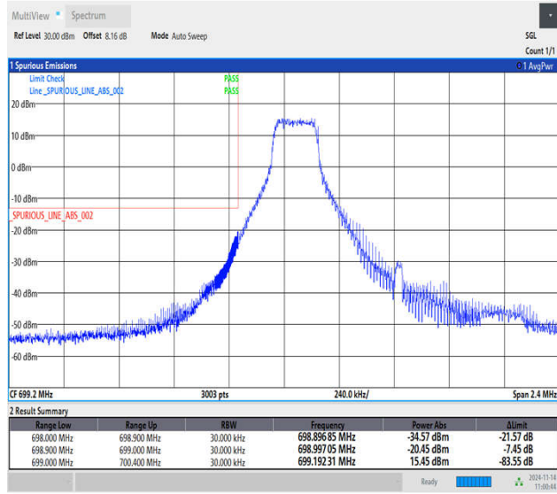
Band12_1.4MHz_16QAM_23017_1RB#0
