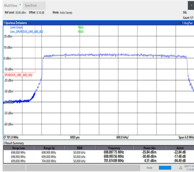
Band12_5MHz_QPSK_23035_25RB#0
