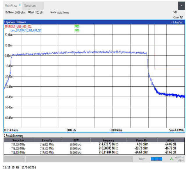
Band12_5MHz_64QAM_23155_25RB#0
