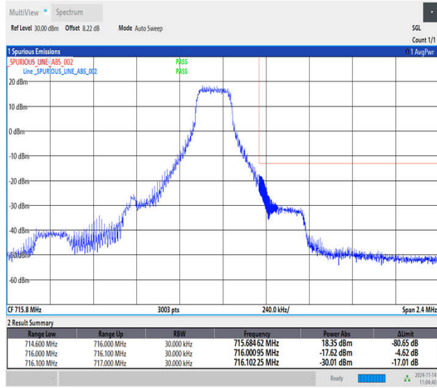
Band12_1.4MHz_16QAM_23173_1RB#5
