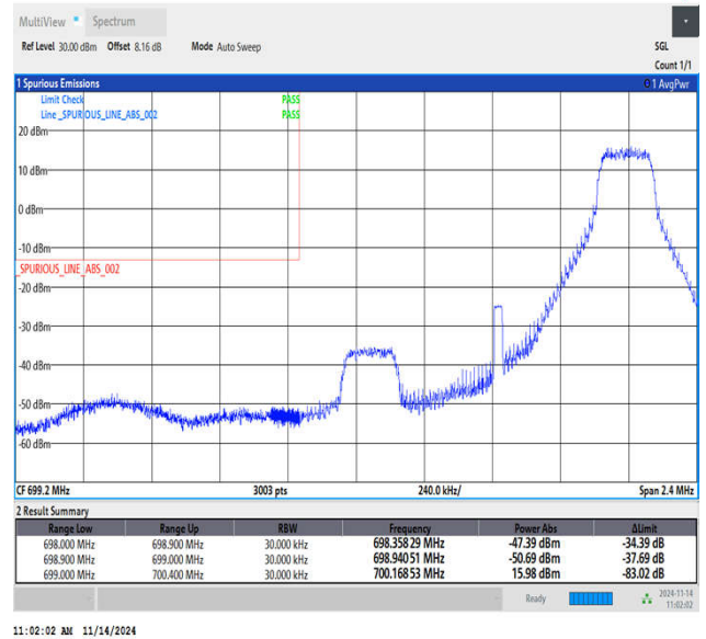
Band12_1.4MHz_64QAM_23017_1RB#5
