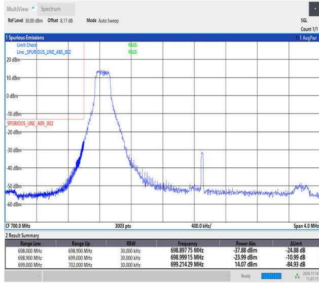
Band12_3MHz_64QAM_23025_1RB#0
