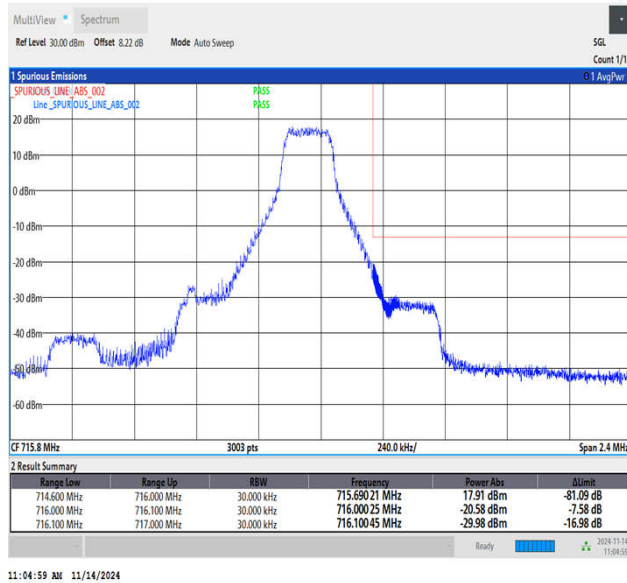
Band12_1.4MHz_64QAM_23173_1RB#5
