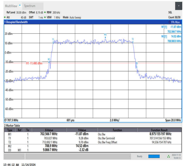
Band12-10MHz-16QAM-23095-50RB#0-PASS
