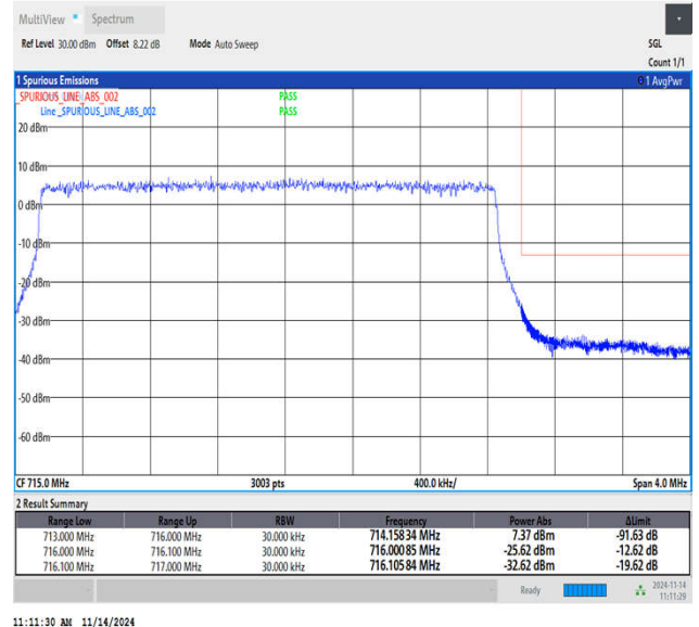
Band12_3MHz_QPSK_23165_15RB#0
