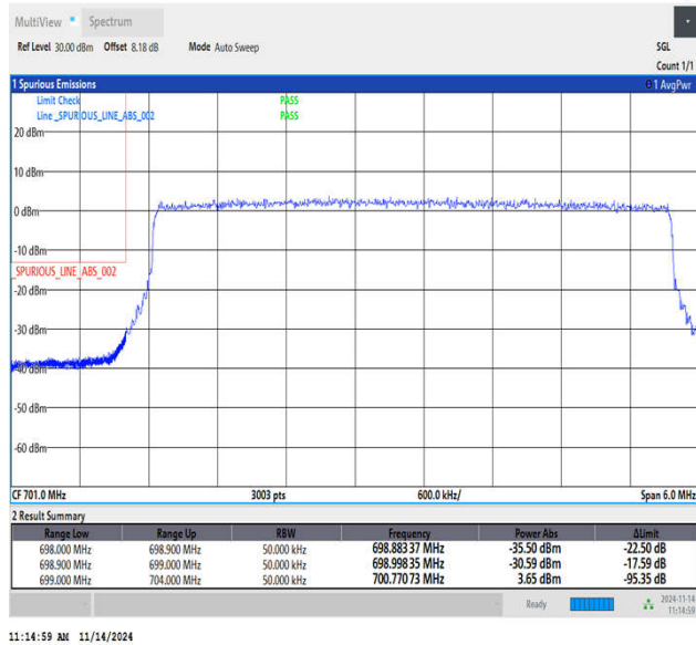
Band12_5MHz_16QAM_23035_25RB#0
