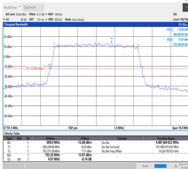
Band12-5MHz-64QAM-23035-25RB#0-PASS
