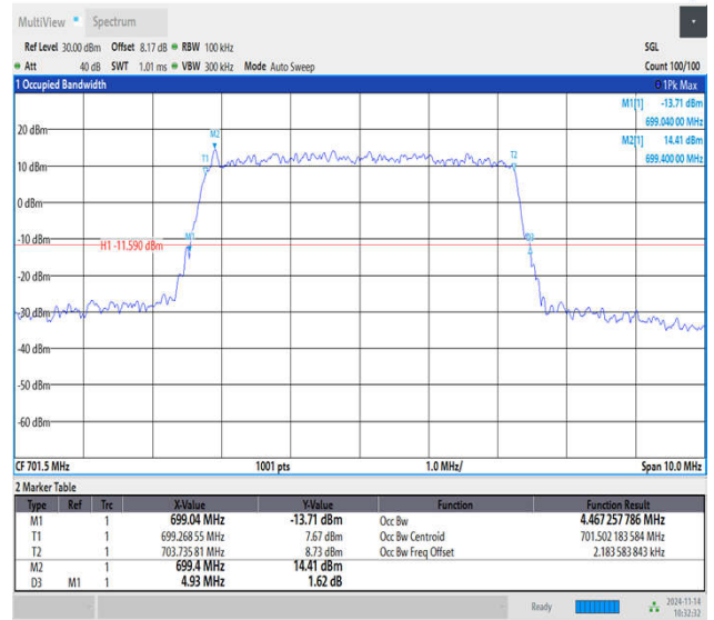
Band12-5MHz-16QAM-23035-25RB#0-PASS
