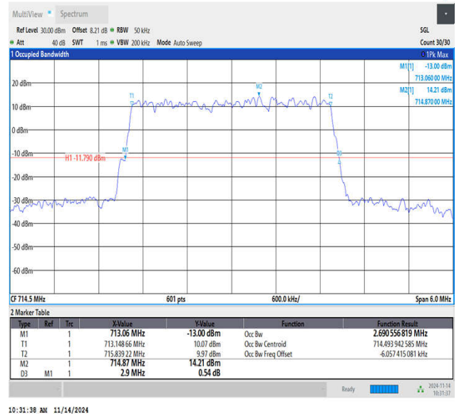
Band12-3MHz-64QAM-23165-15RB#0-PASS
