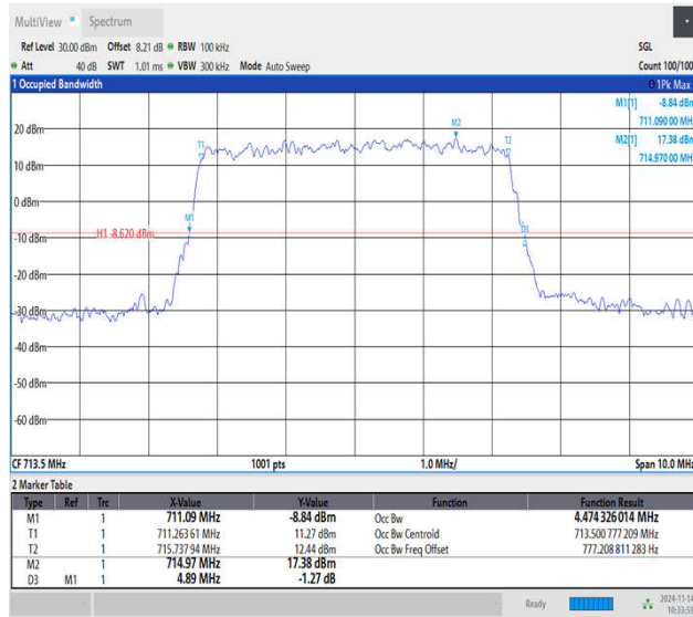
Band12-5MHz-QPSK-23155-25RB#0-PASS
