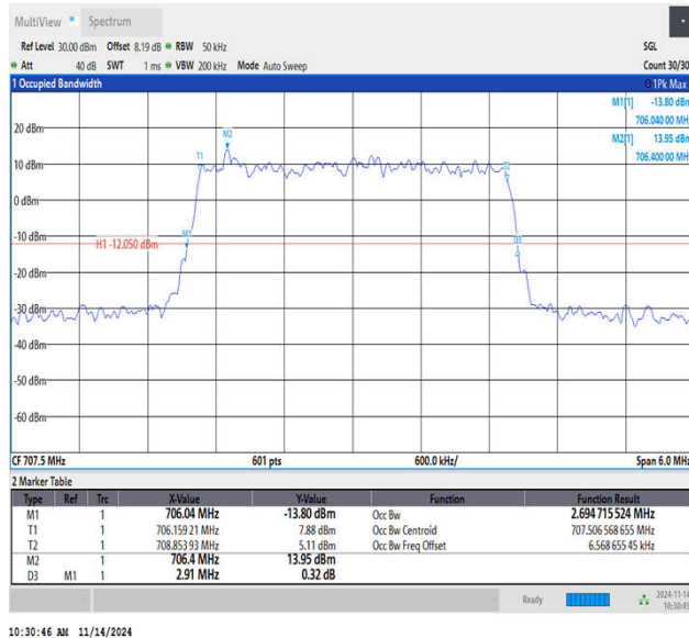
Band12-3MHz-64QAM-23095-15RB#0-PASS
