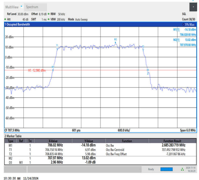
Band12-3MHz-16QAM-23095-15RB#0-PASS
