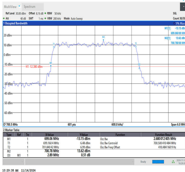
Band12-3MHz-16QAM-23025-15RB#0-PASS
