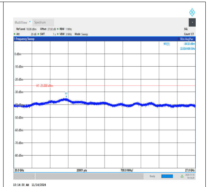
Band7_5MHz_QPSK_21100_1RB#0_20000~27000_20000~27000 7000
