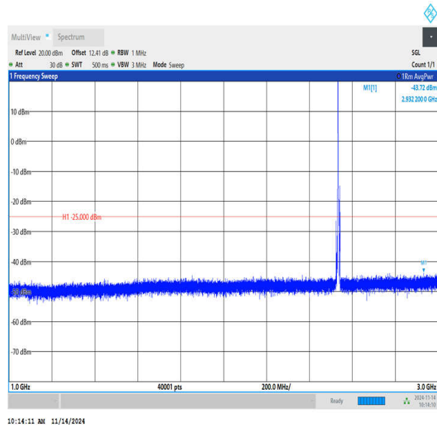
Band7_5MHz_QPSK_21100_1RB#0_1000~3000_1000~3000
