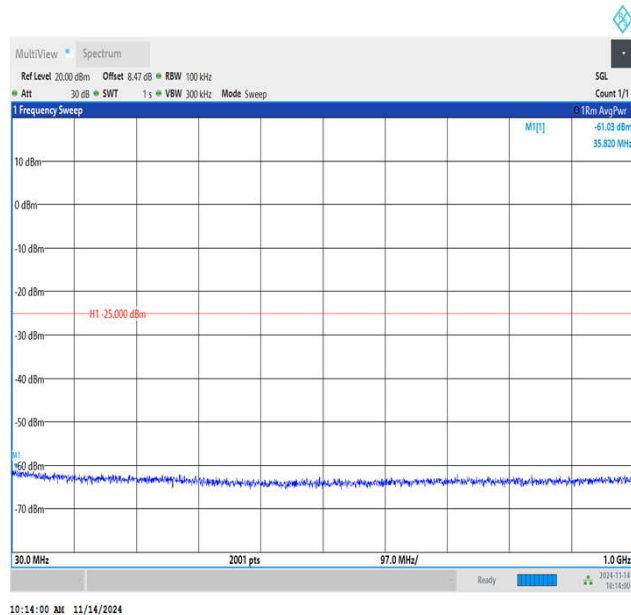
Band7_5MHz_QPSK_21100_1RB#0_30~1000_30~1000
