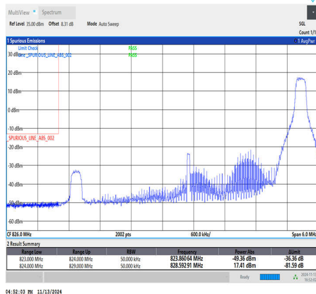
Band5_5MHz_16QAM_20425_1RB#24
