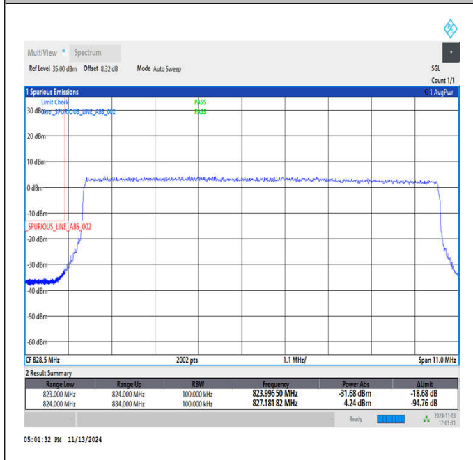
Band5_10MHz_QPSK_20450_50RB#0
