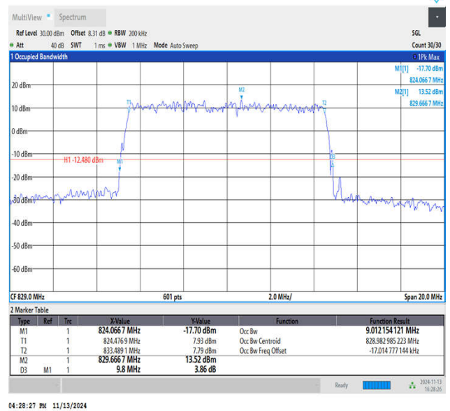
Band5-10MHz-64QAM-20450-50RB#0-PASS
