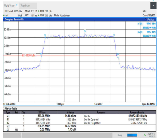
Band5-5MHz-64QAM-20525-25RB#0-PASS
