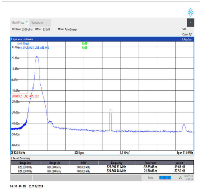
Band5_10MHz_QPSK_20450_1RB#0
