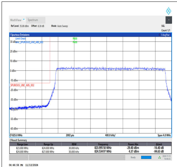
Band5_3MHz_16QAM_20415_15RB#0
