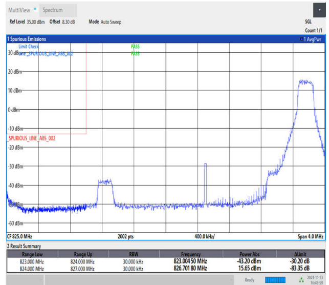
Band5_3MHz_16QAM_20415_1RB#14
