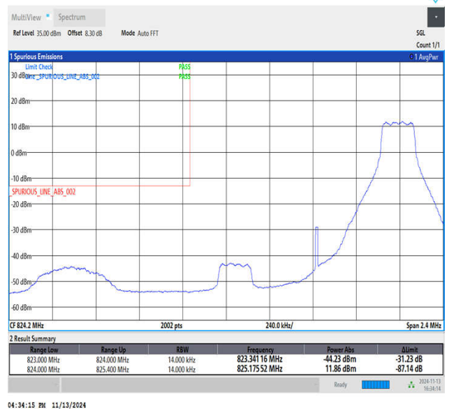
Band5_1.4MHz_64QAM_20407_1RB#5
