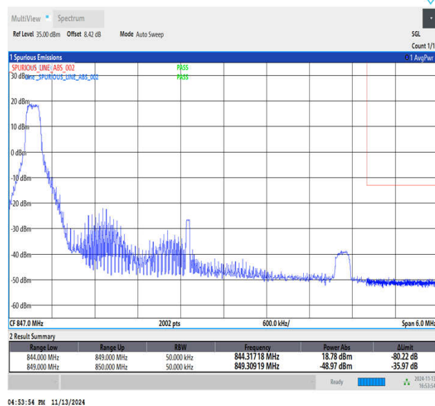
Band5_5MHz_16QAM_20625_1RB#0
