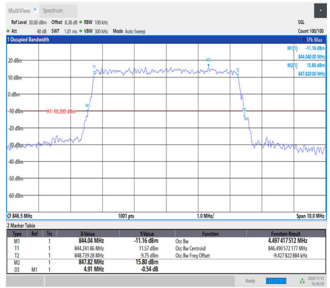
Band5-5MHz-16QAM-20625-25RB#0-PASS
