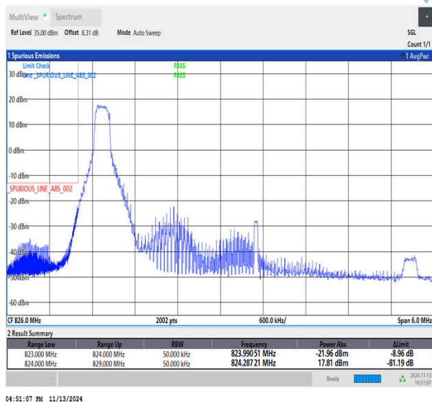
Band5_5MHz_16QAM_20425_1RB#0
