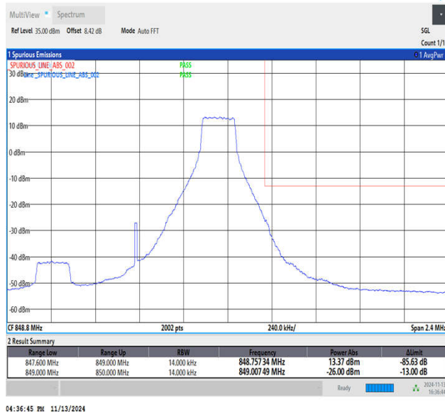
Band5_1.4MHz_16QAM_20643_1RB#5
