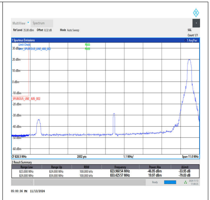
Band5_10MHz_QPSK_20450_1RB#49
