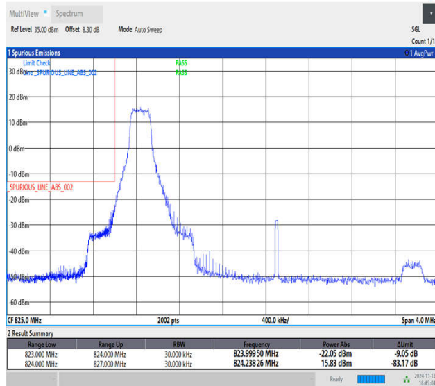
Band5_3MHz_16QAM_20415_1RB#0
