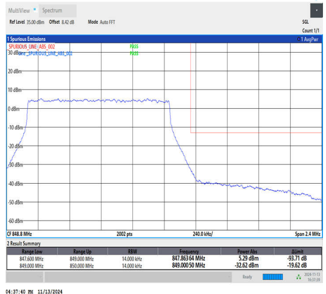
Band5_1.4MHz_16QAM_20643_6RB#0
