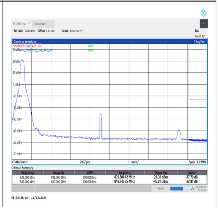
Band5_10MHz_QPSK_20600_1RB#0
