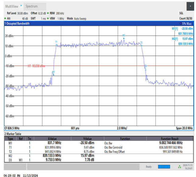
Band5-10MHz-16QAM-20525-50RB#0-PASS
