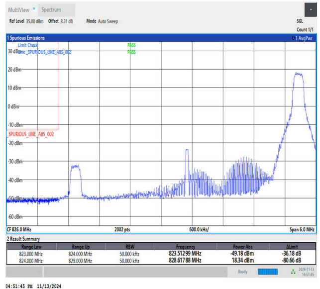
Band5_5MHz_QPSK_20425_1RB#24
