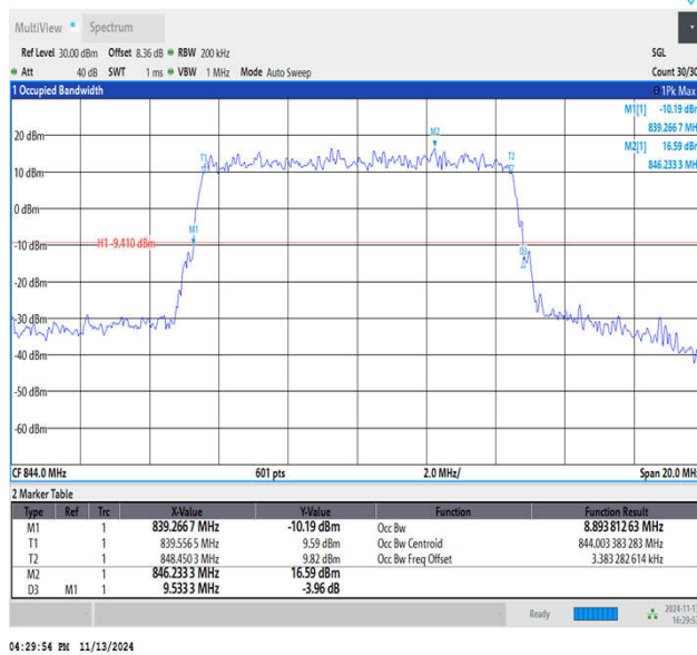
Band5-10MHz-16QAM-20600-50RB#0-PASS
