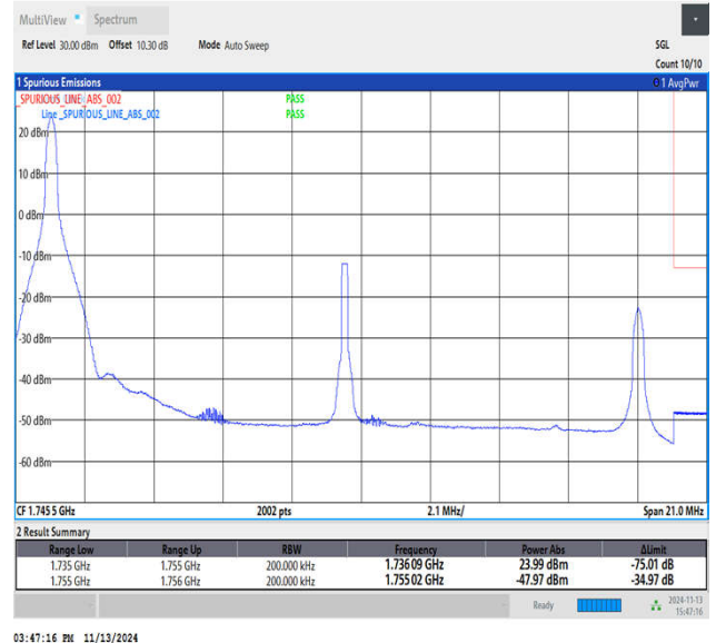
Band4_20MHz_16QAM_20300_1RB#0
