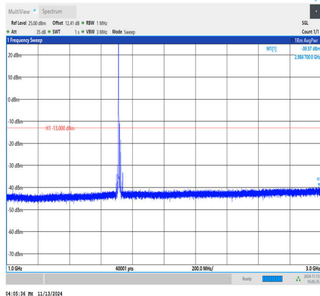
Band4_15MHz_QPSK_20025_1RB#0_1000~3000_1000~3000
