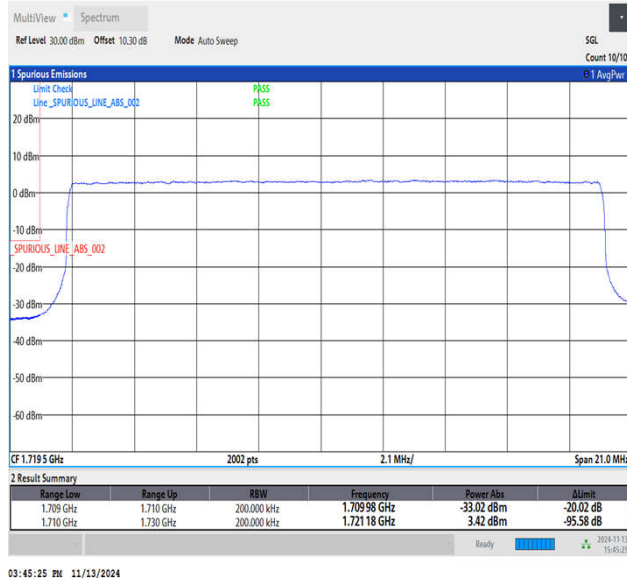
Band4_20MHz_16QAM_20050_100RB#0
