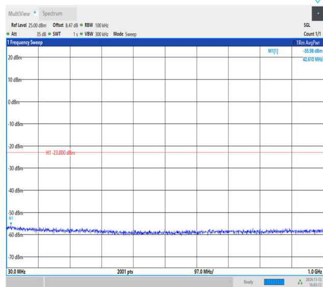
Band4_10MHz_QPSK_20000_1RB#0_30~1000_30~1000
