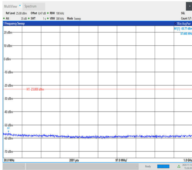
Band4_1.4MHz_QPSK_19957_1RB#0_30~1000_30~1000
