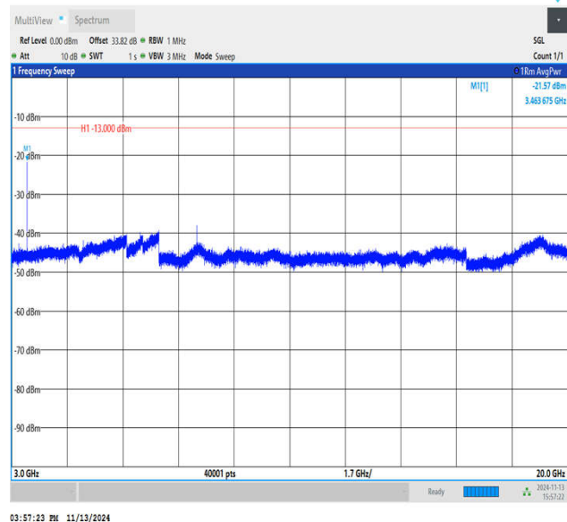
Band4_1.4MHz_QPSK_20175_1RB#0_3000~20000_3000~20000
