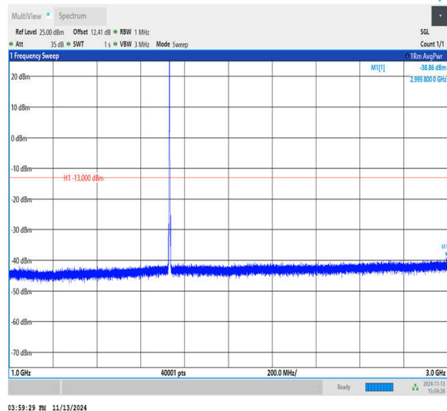
Band4_3MHz_QPSK_20175_1RB#0_1000~3000_1000~3000 0
