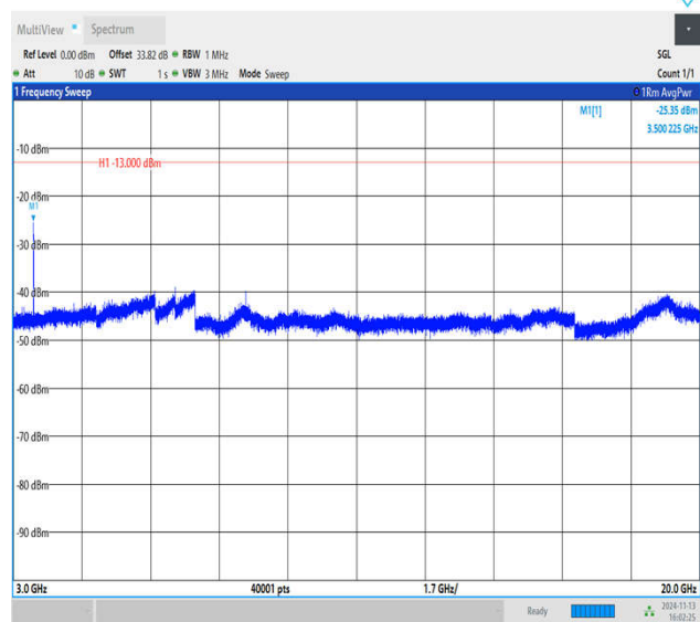
Band4_5MHz_QPSK_20375_1RB#0_3000~20000_3000~20000 000
