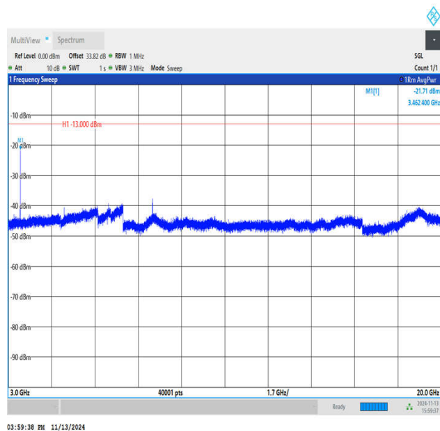
Band4_3MHz_QPSK_20175_1RB#0_3000~20000_3000~20000 000
