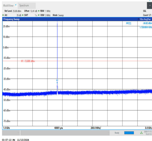
Band4_1.4MHz_QPSK_20175_1RB#0_1000~3000_1000~3000
