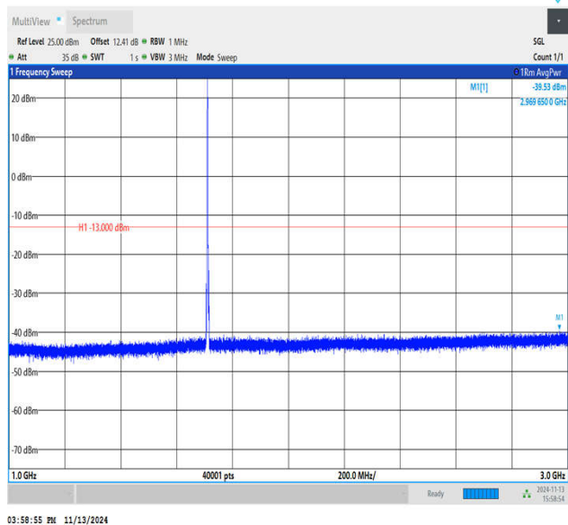
Band4_3MHz_QPSK_19965_1RB#0_1000~3000_1000~3000
