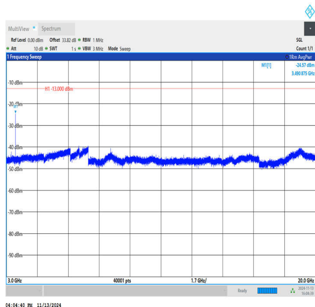
Band4_10MHz_QPSK_20350_1RB#0_3000~20000_3000~20000 0000
