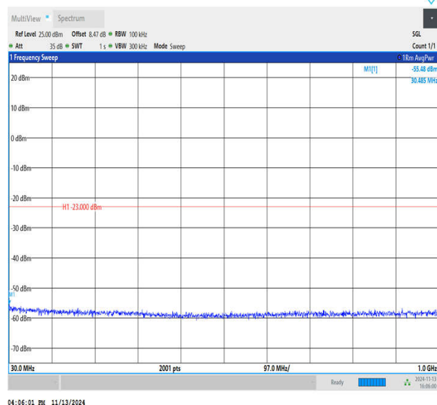
Band4_15MHz_QPSK_20175_1RB#0_30~1000_30~1000
