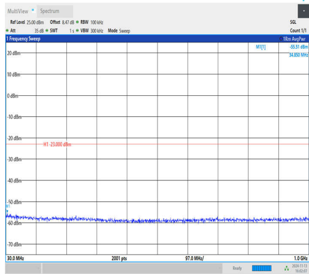
Band4_5MHz_QPSK_20375_1RB#0_30~1000_30~1000
