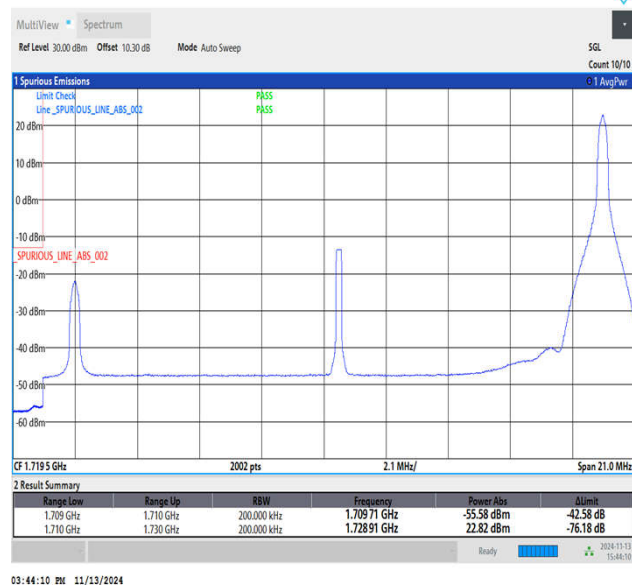
Band4_20MHz_64QAM_20050_1RB#99
