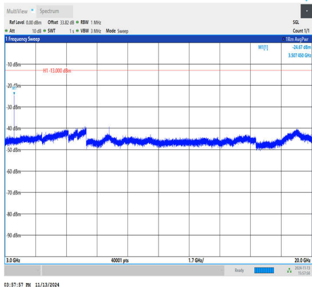
Band4_1.4MHz_QPSK_20393_1RB#0_3000~20000_3000~20000
