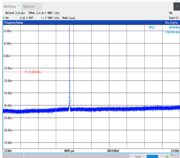
Band4_3MHz_QPSK_20385_1RB#0_1000~3000_1000~300
