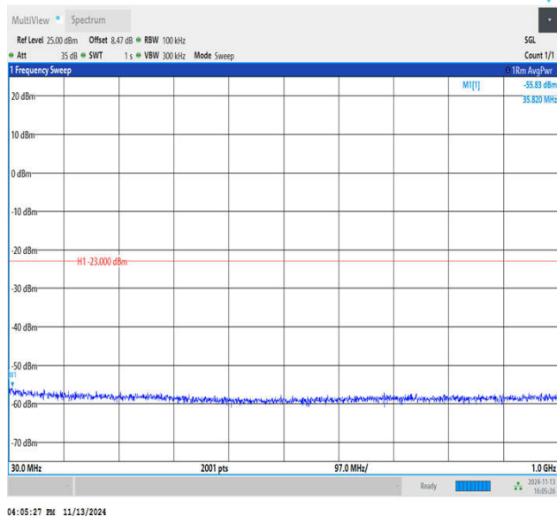
Band4_15MHz_QPSK_20025_1RB#0_30~1000_30~1000
