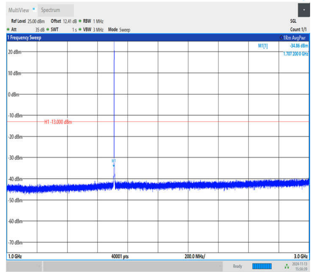
Band4_1.4MHz_QPSK_19957_1RB#0_1000~3000_1000~3000
