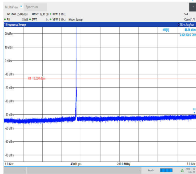
Band4_5MHz_QPSK_20375_1RB#0_1000~3000_1000~3000 0
