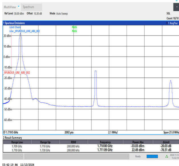
Band4_20MHz_64QAM_20050_1RB#0
