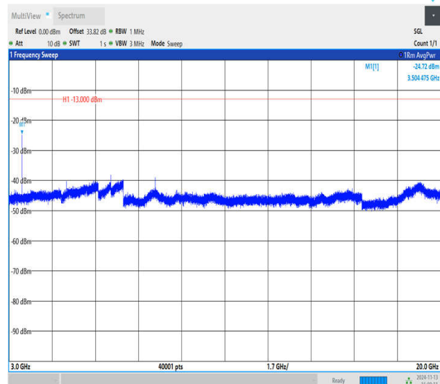
Band4_3MHz_QPSK_20385_1RB#0_3000~20000_3000~20
