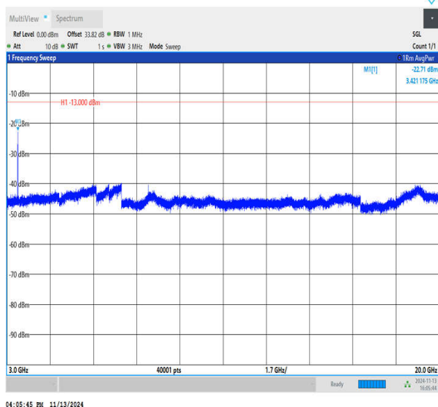
Band4_15MHz_QPSK_20025_1RB#0_3000~20000_3000~20000
