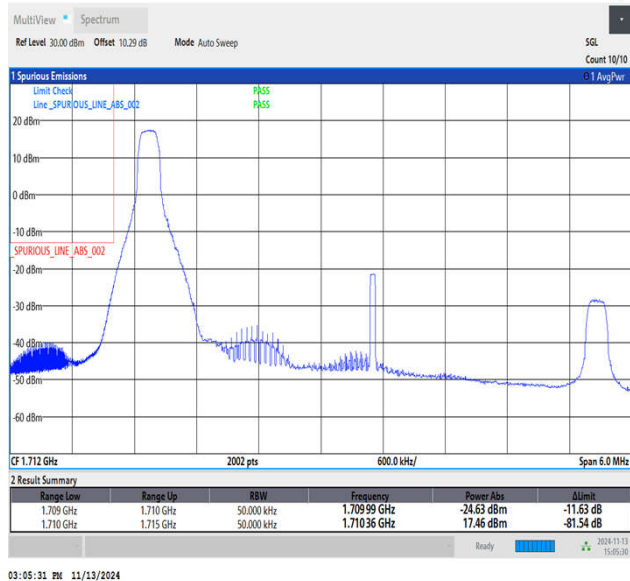
Band4_5MHz_64QAM_19975_1RB#0
