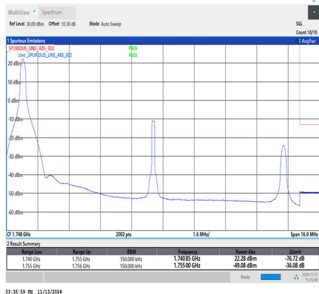
Band4_15MHz_64QAM_20325_1RB#0
