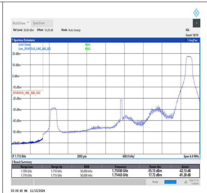
Band4_5MHz_16QAM_19975_1RB#24
