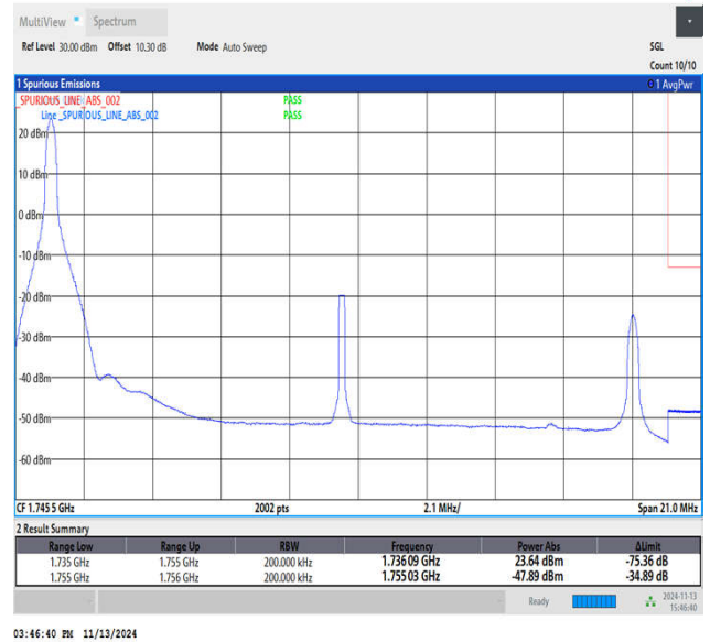
Band4_20MHz_QPSK_20300_1RB#0
