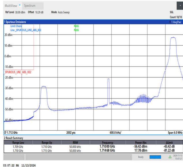
Band4_5MHz_64QAM_19975_1RB#24
