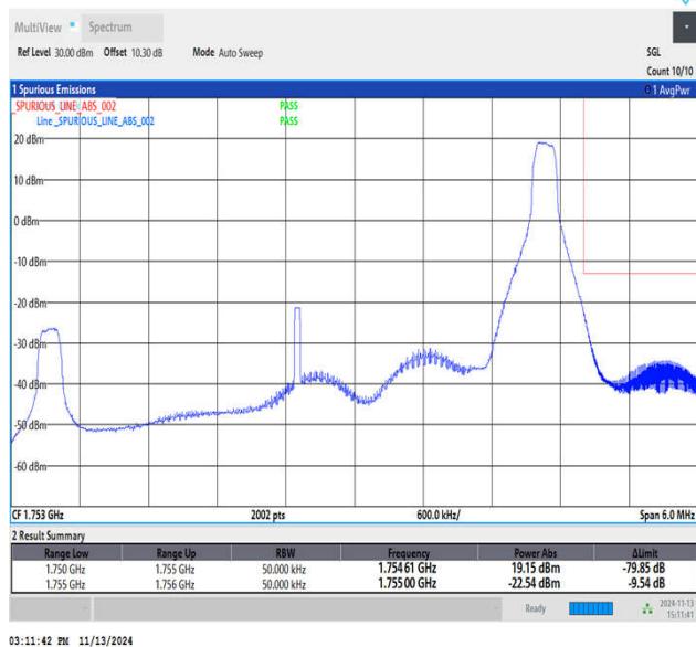
Band4_5MHz_QPSK_20375_1RB#24
