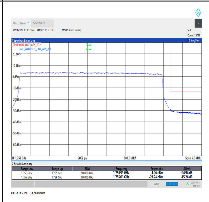
Band4_5MHz_64QAM_20375_25RB#0
