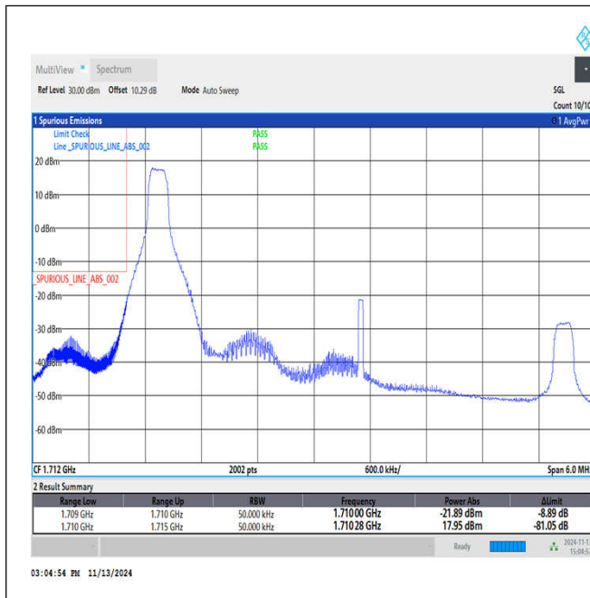
Band4_5MHz_16QAM_19975_1RB#0
