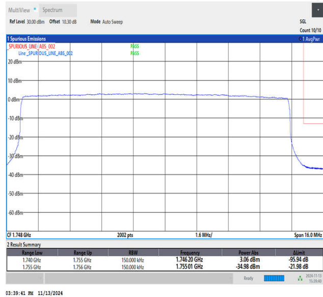
Band4_15MHz_64QAM_20325_75RB#0
