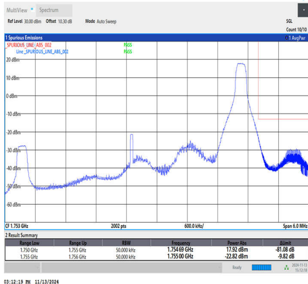
Band4_5MHz_16QAM_20375_1RB#24
