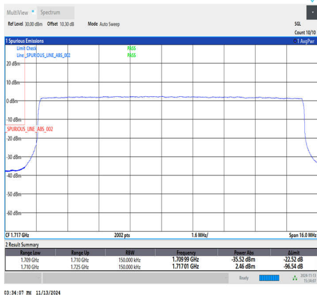
Band4_15MHz_64QAM_20025_75RB#0
