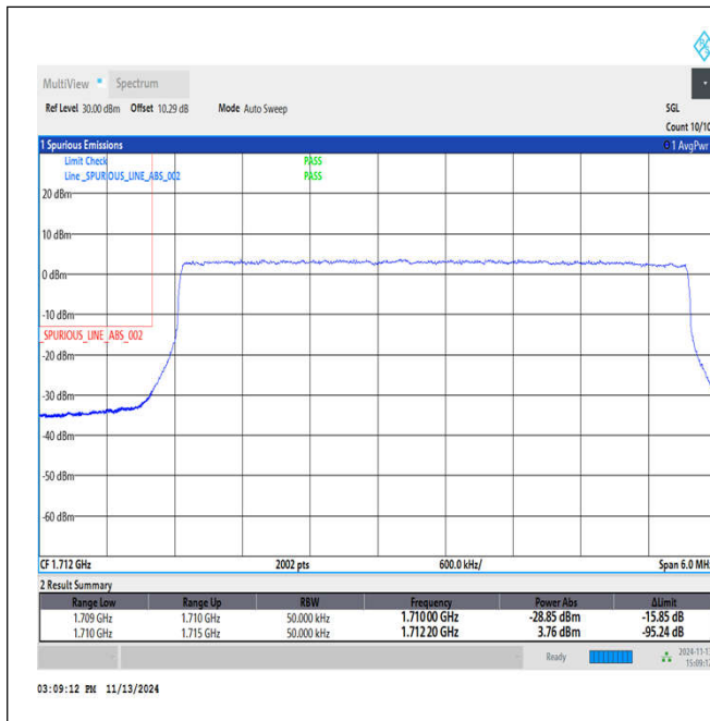
Band4_5MHz_64QAM_19975_25RB#0
