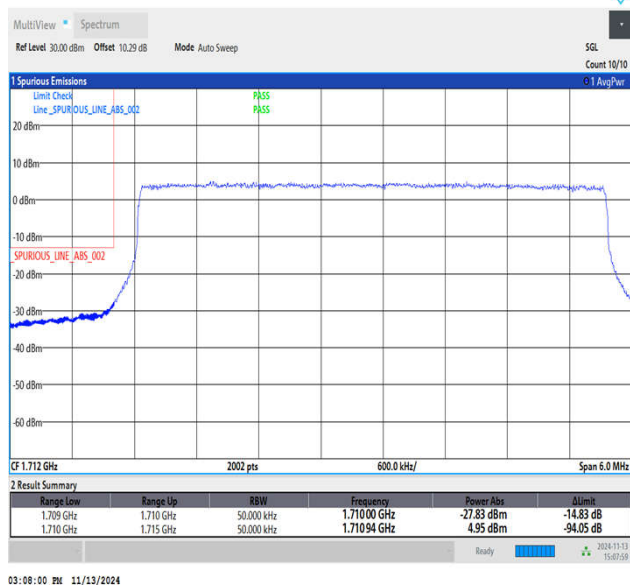
Band4_5MHz_QPSK_19975_25RB#0
