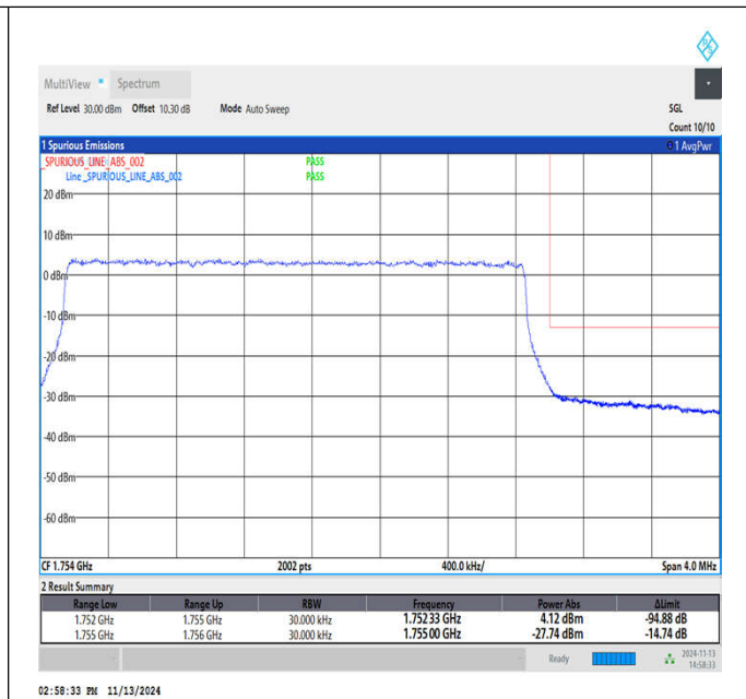
Band4_3MHz_64QAM_20385_15RB#0
