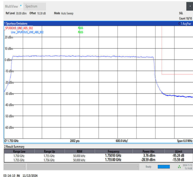
Band4_5MHz_16QAM_20375_25RB#0
