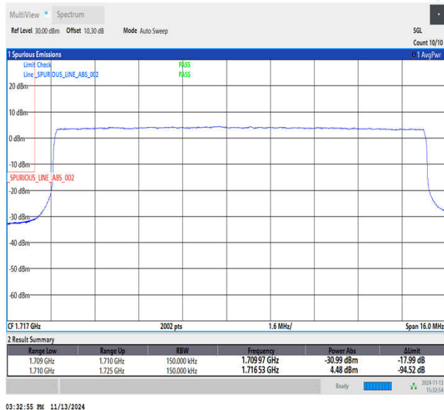
Band4_15MHz_QPSK_20025_75RB#0
