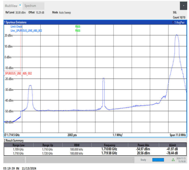
Band4_10MHz_16QAM_20000_1RB#49
