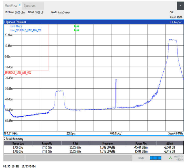
Band4_3MHz_16QAM_19965_1RB#14
