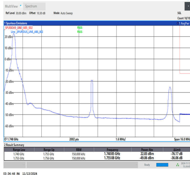
Band4_15MHz_QPSK_20325_1RB#0
