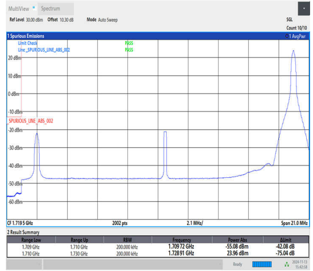
Band4_20MHz_QPSK_20050_1RB#99
