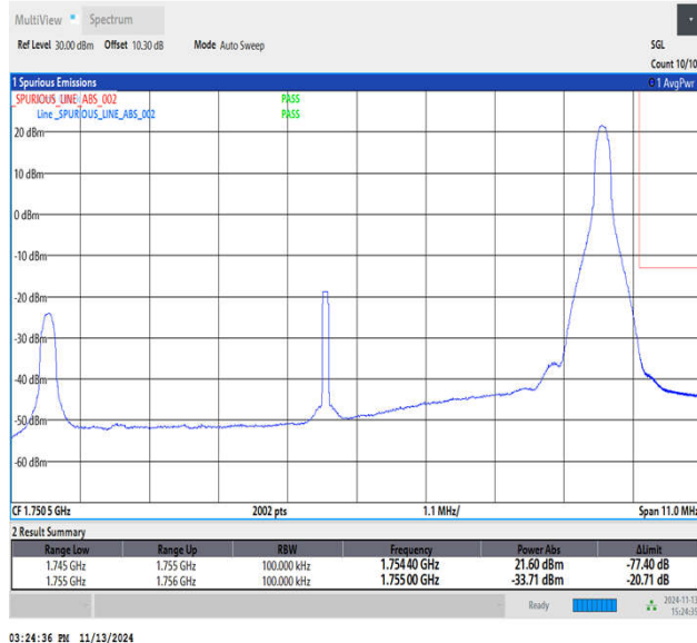
Band4_10MHz_QPSK_20350_1RB#49
