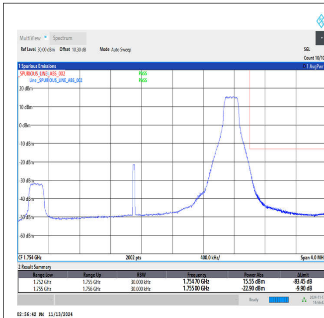
Band4_3MHz_64QAM_20385_1RB#14
