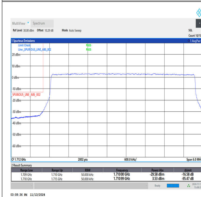
Band4_5MHz_16QAM_19975_1RB#0
