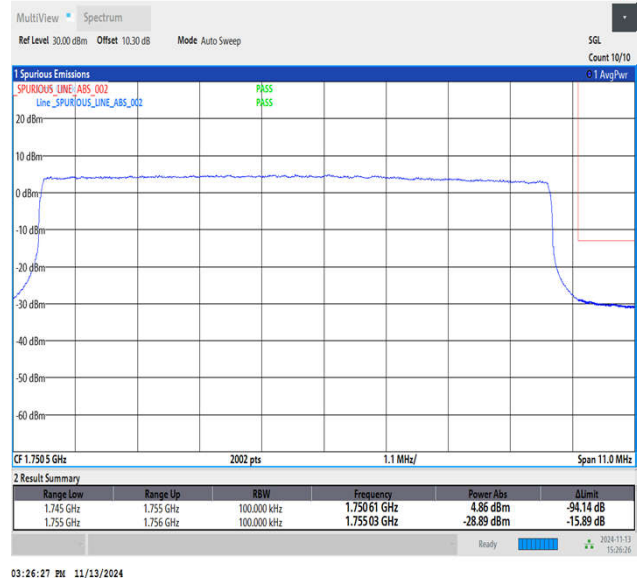
Band4_10MHz_QPSK_20350_50RB#0
