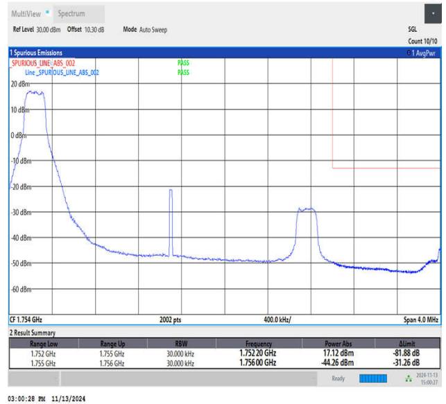
Band4_3MHz_QPSK_20385_1RB#0
