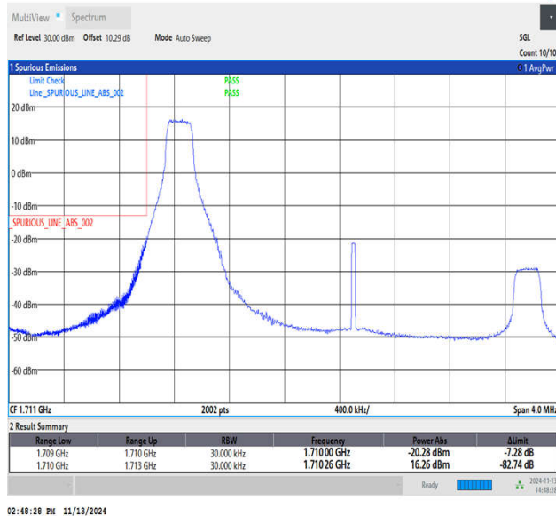
Band4_3MHz_16QAM_19965_1RB#0
