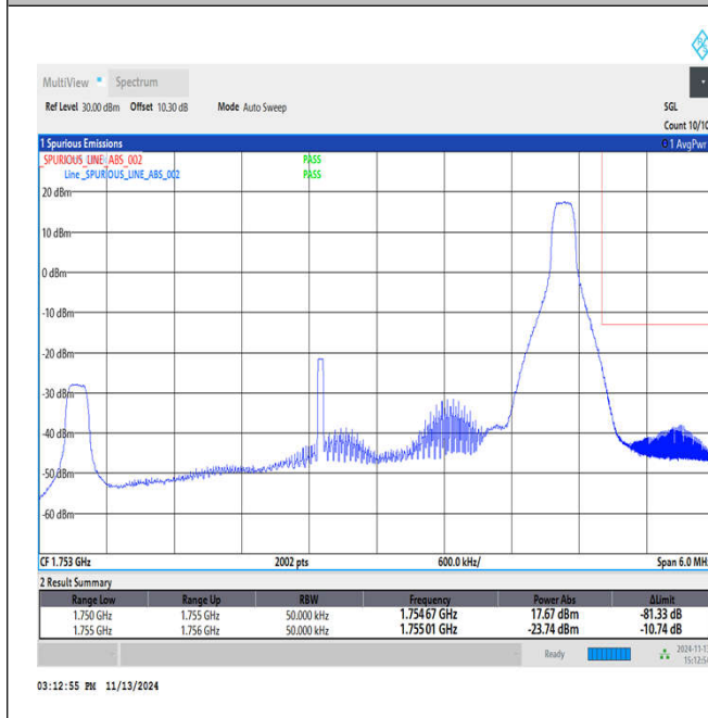
Band4_5MHz_64QAM_20375_1RB#24
