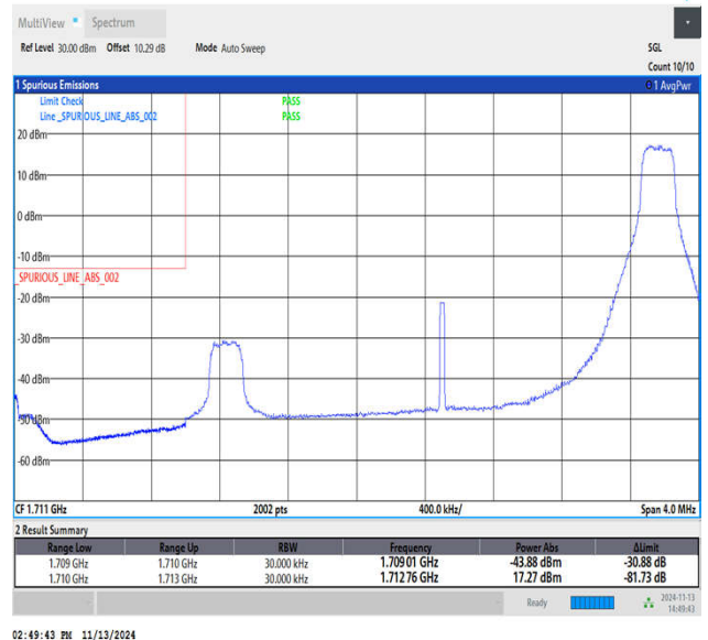
Band4_3MHz_QPSK_19965_1RB#14
