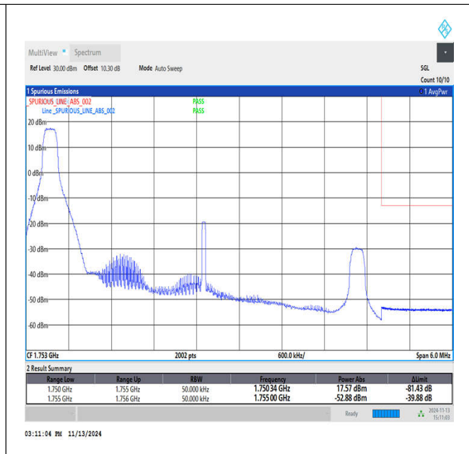
Band4_5MHz_64QAM_20375_1RB#0
