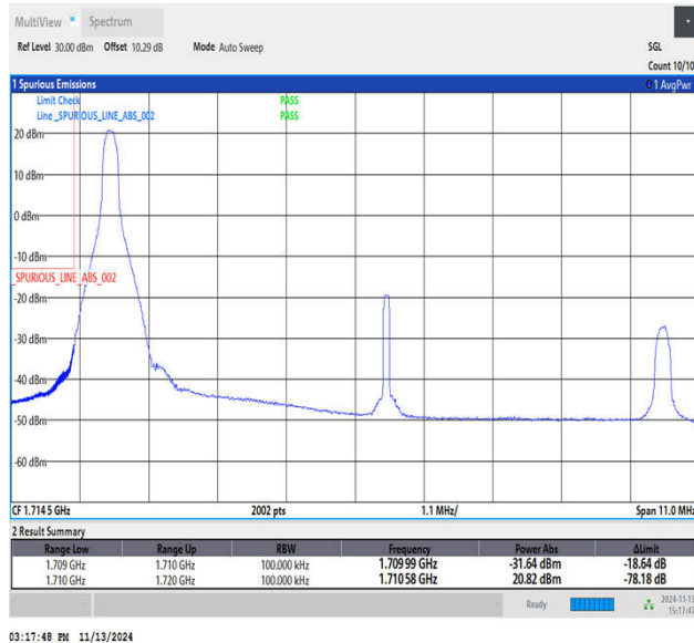
Band4_10MHz_16QAM_20000_1RB#0
