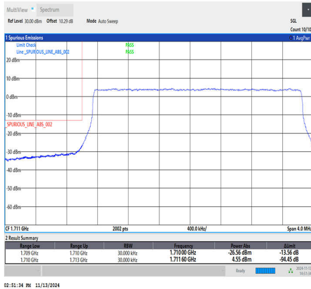
Band4_3MHz_QPSK_19965_15RB#0
