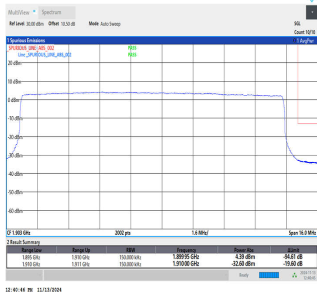
Band2_15MHz_16QAM_19125_75RB#0
