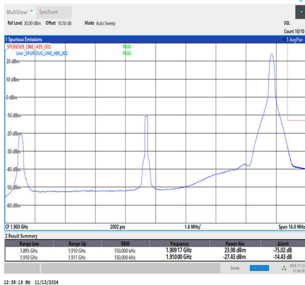
Band2_15MHz_QPSK_19125_1RB#74
