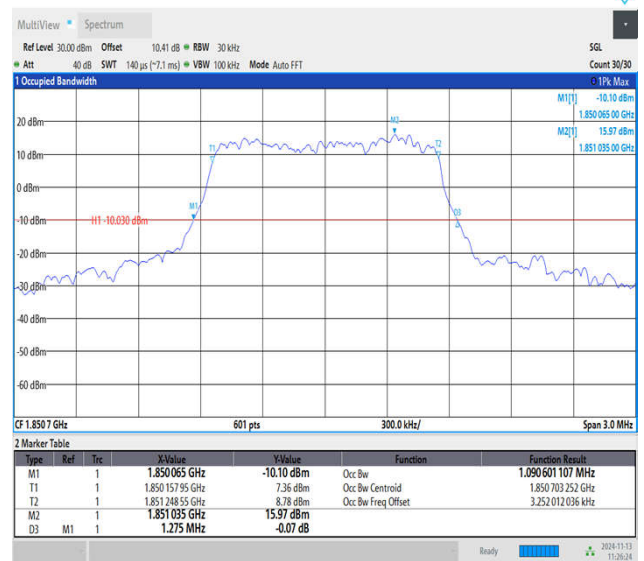
Band2-1.4MHz-16QAM-18607-6RB#0-PASS
