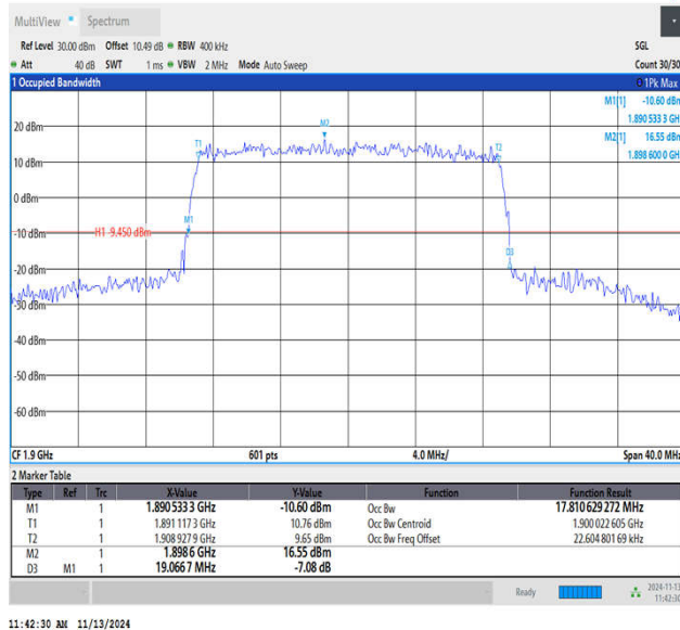
Band2-20MHz-16QAM-19100-100RB#0-PASS
