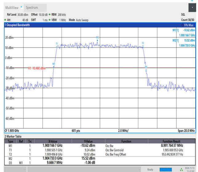
Band2-10MHz-64QAM-19150-50RB#0-PASS
