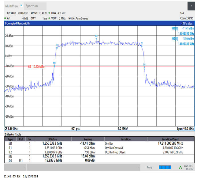
Band2-20MHz-64QAM-18700-100RB#0-PASS
