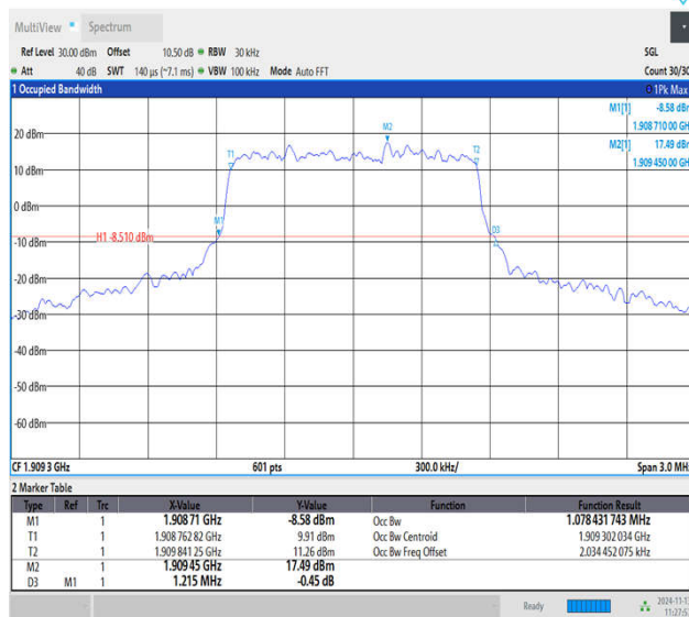
Band2-1.4MHz-QPSK-19193-6RB#0-PASS
