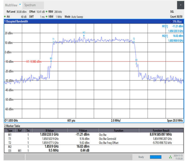
Band2-10MHz-64QAM-18650-50RB#0-PASS
