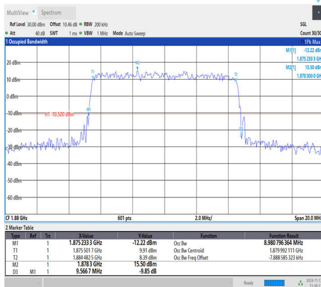
Band2-10MHz-64QAM-18900-50RB#0-PASS
