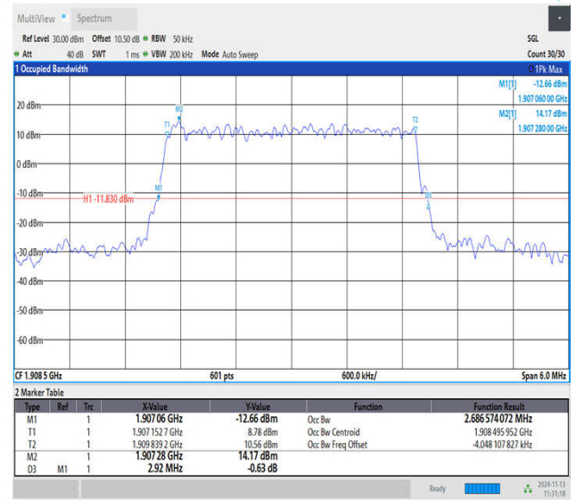
Band2-3MHz-64QAM-19185-15RB#0-PASS
