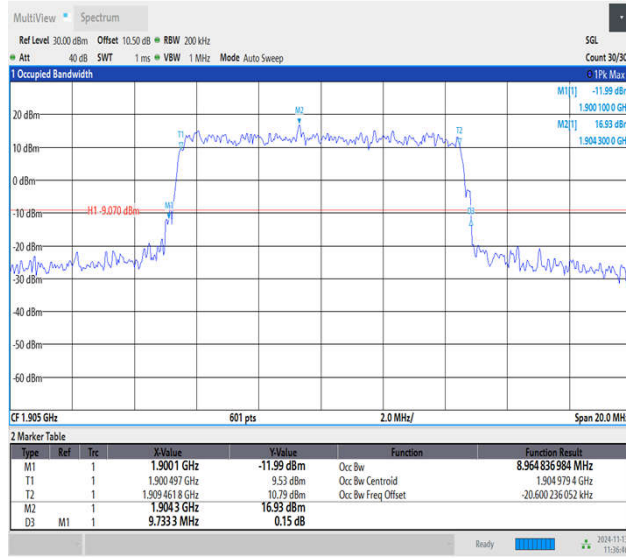
Band2-10MHz-16QAM-19150-50RB#0-PASS
