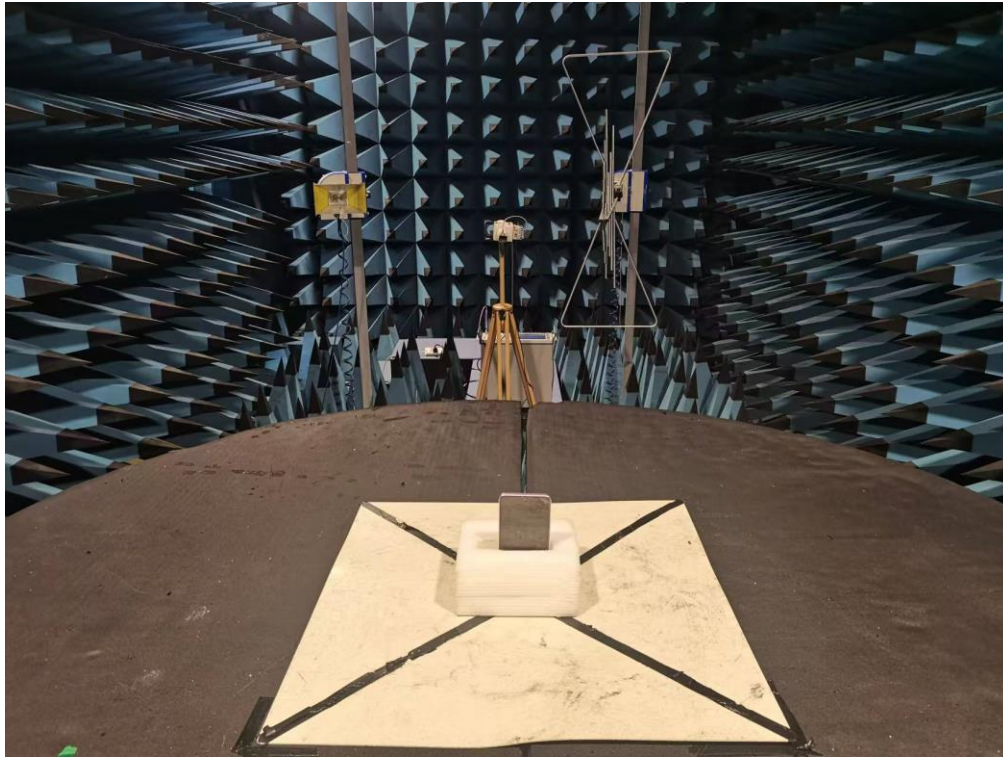
Radiated Spurious 18GHz -26.5GHz -Front
